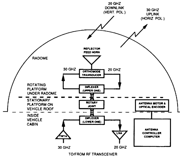
Fig. 3 Reflector Antenna Block Diagram
