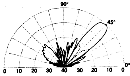
Fig. 7 Elevation Pattern, 30 GHz, Co- and X-pol.
