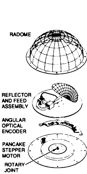
Fig. 2 Reflector Antenna Exploded View
