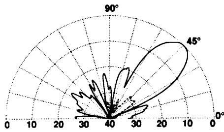
Fig. 6 Elevation Pattern, 20 GHz, Co- and X-pol.
