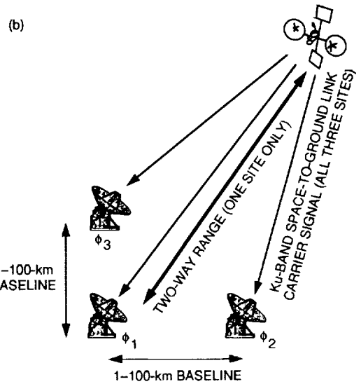
Fig. 9. Hypothetical TDRS tracking with short-baseline differential carrier phase and distributed (connected element) clock plus two-way range to one of the three sites: (a) expected accuracy and (b) schematic of ground network and data links.
