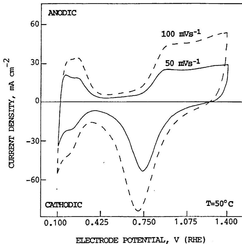
FIGURE 11. Cyclic voltammograms for an M&E assembly fabricated using Nafion-impregnated unsupported high platinum loading electrodes (5 mg Pt per \text{cm}^2 ) and Nafion 117 PEM.
