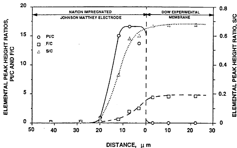
FIGURE 10. Elemental peak height ratios as a function of distance along the cross-section of an M&E assembly fabricated using unsupported high platinum loading electrodes and Dow experimental PEM.
