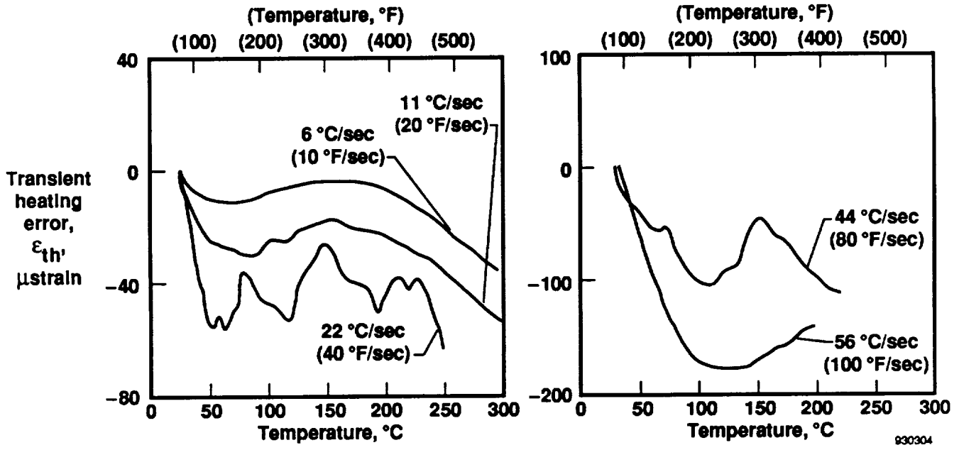
Figure 5. Transient heating error results.
