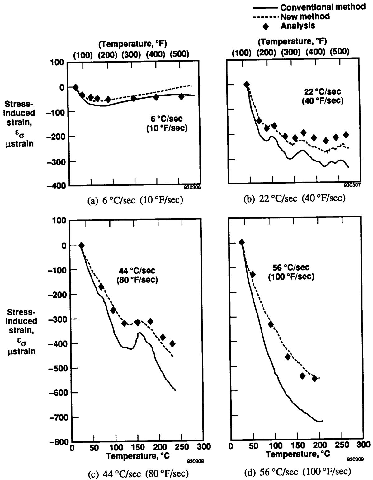
Figure 7. Stress-induced strain comparisons.
