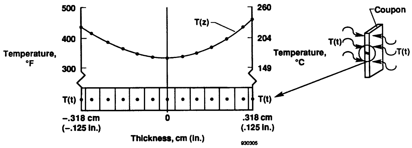
Figure 6. Finite-difference model.
