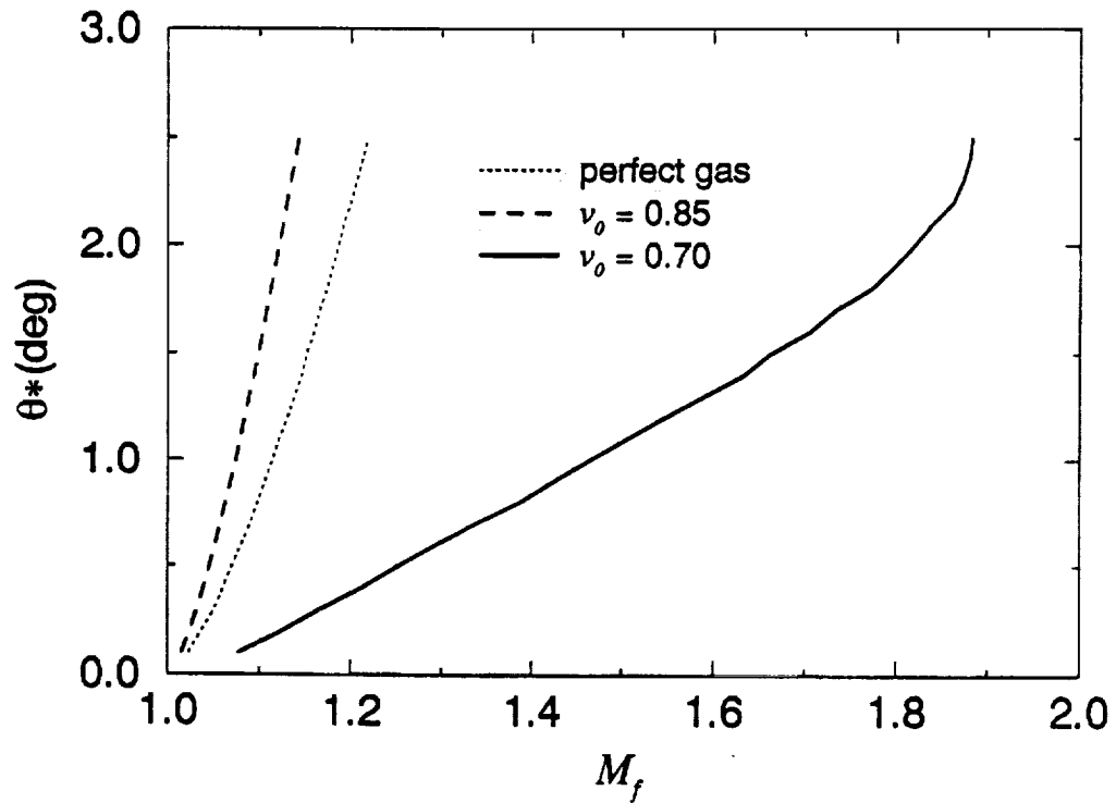
Fig. 4 (b) Initial wall turn angle \theta^* vs. M_f , nominal conditions, variable \nu_0 , two-dimensional case.
