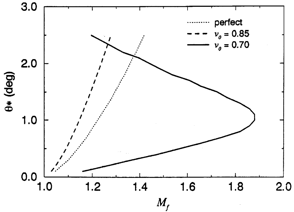
Fig. 4 (a) Initial wall turn angle \theta^* vs. M_f , nominal conditions, variable \nu_0 , axisymmetric case.
