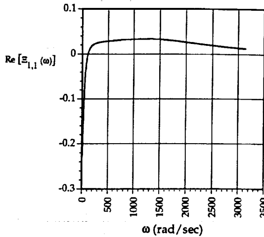
Figure 9.7: Real Part of \Xi_{1,1}(\omega) , a Component of the "Rational" Part of Forcing Spectrum for Subsonic Benchmark Parameters: A = g + iw/U_c, g = 1/(U_c\theta), U_c\theta = 17\delta^*, U_c = 88m/s, and \delta^* = 0.0039m.
