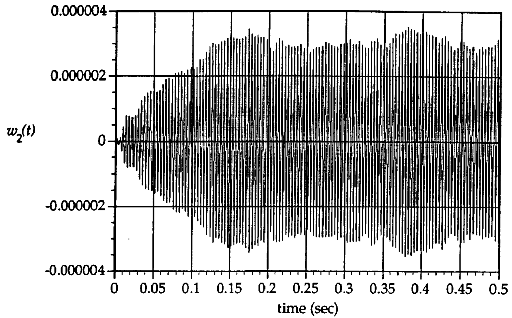
Figure 9.18a: Uncontrolled Second Mode Response of Beam to Laminar-to-Turbulent Transitional Flow
