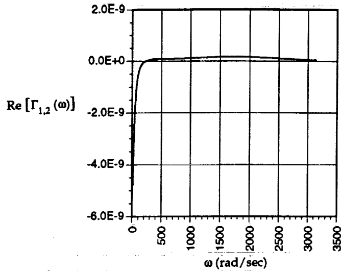
Figure 9.14a: Real Part of Spectral Density Matrix Term \Gamma_{1,2}
