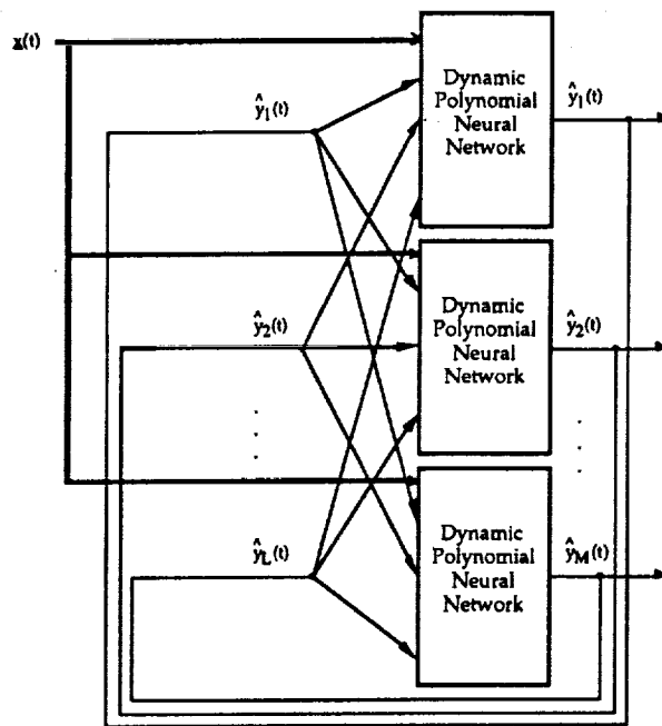
Figure 11.1: General Multi-Input, Multi-Output, Polynomial Neural Network (PNN) Mapping a Vector of L Sensor Measurements, \underline{x}(t) , Into a Vector of M Controllers, \underline{y}(t) ; Note that the Dynamic PNNs (see Fig. 9.2) may Contain Output Feedbacks and Internal Time Delays
