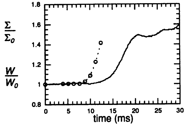
FIGURE 4. Evolution of W/W_0 (—) and \Sigma/\Sigma_0 (o), where W is the overall reaction rate, \Sigma is the total flame surface area, and the subscript 0 refers to the value at time t = 0 . The operating conditions are the same as in Fig. 3.
