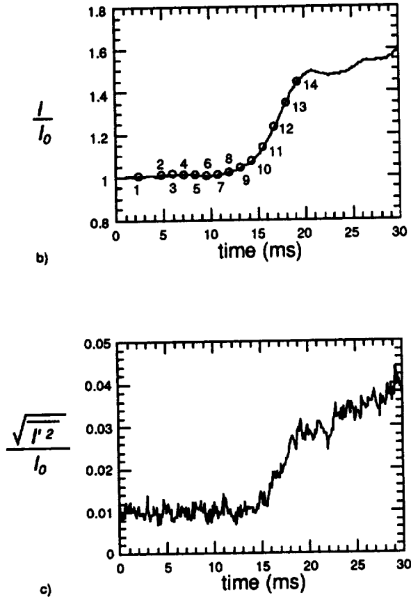
FIGURE 3. Flame-vortex interaction: fuel = C_3H_8 , \phi = 0.55 , V_0 = 0.35 m/s, \delta_l = 1 mm, S_l = 0.12 m/s, d_c = 3 mm, u_\theta = 24 m/s, Le = 1.8 ( u_\theta/S_l = 200 , d_c/\delta_l = 3 ). a) Sequence of schlieren photographs showing the evolution of the reacting flow field (see previous page) - b) evolution of the corresponding I/I_0 , where I is the mean global CH emission averaged over 50 realizations, and I_0 is the initial value of I . The numbered circles correspond to the schlieren photographs - c) evolution of \sqrt{I'^2}/I_0 , where \sqrt{I'^2} is the standard deviation of I , the global CH emission signal computed from 50 realizations, and I_0 is the initial value of I .
