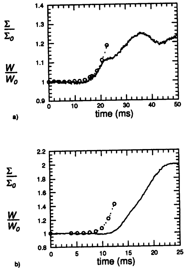
FIGURE 7. Methane-air flame. Evolution of W/W_0 (—) and \Sigma/\Sigma_0 ( \circ ), where W is the overall reaction rate, \Sigma is the total flame surface area, and the subscript 0 refers to the value at time t = 0 . The conditions are: fuel = CH_4 , \phi = 0.55 , V_0 = 0.35 \text{ m/s} , \delta_l = 2 \text{ mm} , S_l = 0.07 \text{ m/s} , d_c = 3 \text{ mm} , Le = 0.96 . a) u_\theta = 11 \text{ m/s} ( u_\theta/S_l = 160 ). b) u_\theta = 24 \text{ m/s} ( u_\theta/S_l = 340 )
