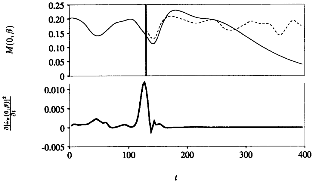
FIGURE 6. Regeneration process of unsustained flow, and modified flow. —, M(0, \beta) ; ----, same flow with \hat{v} , \hat{w}(0, y, n\beta) ( n \neq 0 ) modes multiplied by 1.5 at t = 130.0 (denoted by heavy vertical line); —, \partial|\hat{\omega}_x(0, y, \beta)|^2/\partial t , due to nonlinear terms only, integrated in y for unmodified flow.
