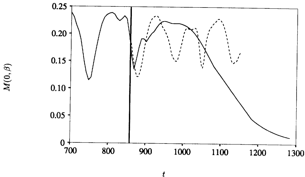
FIGURE 5. M(0, \beta) for: —, unsustained turbulent flow of Figure 3; ----, same flow with \hat{v} , \hat{w}(0, y, n\beta) ( n \neq 0 ) modes multiplied by 2.0 at t = 858.5 (denoted by heavy vertical line).
