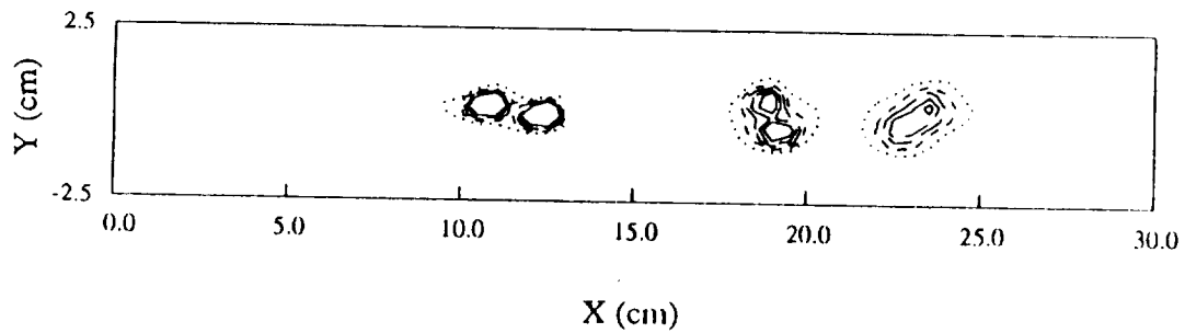
FIGURE 9. Centerplane spanwise vorticity calculated using Taylor's hypothesis at X = 13 cm, X = 20.5 cm and X = 25 cm normalized by U_1 - U_2 for \beta_2 = 22.5^\circ , 0.125 ····· ; 0.25 — — — — ; 0.375 — — — — ; 0.5 — — — — ; 0.625 — — — — ( \text{s}^{-1} ).
