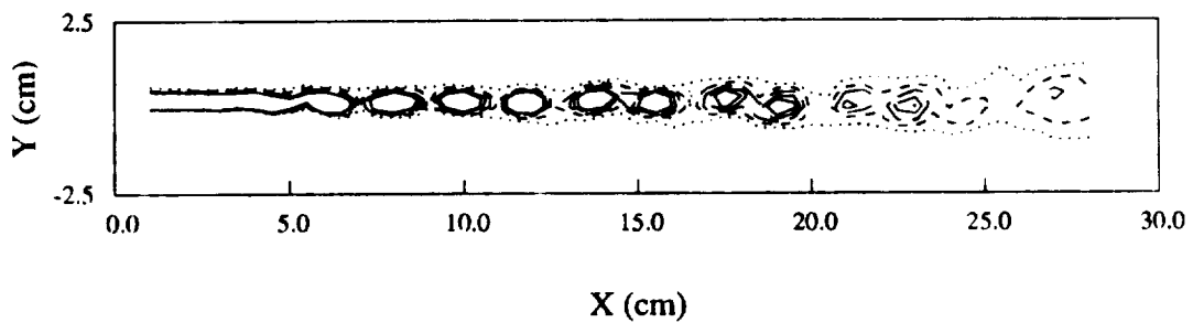
FIGURE 4. Centerplane spanwise vorticity normalized by U_1 - U_2 at T = 0 for \beta_2 = 90^\circ , 0.125 \cdots ; 0.25 ---- ; 0.375 ---- ; 0.5 ---- ; 0.625 ---- ( s^{-1} ).
