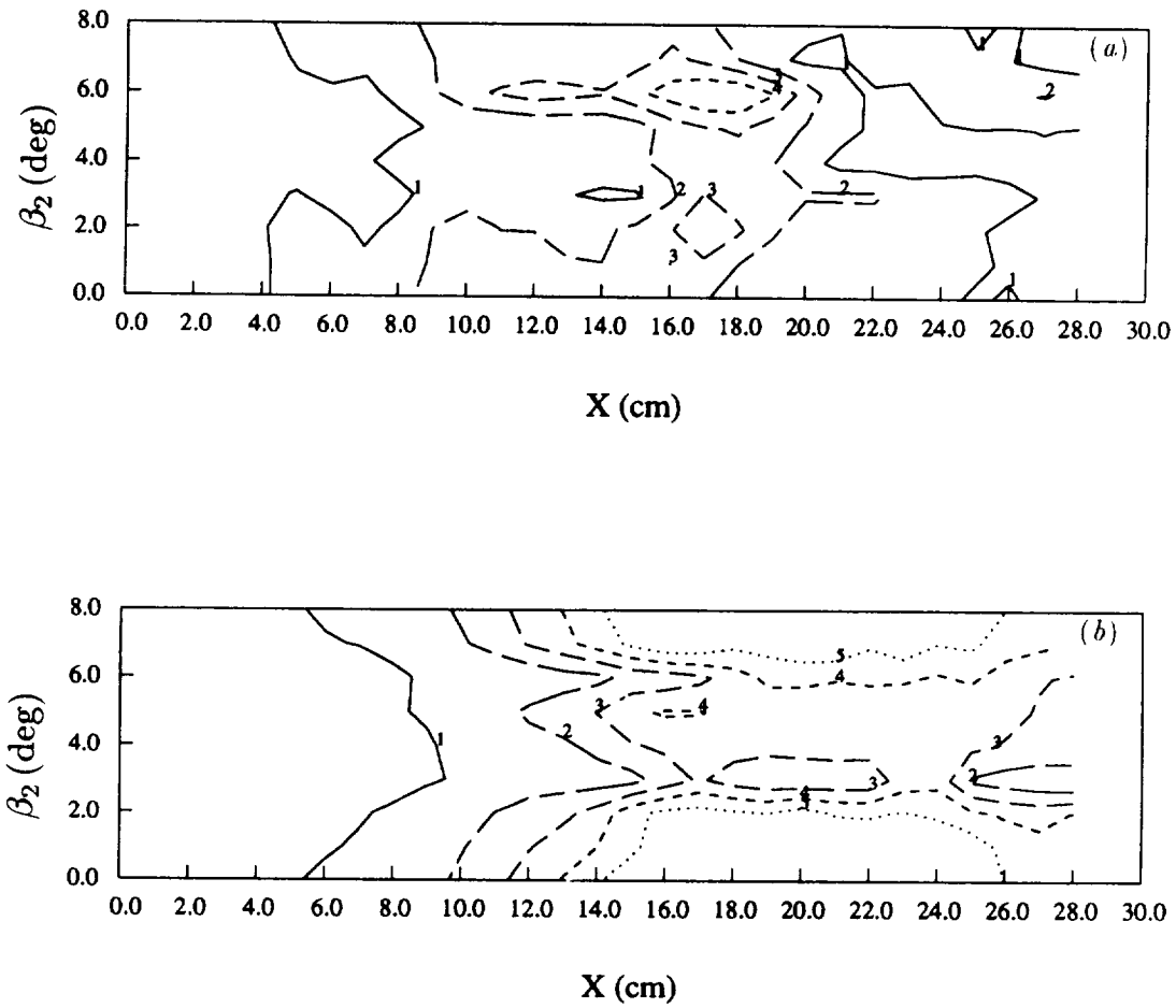
FIGURE 8. Streamwise development of subharmonic centerline spectra. (a) u , levels are 0.003 — ; 0.008 — — ; 0.013 — — — ; 0.018 — — — — ; 0.023 ·····, \text{m}^2 . (b) v , levels are 0.003 — ; 0.010 — — ; 0.017 — — — ; 0.024 — — — — ; 0.031 ·····, \text{m}^2 .
