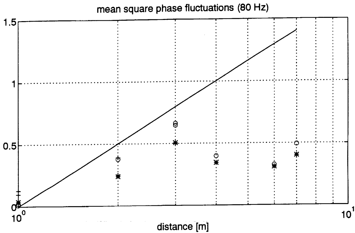
Figure 11 Mean square phase fluctuations in the transverse array.
