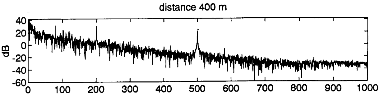
Figure 3 FFT spectra from the data in Figure 2.
