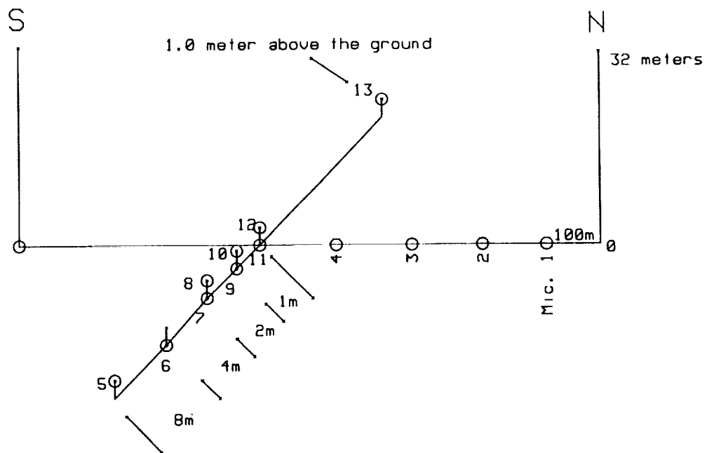
Figure 1 Short range propagation site
