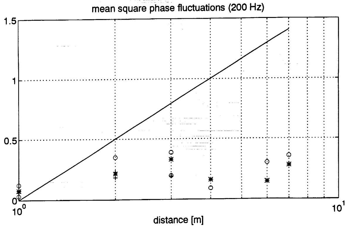
Figure 12 Mean square phase fluctuations in the transverse array.
