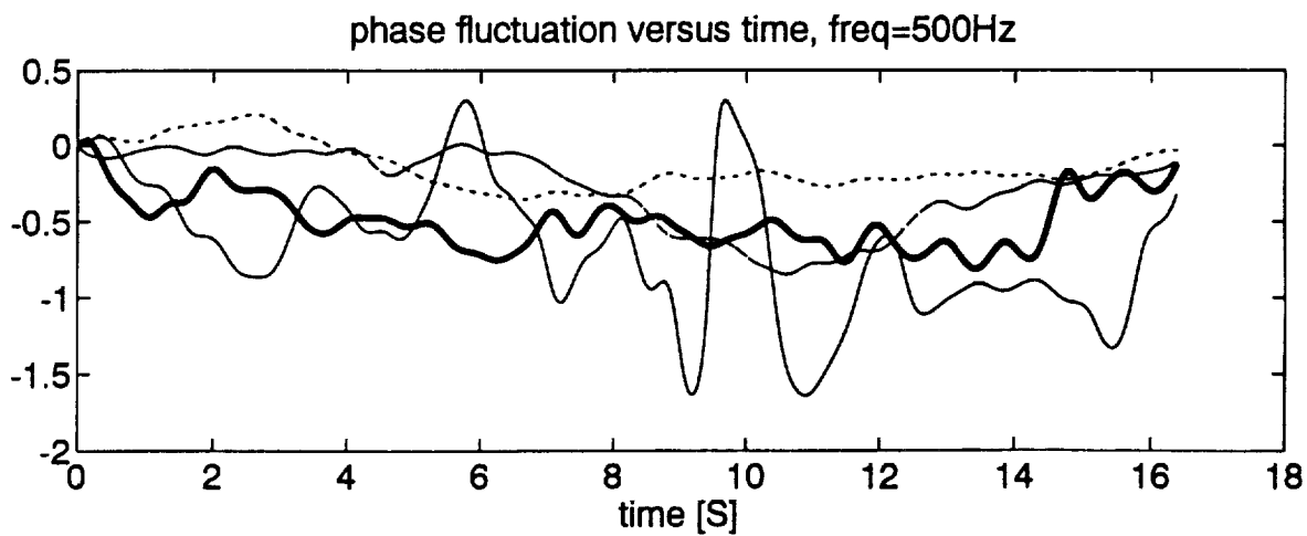
Figure 6 Phase fluctuations at distances 100 m - 400 m
