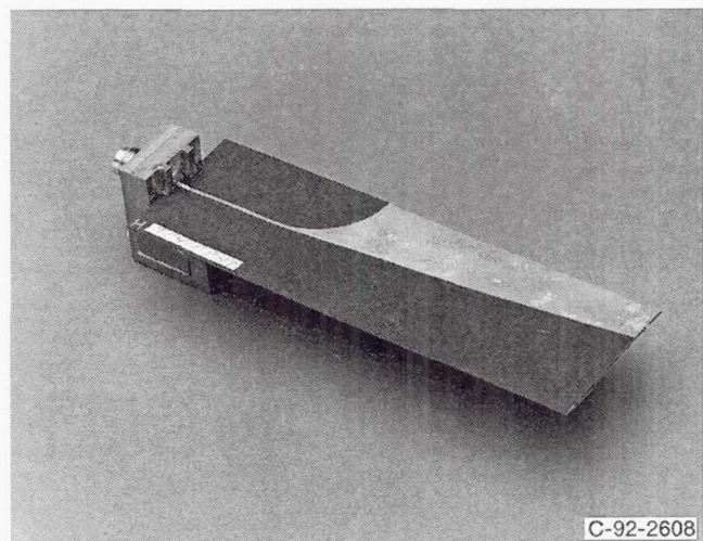
Figure 3.—Nonplanar linearly tapered slot antenna on duroid in a test fixture.
