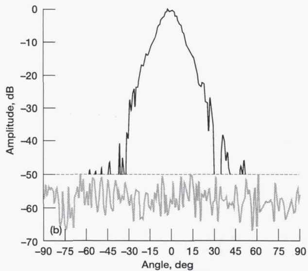
Figure 6.—Measured radiation pattern of the horn antenna showing space power combining at the second harmonic frequency of 17.9 GHz. (a) E-plane. (b) H-plane.
