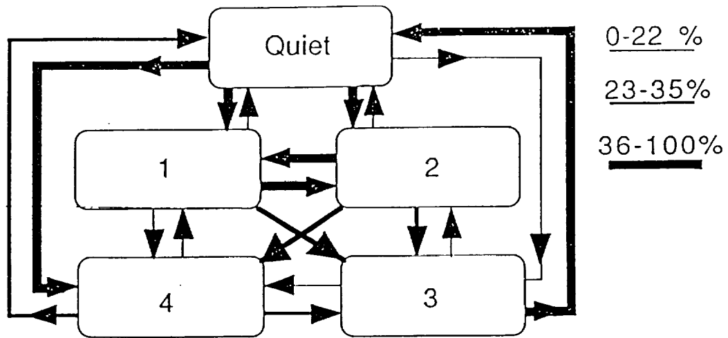
Figure 7. Emission state transition probabilities, destination normalized.
