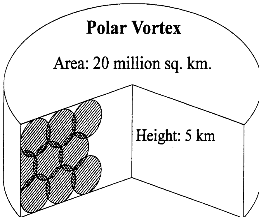
Figure 4.2-1. Depiction of the Polar Vortex geometry and the proposed delivery scheme.
