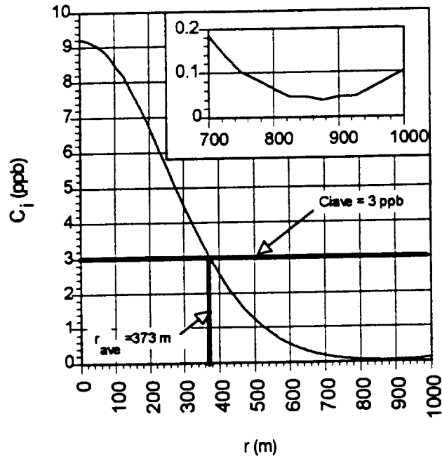
Figure 5.3 Propane concentration.
