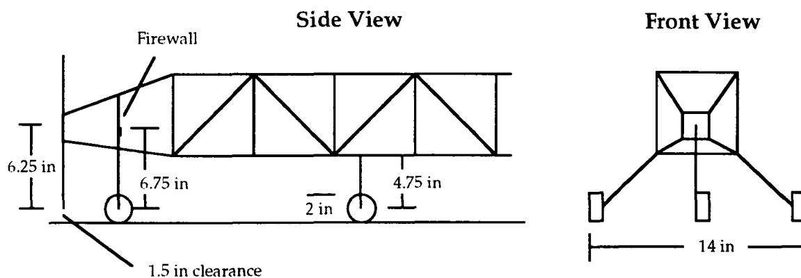
Figure H.6 - Landing Gear Schematic
