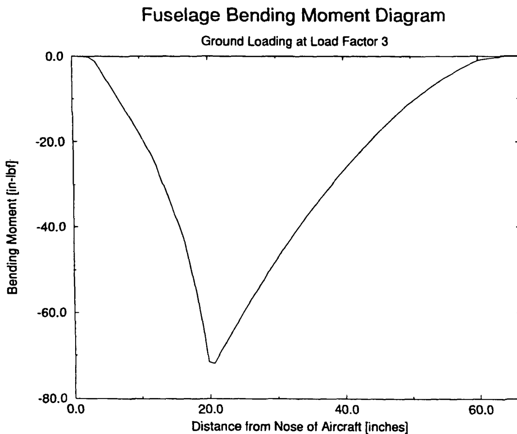
Figure H.2 - Fuselage Bending Moment Diagram (load factor=3.0, weight=4.9 lbf)
