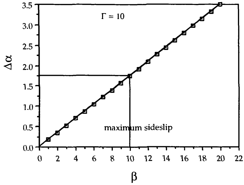
Figure F-7 - Change in angle of attack vs. sideslip due to dihedral
