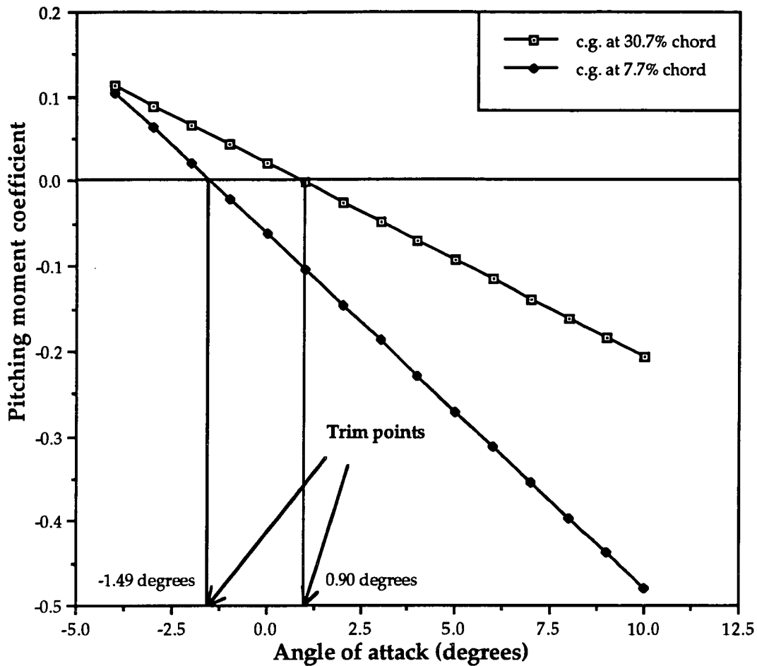
Pitching moment coefficient vs. \alpha (forward and aft c.g. positions)
