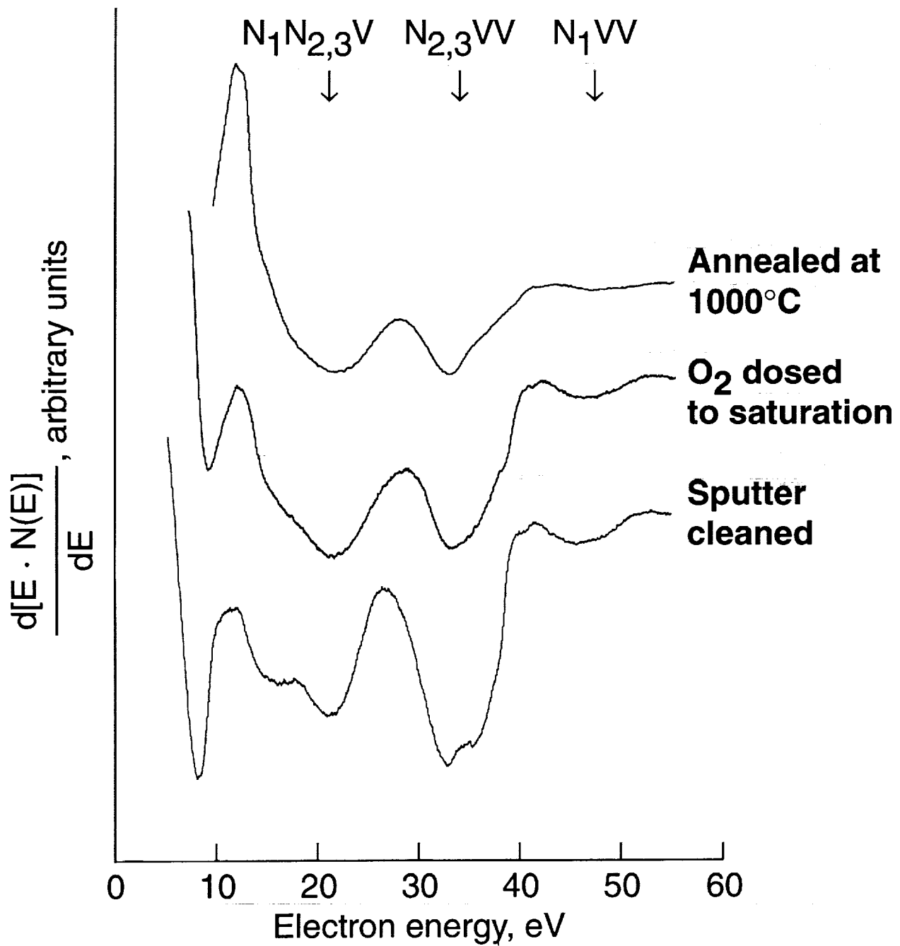
Figure 13. Low-energy AES (0 to 60 eV) molybdenum peak changes for Mo-47Re surfaces sputter cleaned, O 2 dosed to saturation, and annealed at 1000°C and then cooled to room temperature.
