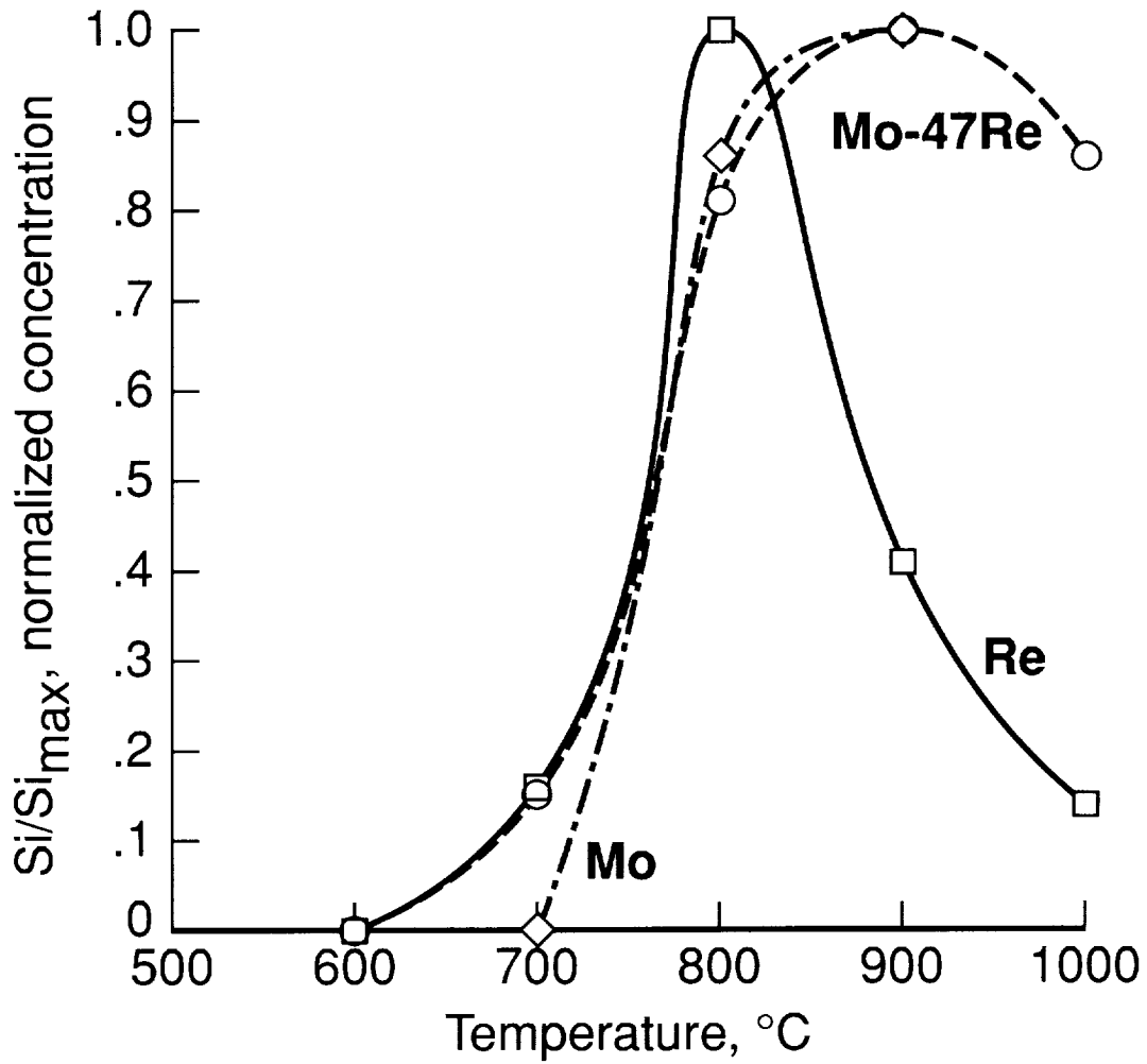
Figure 16. Segregated silicon (normalized) surface concentration (AES) as function of temperature for Mo-47Re, rhenium, and molybdenum.
