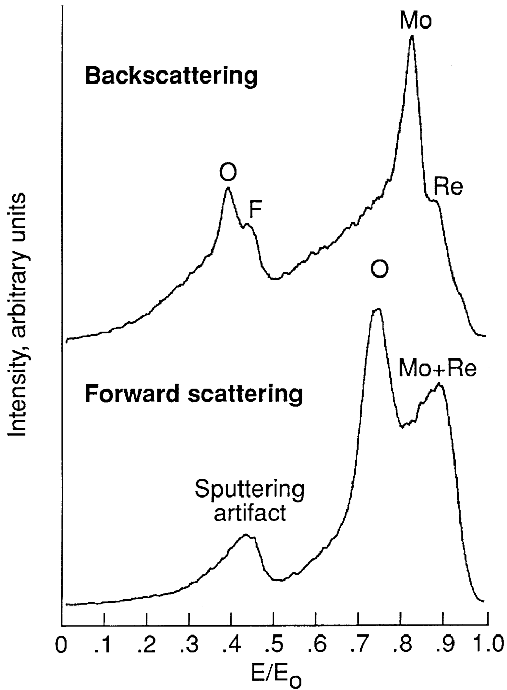
Figure 3. Forward-scattered and backscattered ISS ( ^4\text{He}^+ ) spectra taken from same as-received sample as that used for figure 2.
