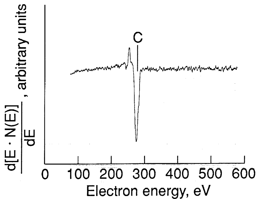
(a) AES spectrum.
