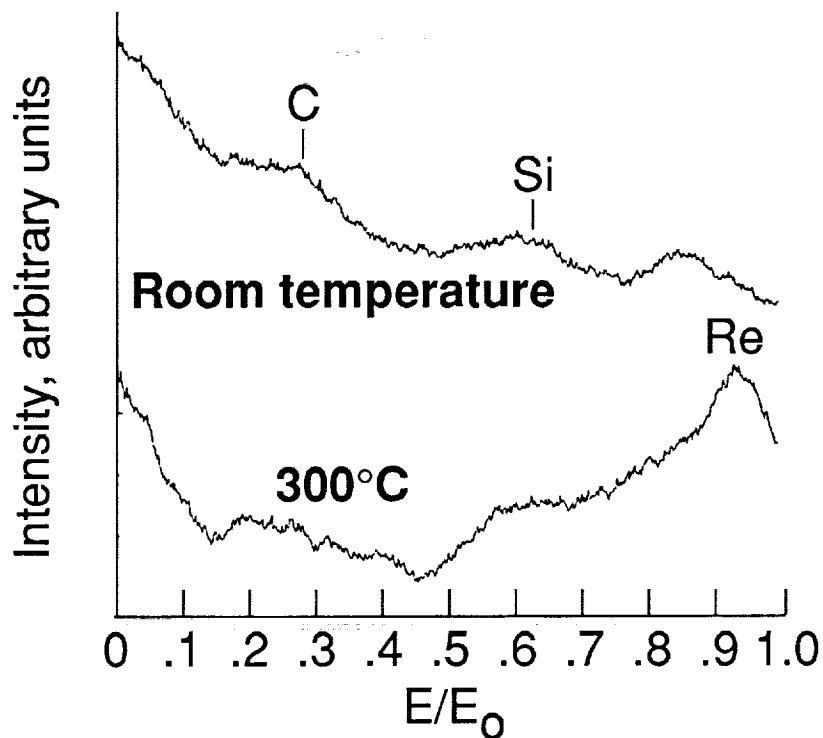
(b) Backscattered ISS ( ^4\text{He}^+ ) spectra.
