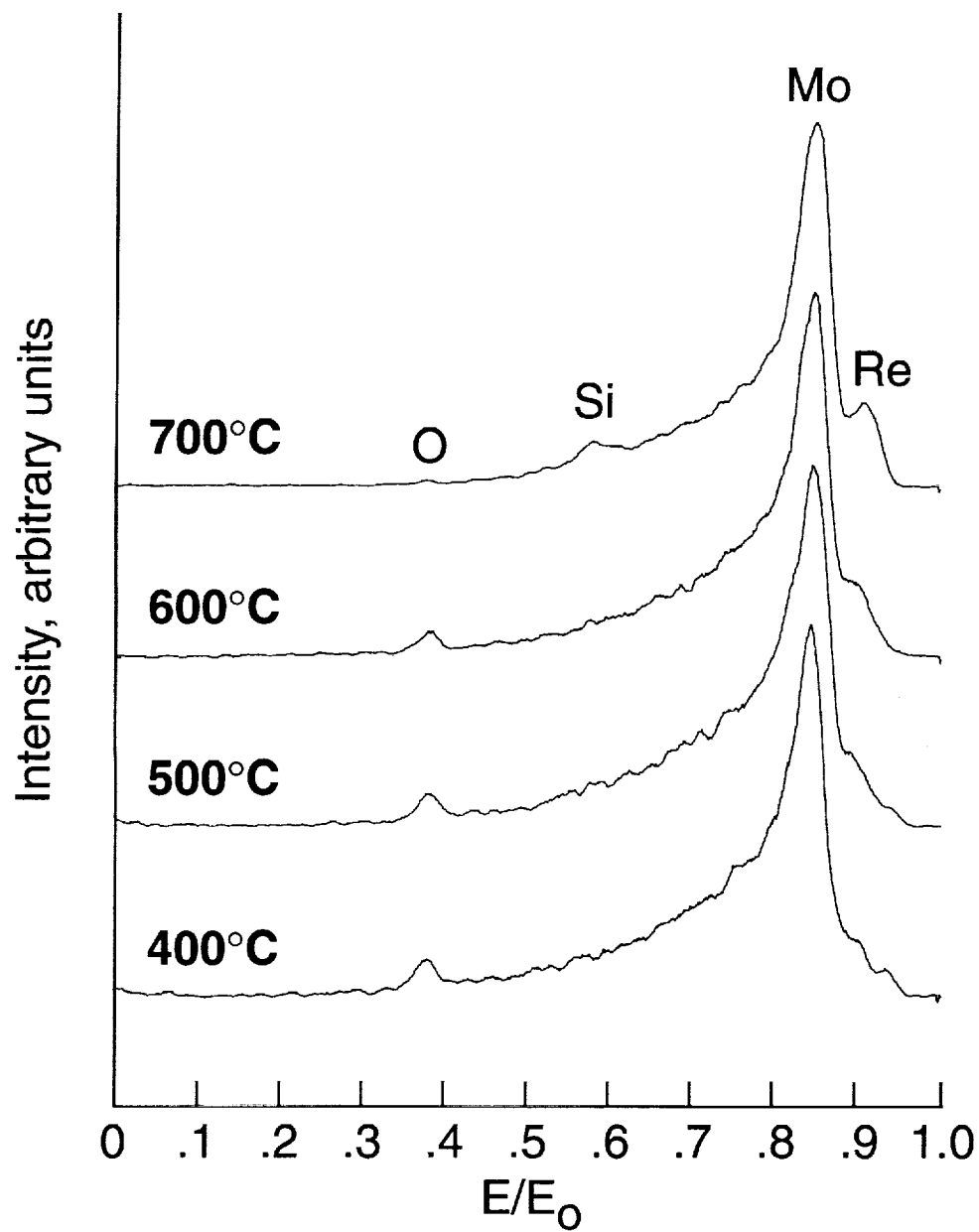
Figure 19. Backscattered ISS ( ^4\text{He}^+ ) spectra of O_2 dosed to saturation surface of silicon segregated Mo-47Re as function of temperature.
