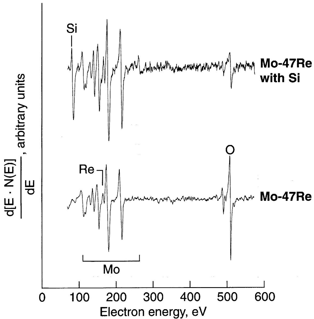
Figure 17. AES survey spectra of Mo-47Re surfaces O_2 dosed to saturation in presence or absence of silicon segregant.
