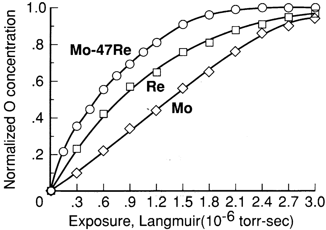
Figure 9. Oxygen (normalized) adsorption curves for Mo-47Re, rhenium, and molybdenum. Adsorption conditions are 3 \times 10^{-9} torr oxygen at 50^\circ\text{C} .
