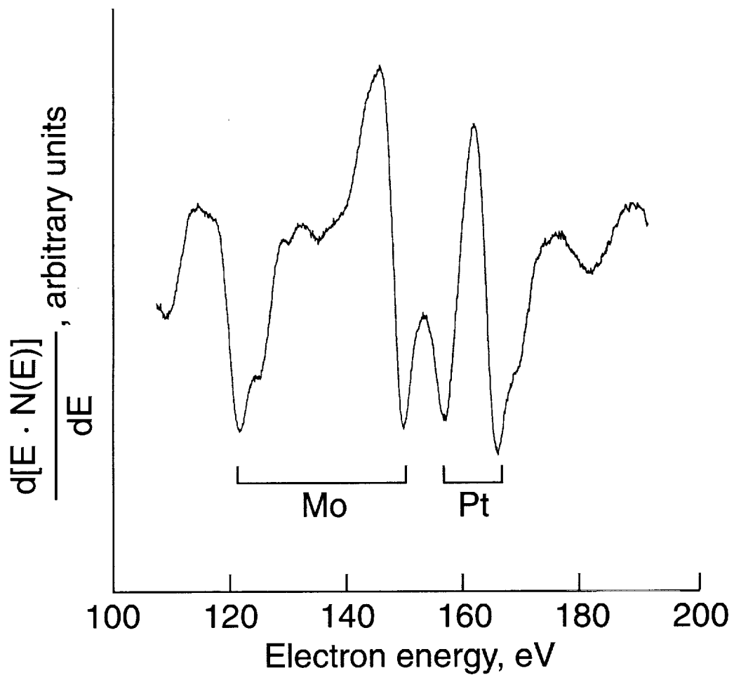
Figure 20. Mid-energy AES (100 to 200 eV) spectrum of molybdenum appearing through platinum-clad Mo-47Re after heating in vacuum to 800°C for 3 hours.
