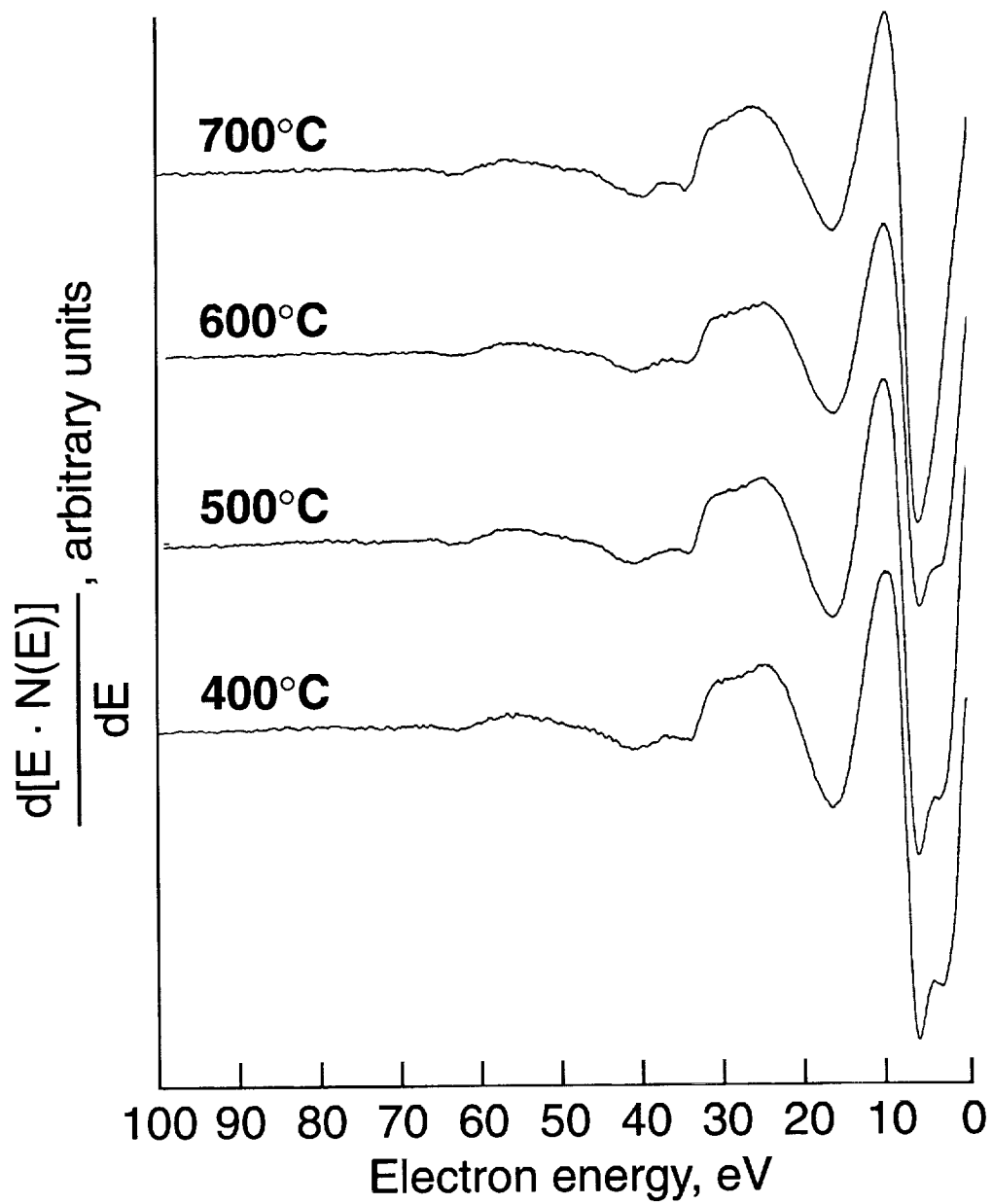
Figure 18. EELS spectra of O 2 dosed to saturation surface of silicon segregated Mo-47Re as function of temperature.
