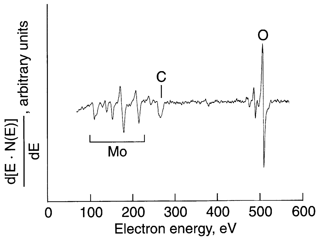
Figure 2. AES survey spectrum of polished and etched as-received Mo-47Re alloy.
