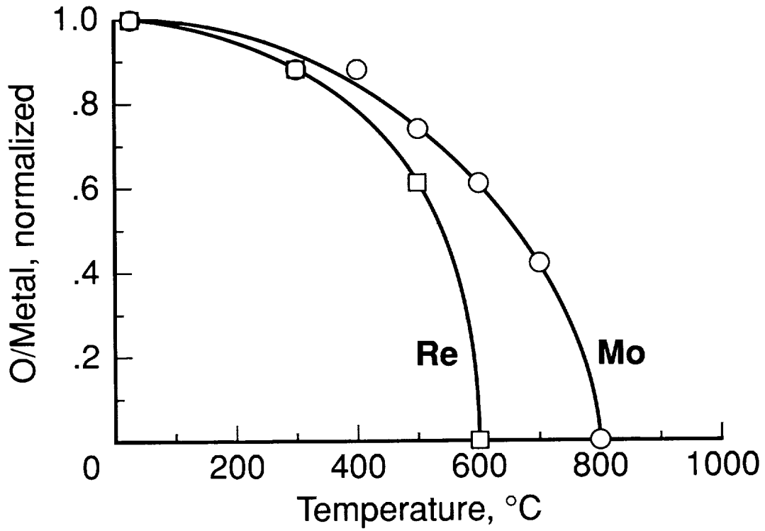
Figure 11. Oxygen (normalized) disappearance curves for rhenium and molybdenum as function of temperature.
