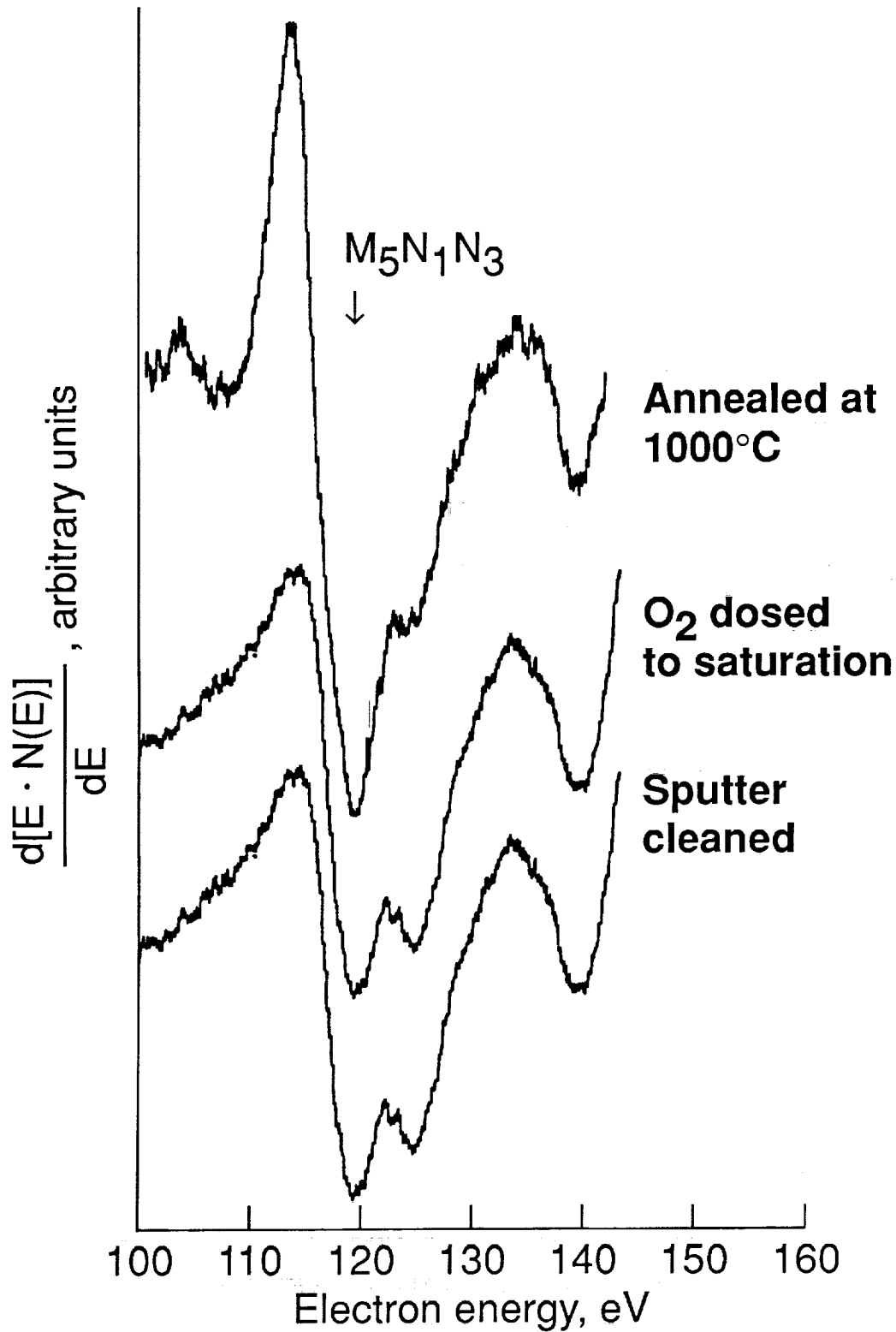
Figure 15. Mid-energy AES (100 to 150 eV) Mo peak changes for molybdenum and Mo-47Re surfaces sputter cleaned, O 2 dosed to saturation, and annealed at 1000°C and then cooled to room temperature.
