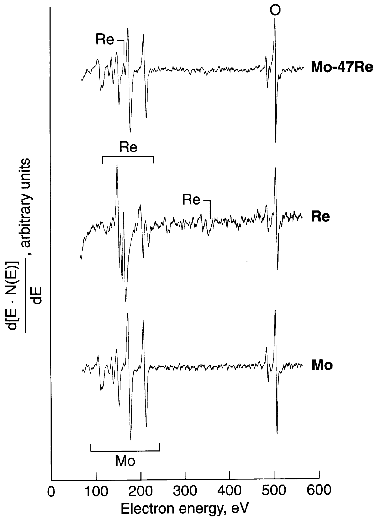
Figure 8. AES survey spectra of oxygen-saturated chemisorption on Mo-47Re, rhenium, and molybdenum.
