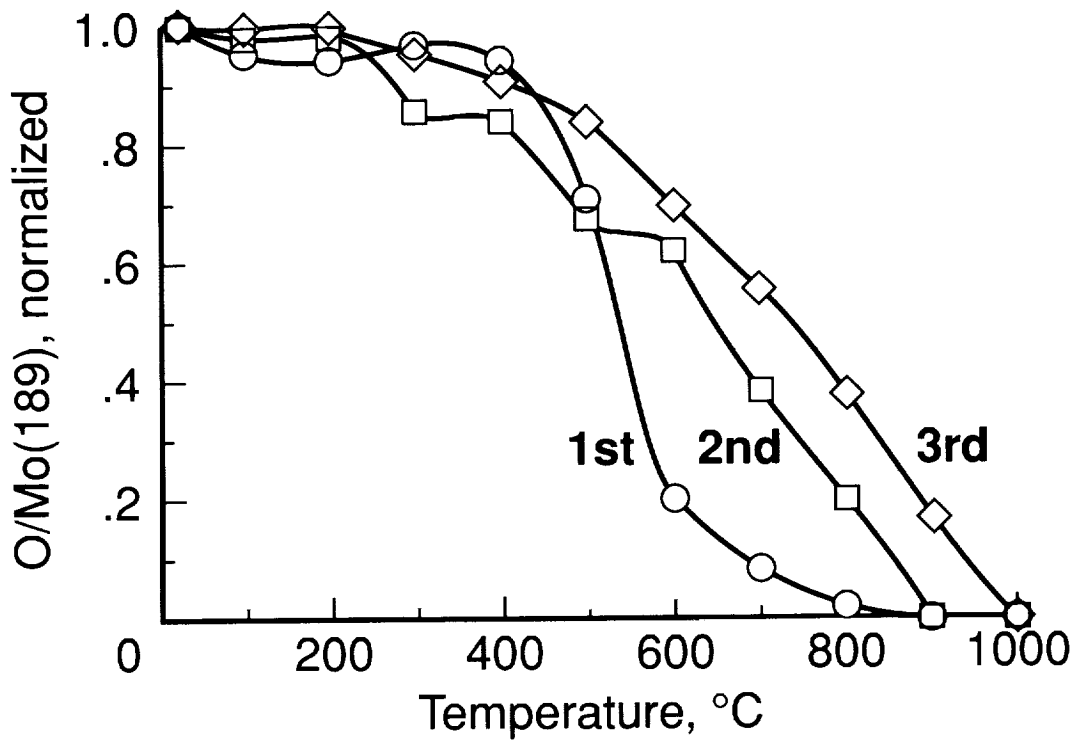
Figure 12. Successive oxygen (normalized) disappearance curves for Mo-47Re as function of temperature.
