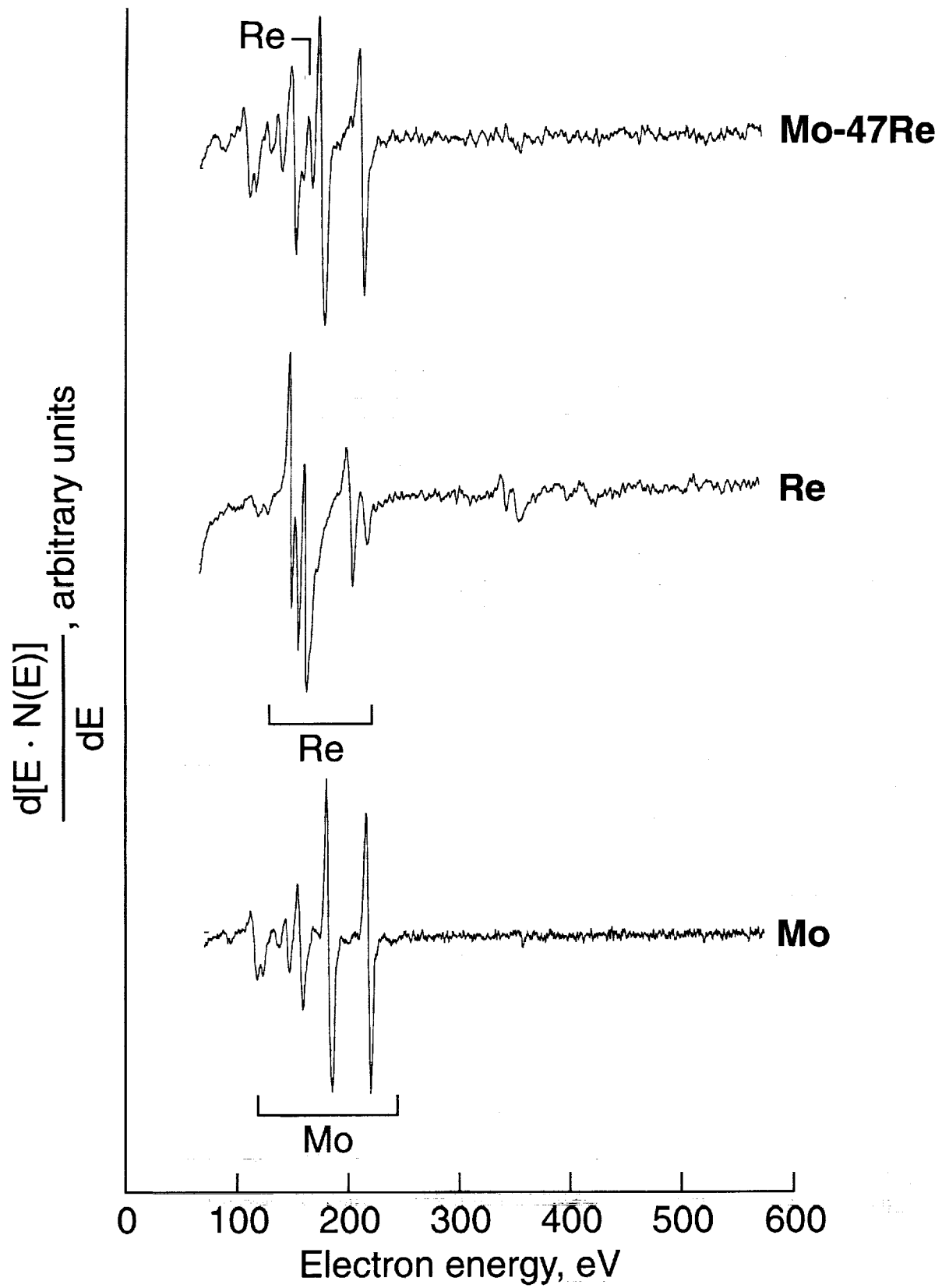
Figure 7. AES survey spectra of sputter-cleaned Mo-47Re, rhenium, and molybdenum.
