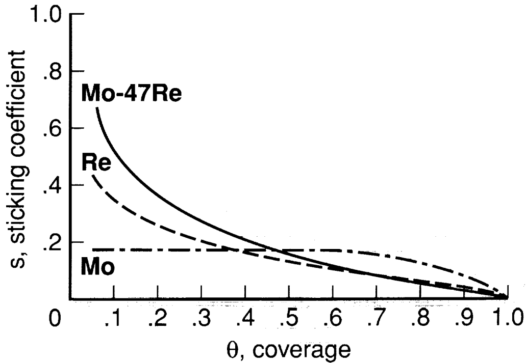
Figure 10. Sticking coefficient as function of coverage for oxygen on Mo-47Re, rhenium, and molybdenum.
