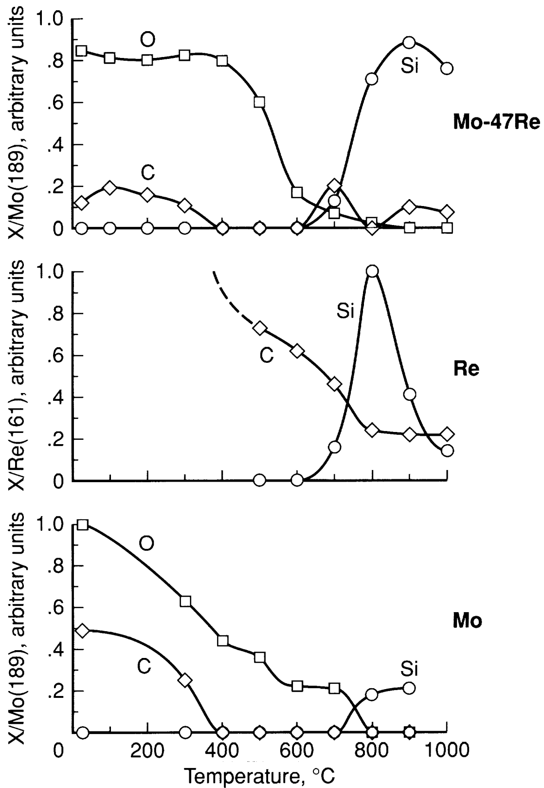
Figure 6. Surface AES compositional changes as function of temperature for as-received samples of Mo-47Re, rhenium, and molybdenum.
