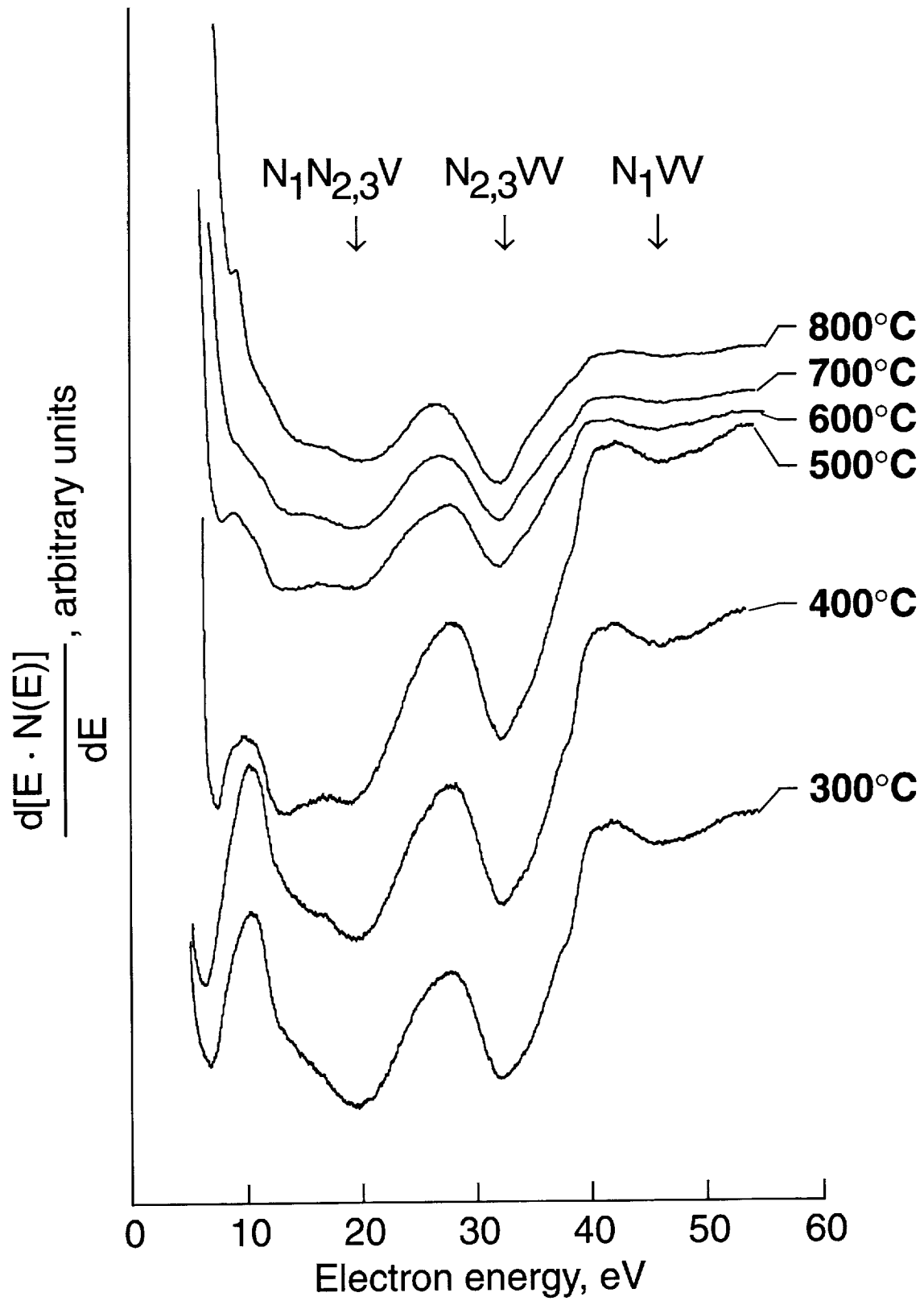
Figure 14. Low-energy AES (0 to 60 eV) Mo peak changes for Mo-47Re surface O 2 dosed to saturation and heated from 300°C to 800°C.
