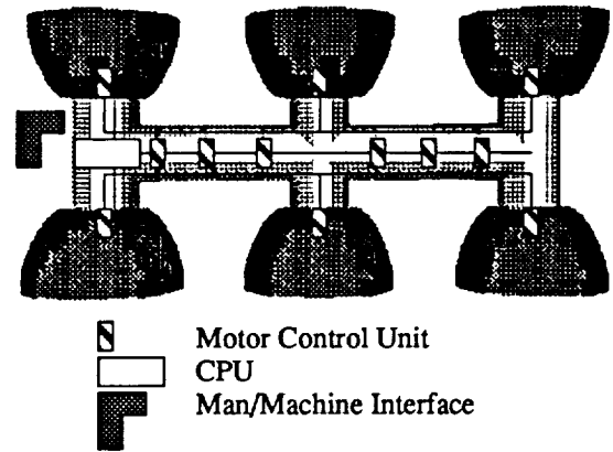
Fig. 7 Chassis controls schematic
