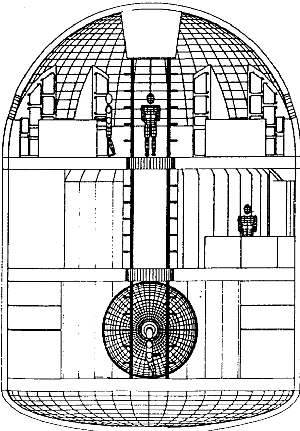
Fig. 6.6 Section C-C
