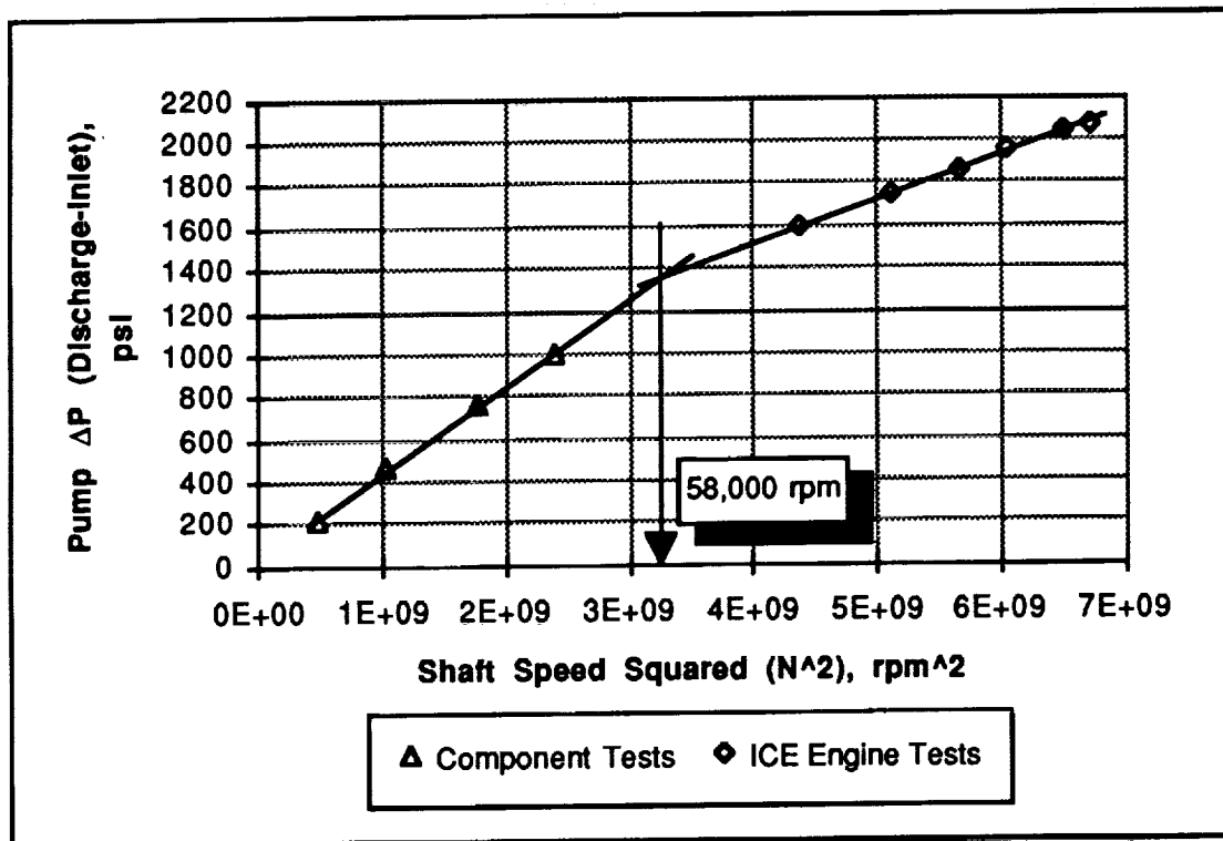
Figure 7-87 Pump Performance Shift above 58,000 RPM
