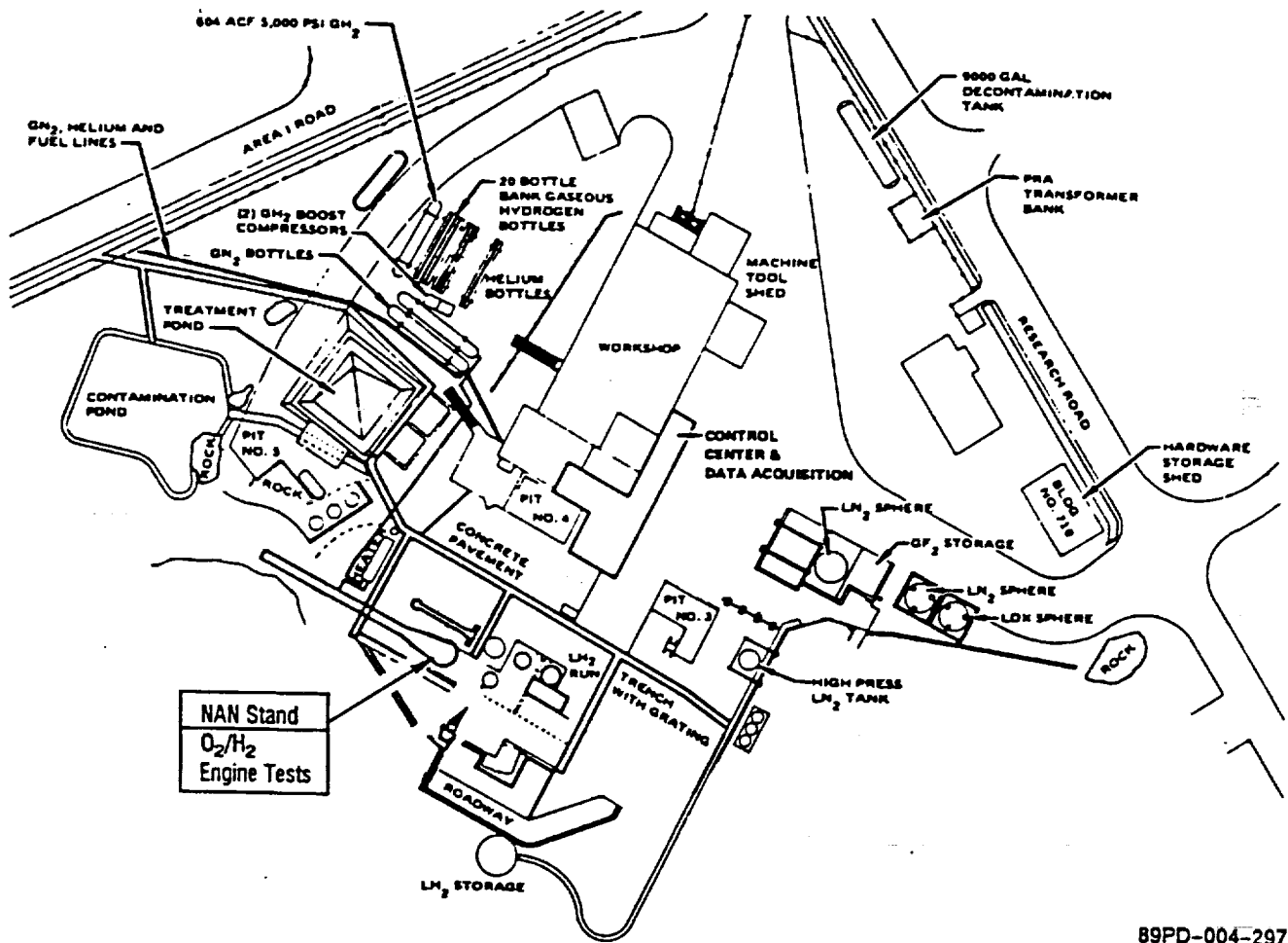
Figure 7-14 APTF OVERVIEW
