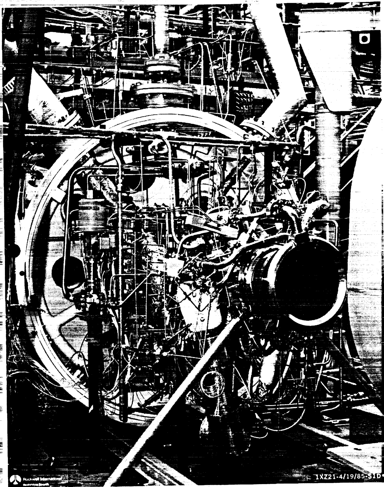
Figure 7-22 RS-44 ENGINE INSTALLATION - NAN STAND (FUEL PUMP SIDE)
