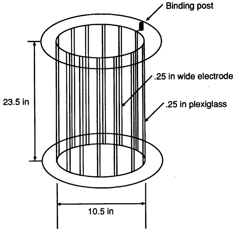
Figure 1: Tank used for data collection.
