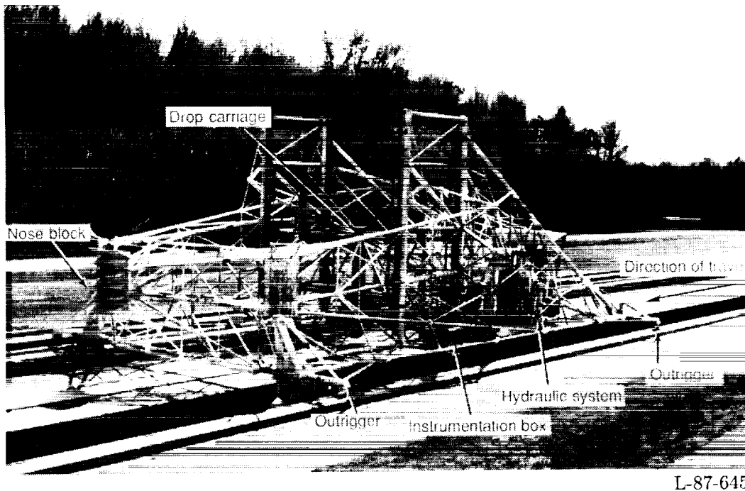
Figure 2. High-speed carriage.
