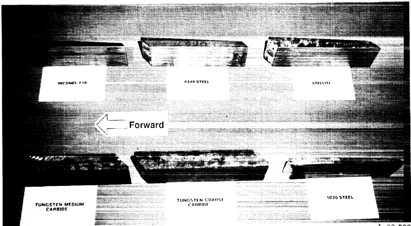
Figure 10. Skid specimens after testing.
