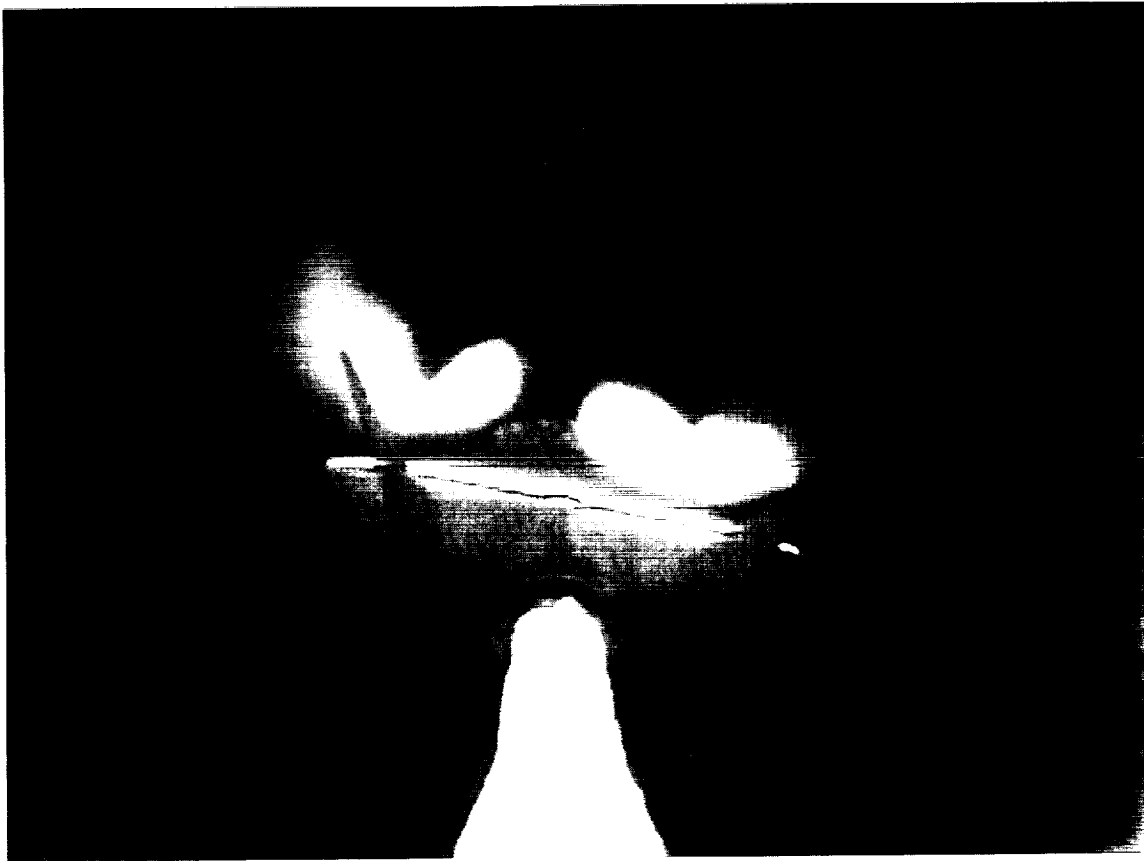
(g) Wing and LEX vortex flows upstream of tails at \beta = 5^\circ .
