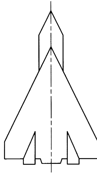
(b) 65° cropped delta wing-LEX.
