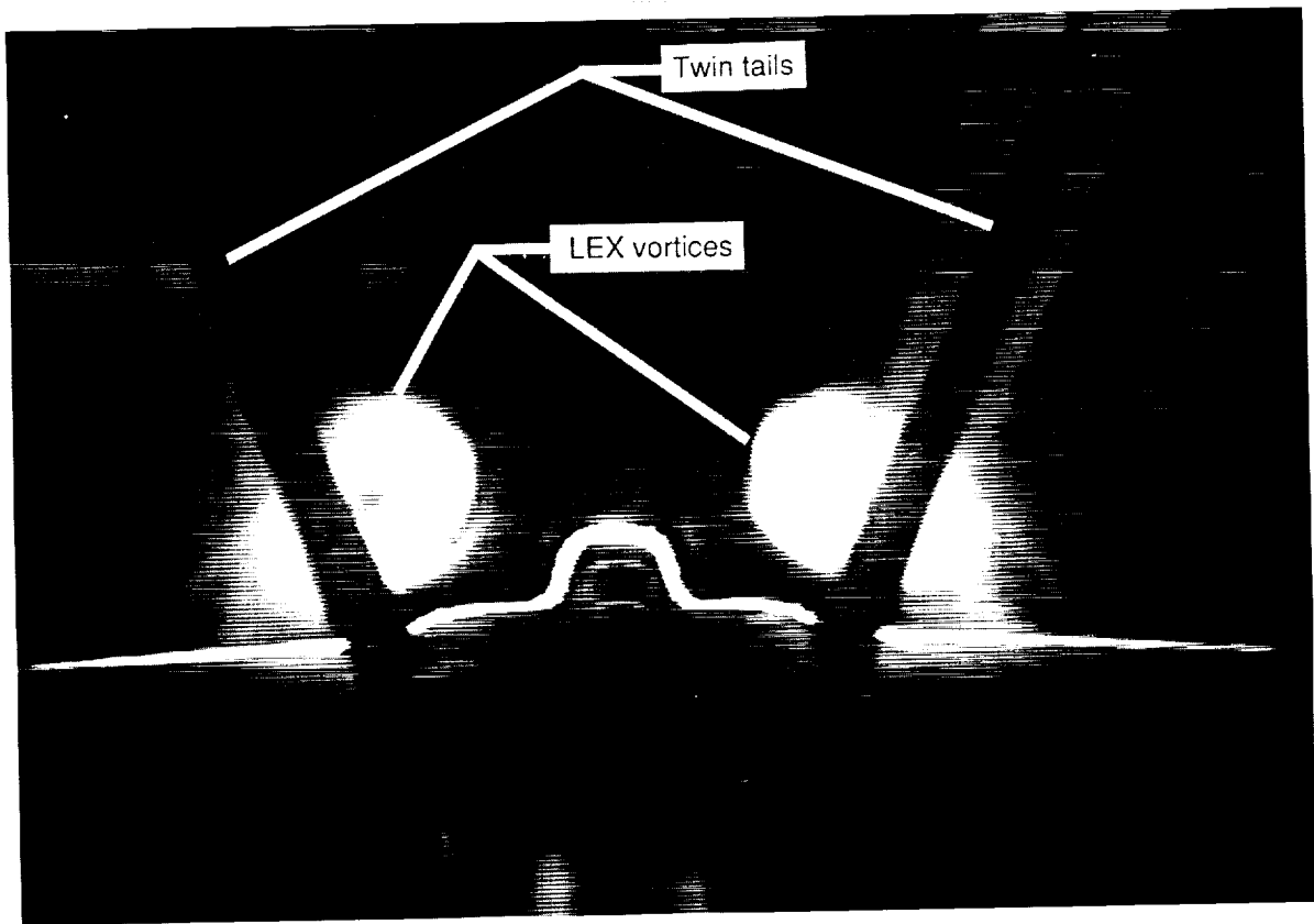
(a) M_\infty = 0.60 ; \alpha = 20^\circ .
