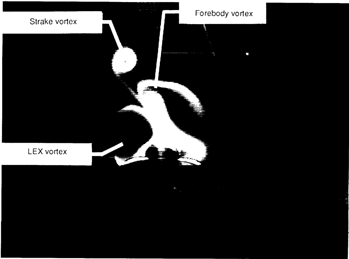
(b) M_\infty = 0.80 ; \alpha = 40^\circ .
