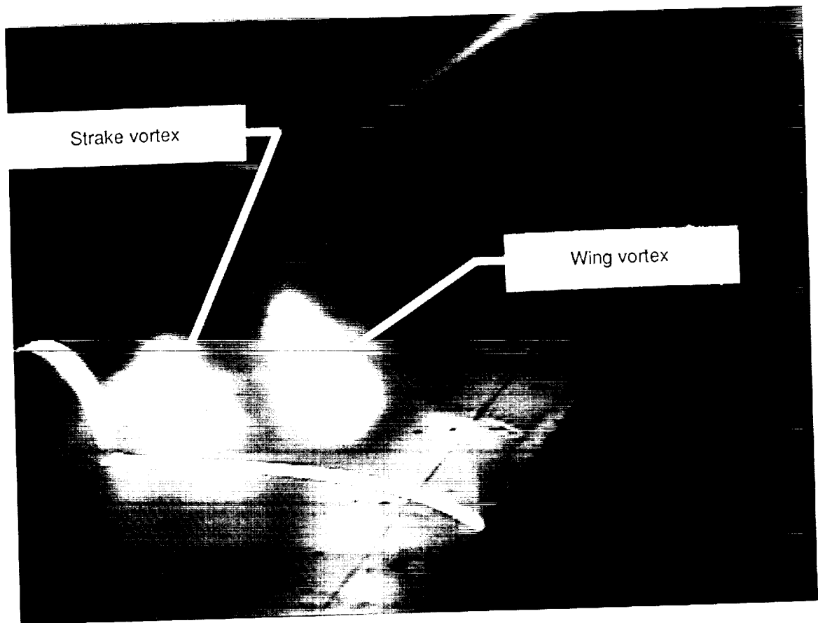
(b) Close-up view of strake and wing vortices.
