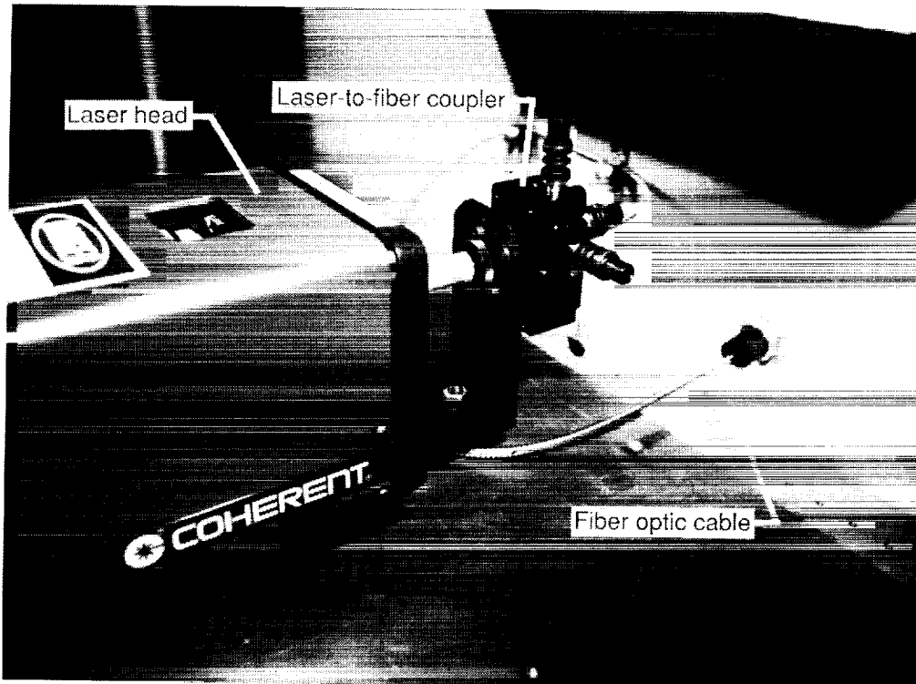
(a) Laser-to-fiber coupler.
