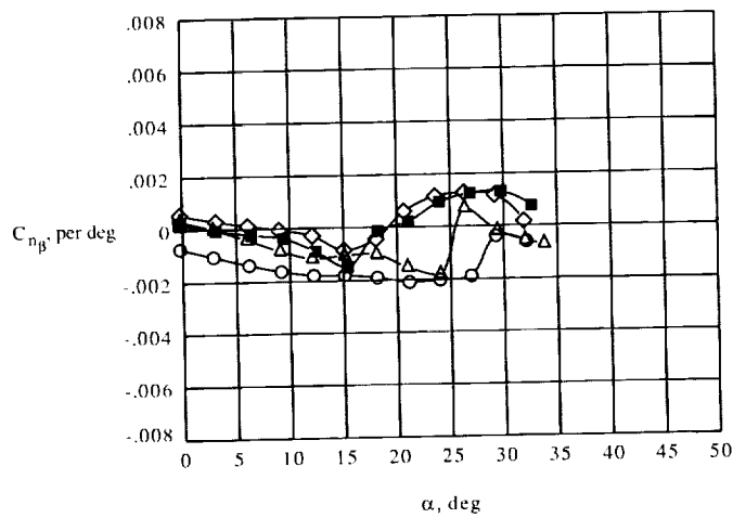
(k) Lateral-directional stability derivatives at M_\infty = 0.50 .
