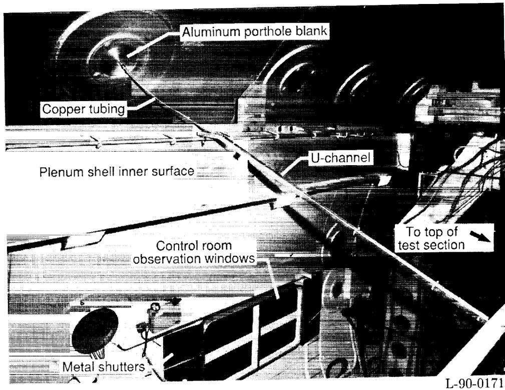
(a) Fiber optic cable penetration into plenum.
