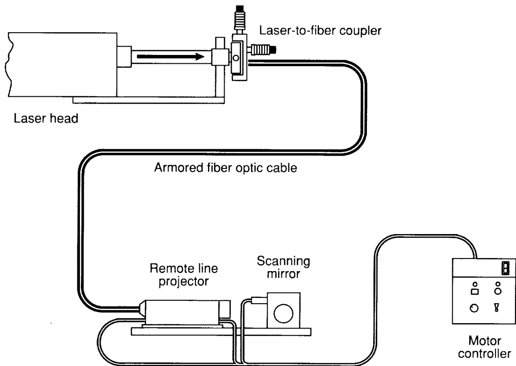
Figure 14. Sketch of fiber-optic-based beam delivery system.
