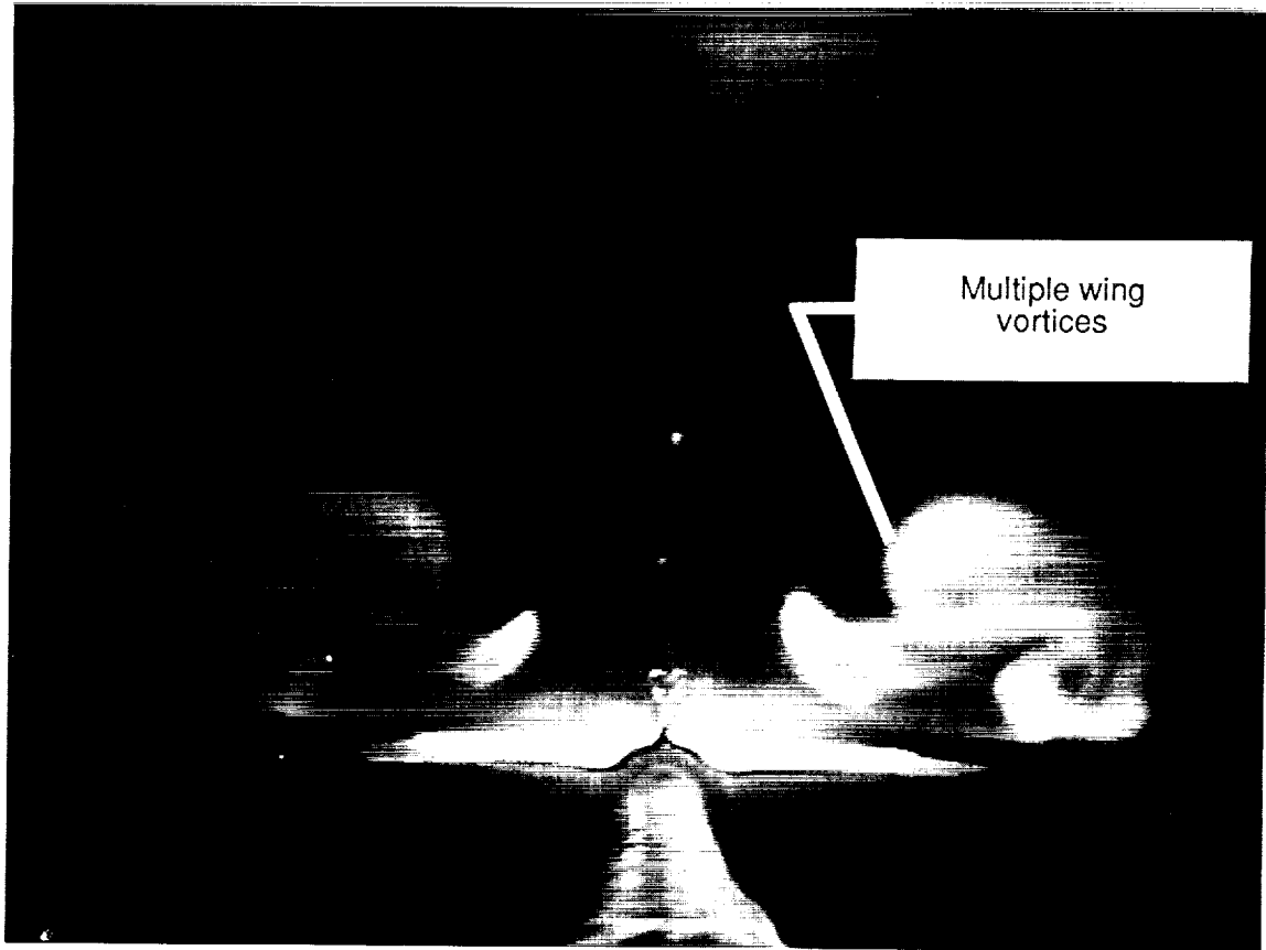
(a) Multiple vortices from wing; M_\infty = 0.85 ; \alpha = 18^\circ ; \beta = 0^\circ .
