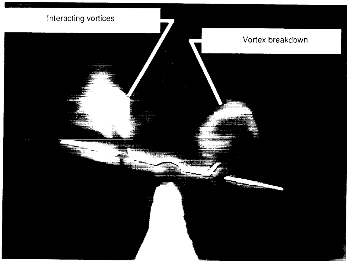
(h) Wing and LEX vortex flows at tails and \beta = 5^\circ .
