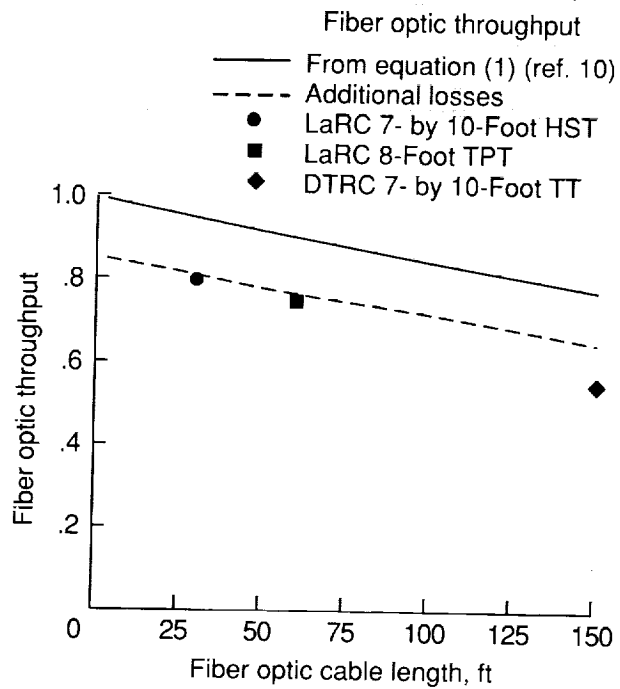
(b) Effect on fiber optic throughput.
