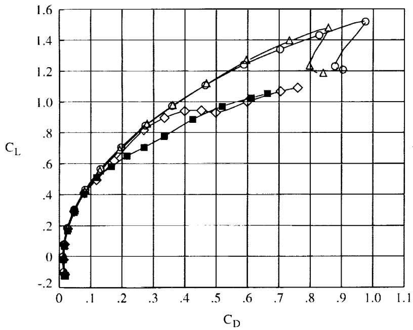
(j) Longitudinal characteristics at M_\infty = 0.50 .
