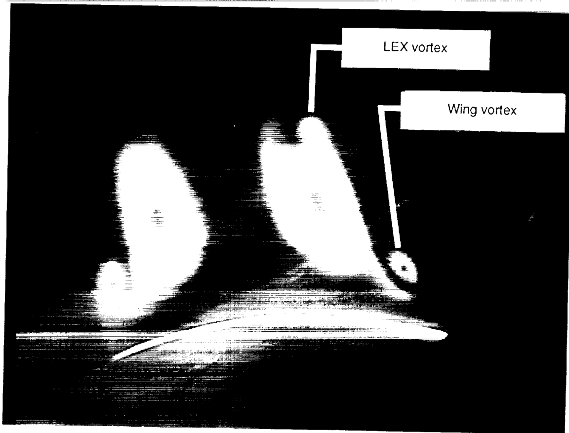
(b) Close-up view of wing and LEX vortex flows.
