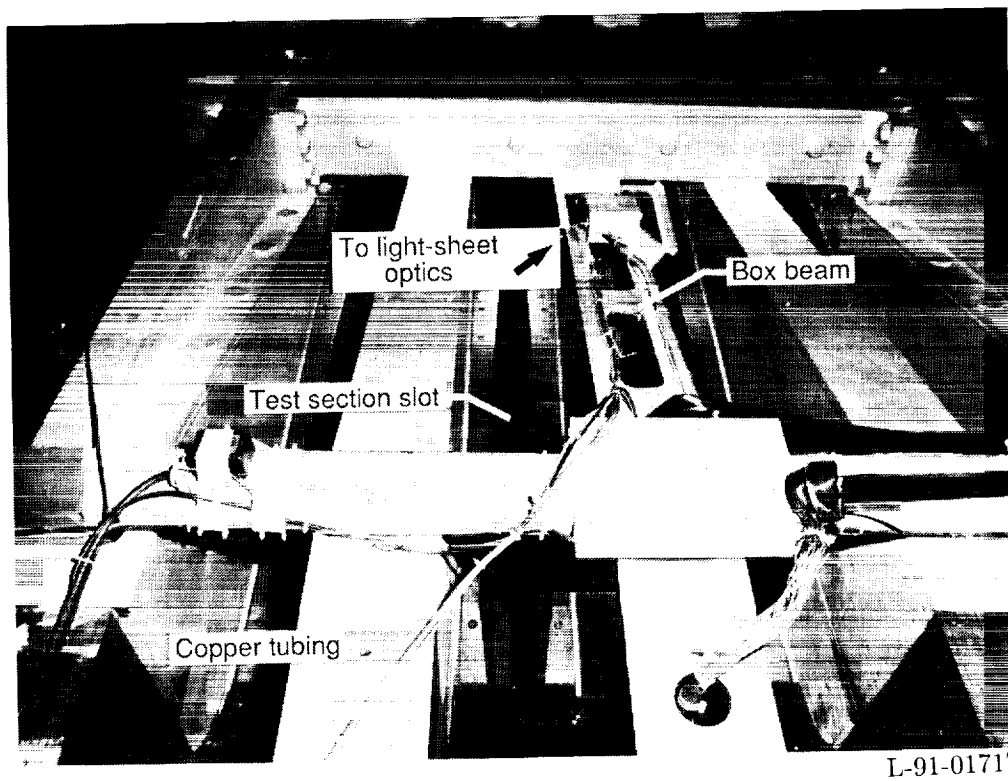
(b) Fiber optic cable routing to light-sheet optics.
