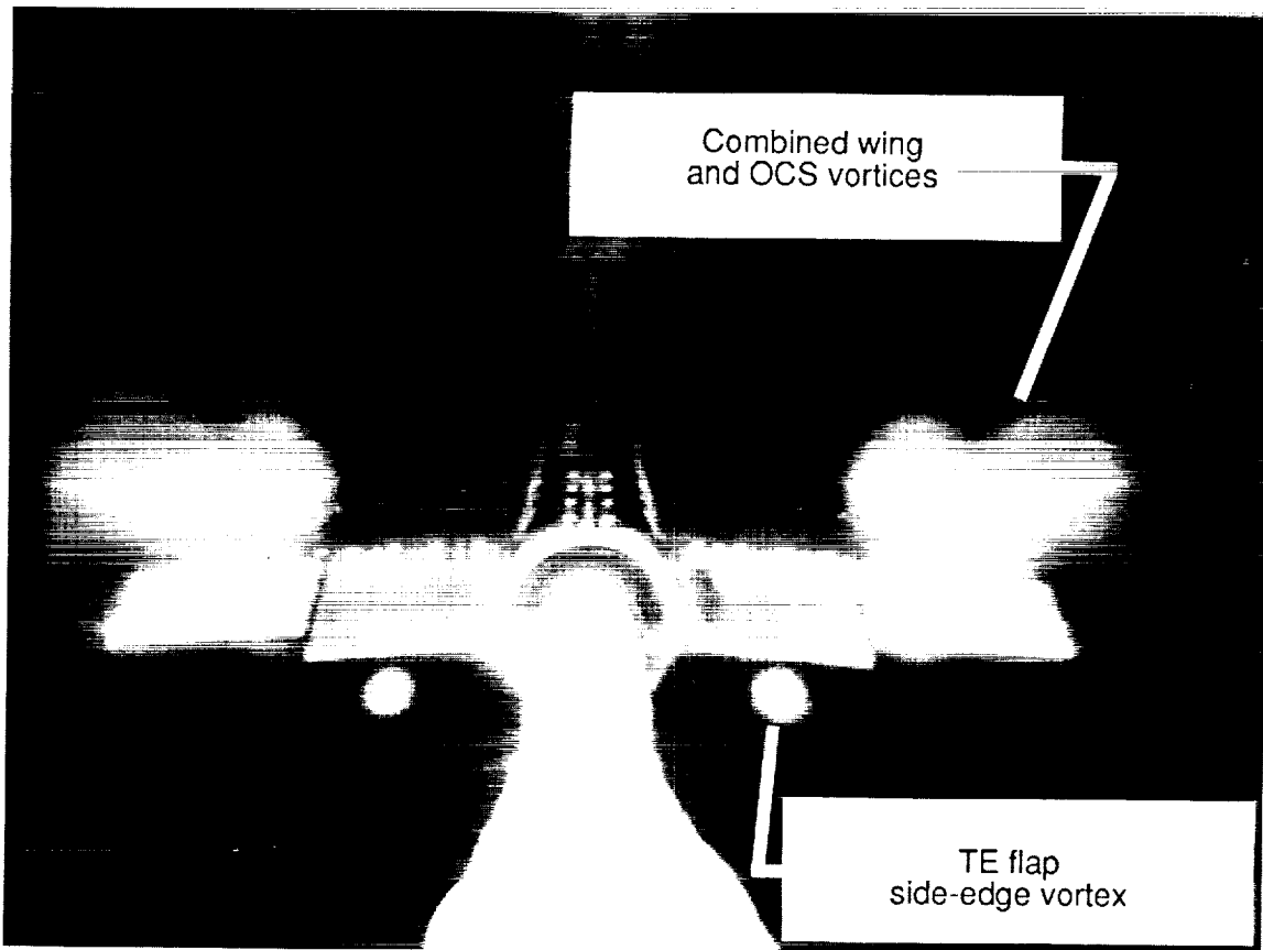
(a) M_\infty = 0.50 ; \alpha = 20^\circ (Langley 7- by 10-Foot High-Speed Tunnel).
