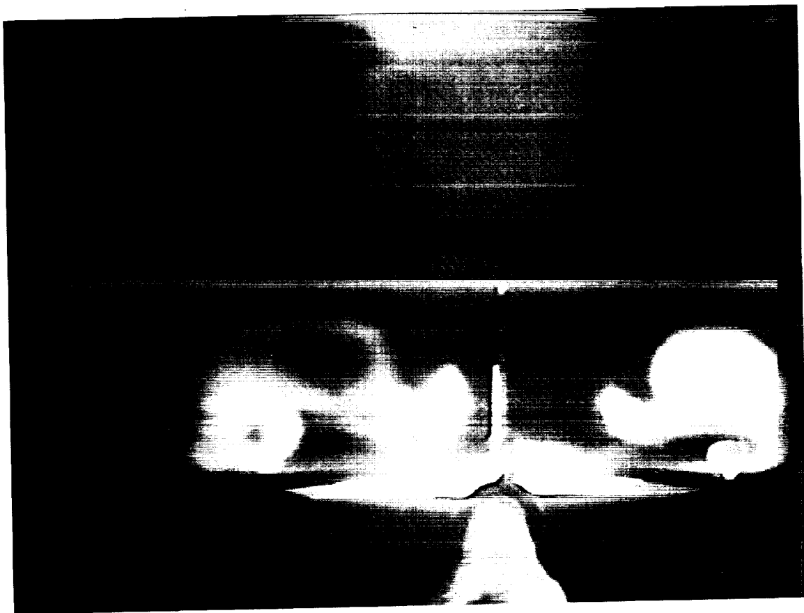
(b) Wing vortex flows in sideslip; M_\infty = 0.85 ; \alpha = 18^\circ ; \beta = -4^\circ .
