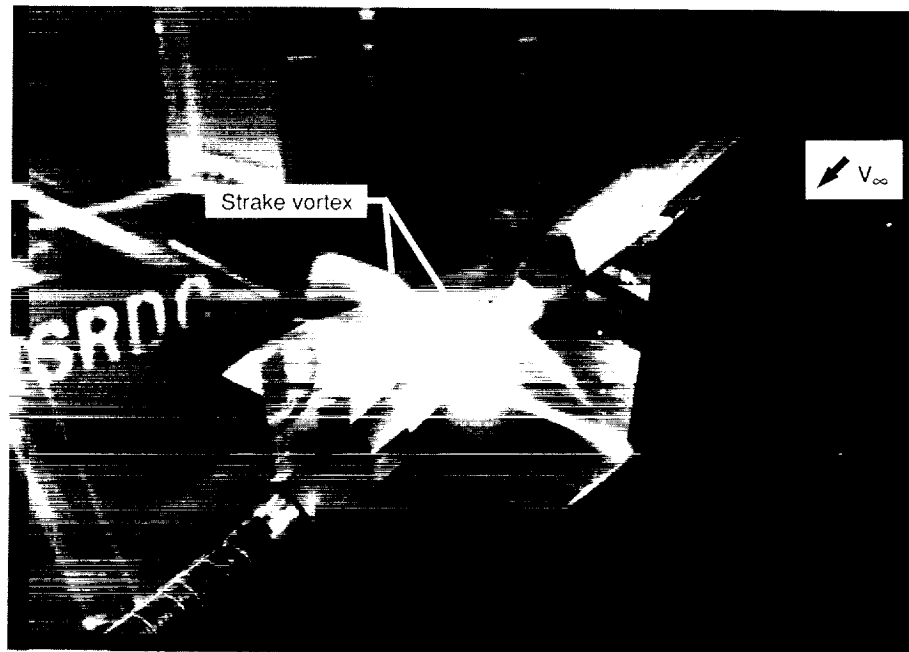
(a) M_\infty = 0.90 ; \alpha = 20^\circ .
