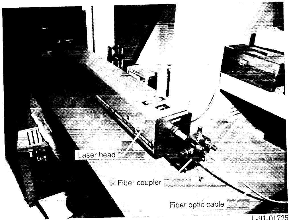
(a) Argon-ion laser head.
