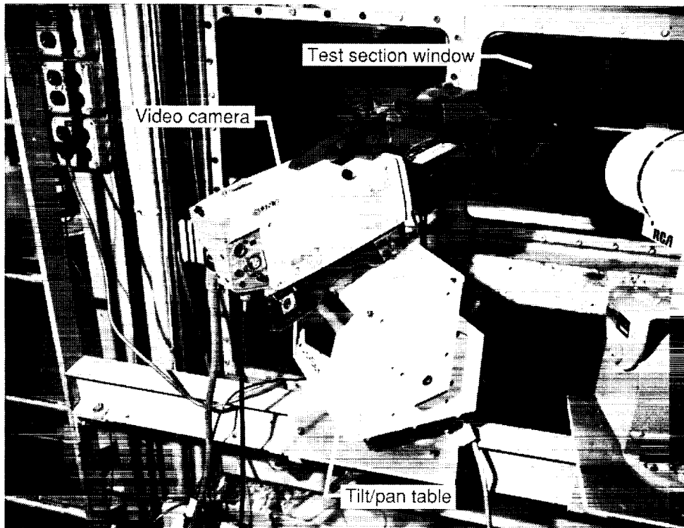
Figure 21. Photograph of color video camera on tilt/pan table.
