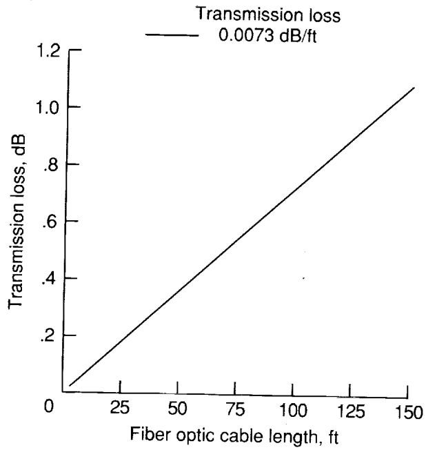
(a) Effect on transmission loss.
