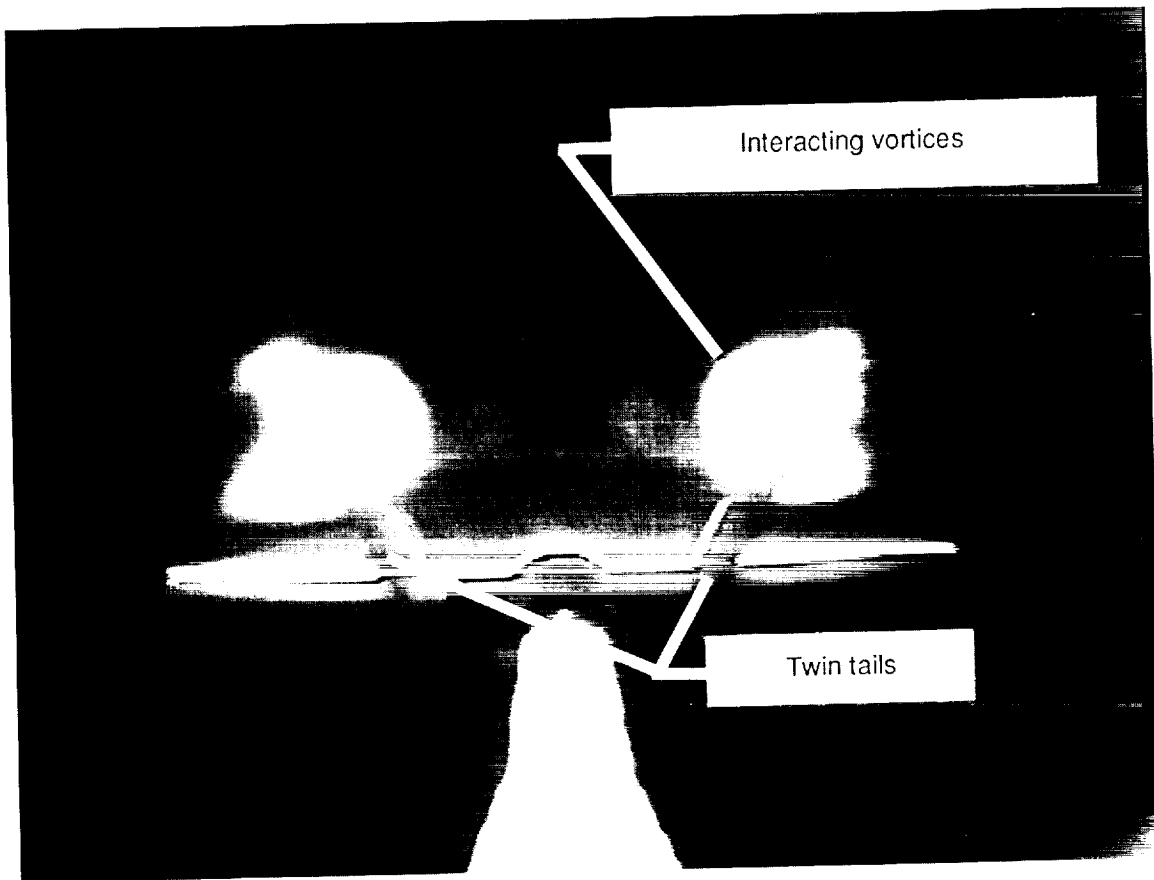
(e) Vortex-vortex and vortex-tail interactions near tail apex.
