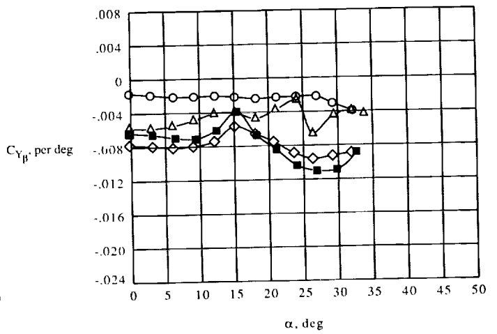
(k) Lateral-directional stability derivatives at M_\infty = 0.50 .
