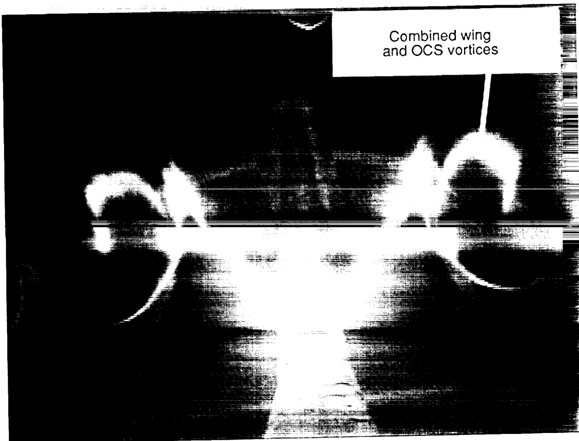
(b) M_\infty = 1.20 ; \alpha = 20^\circ (Langley 8-Foot High-Speed Tunnel).
