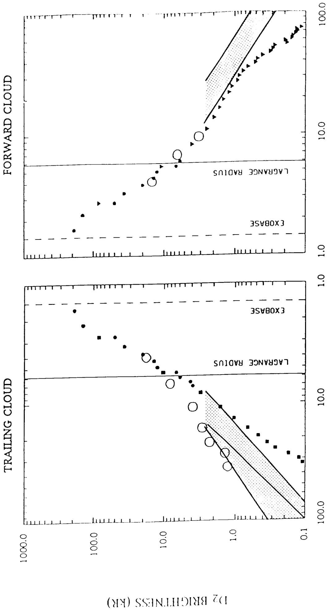
RADIAL DISTANCE FROM IO (R 10 )
