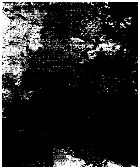
Fig. 22. Quartz grains with lamellar features.
