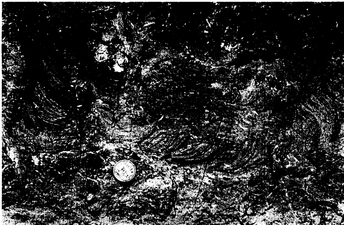
Fig. 71. El Mulato, top of unit 3, bioturbation by Zoophycos (spreiten structures).
