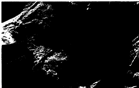
Fig. 77. La Sierrita II, Thalassinoides(?) burrows at the top of unit 3.
