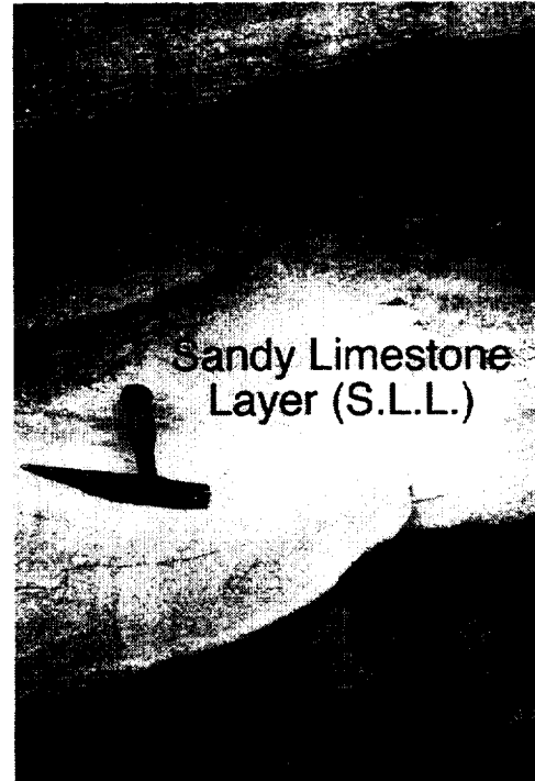
Fig. 13. Drapes of spherules over SLL.
