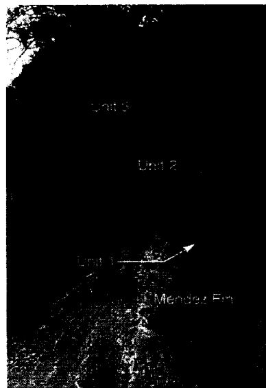
Fig. 66. El Mulato, clastic deposit showing lower contact with Mendez marls.
