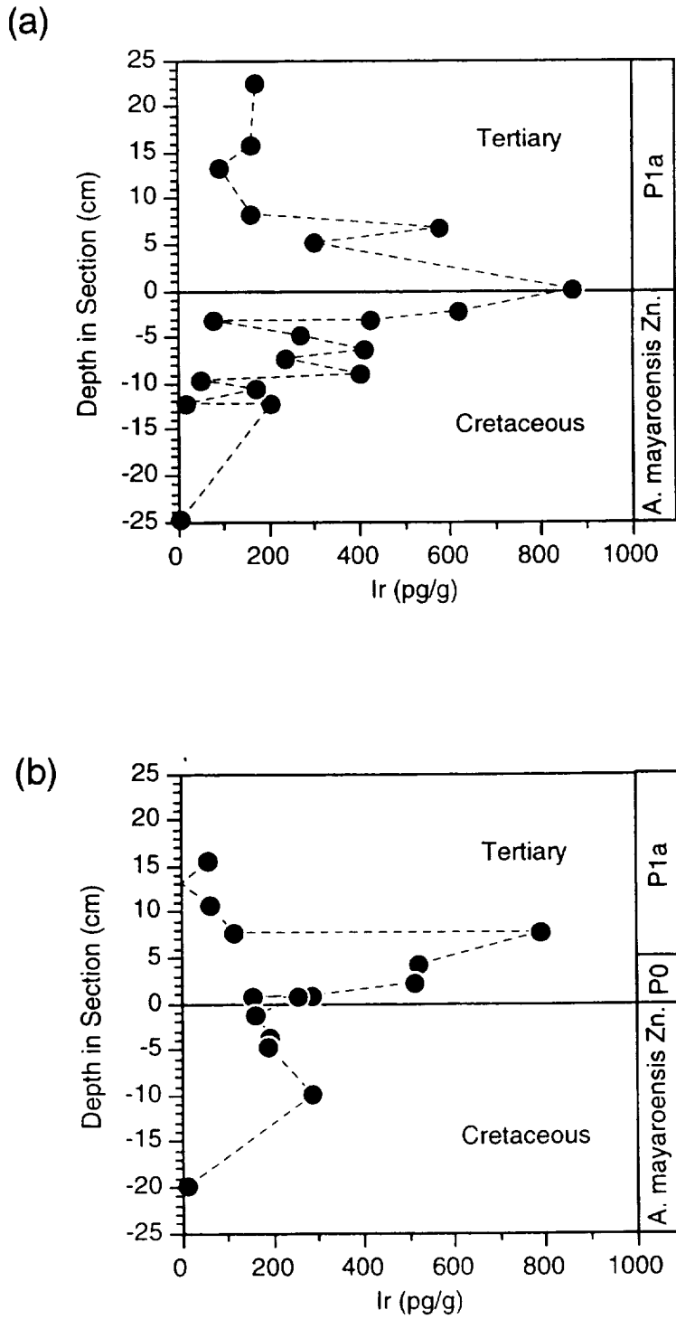
Fig. 99. Iridium concentrations at (a) El Mibrál I in the center of channel (from Smit et al., 1992), and (b) at El Mibrál II outside the channel (from Rocchia and Robin, in Stinnesbeck et al., 1993).
