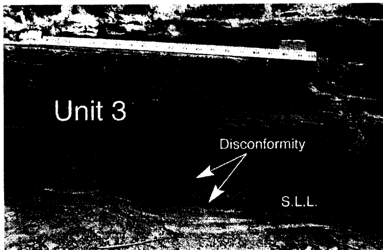
Fig. 35. La Lajilla 1, note discontinuities above and below the SLL of unit 1.
