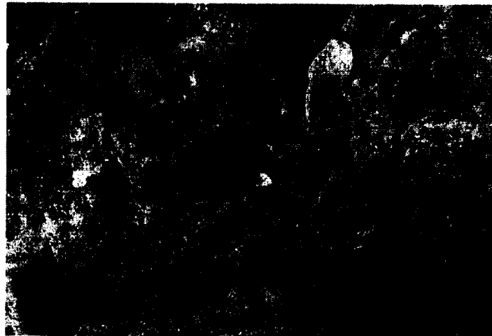
Figs. 26. Plant debris in discrete layers near the base of unit 2. See Fig. 24 for location.
