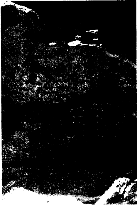
Fig. 82. Los Ramones, mudclasts at base of clastic deposit.
