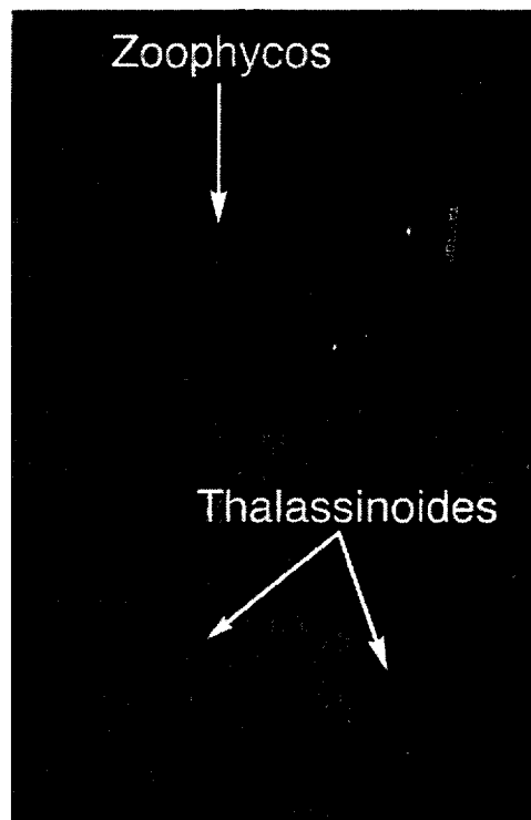
Fig. 59. Zoophycos and Thalassinoides(?) burrows near top of unit 3 at El Peñon I.
