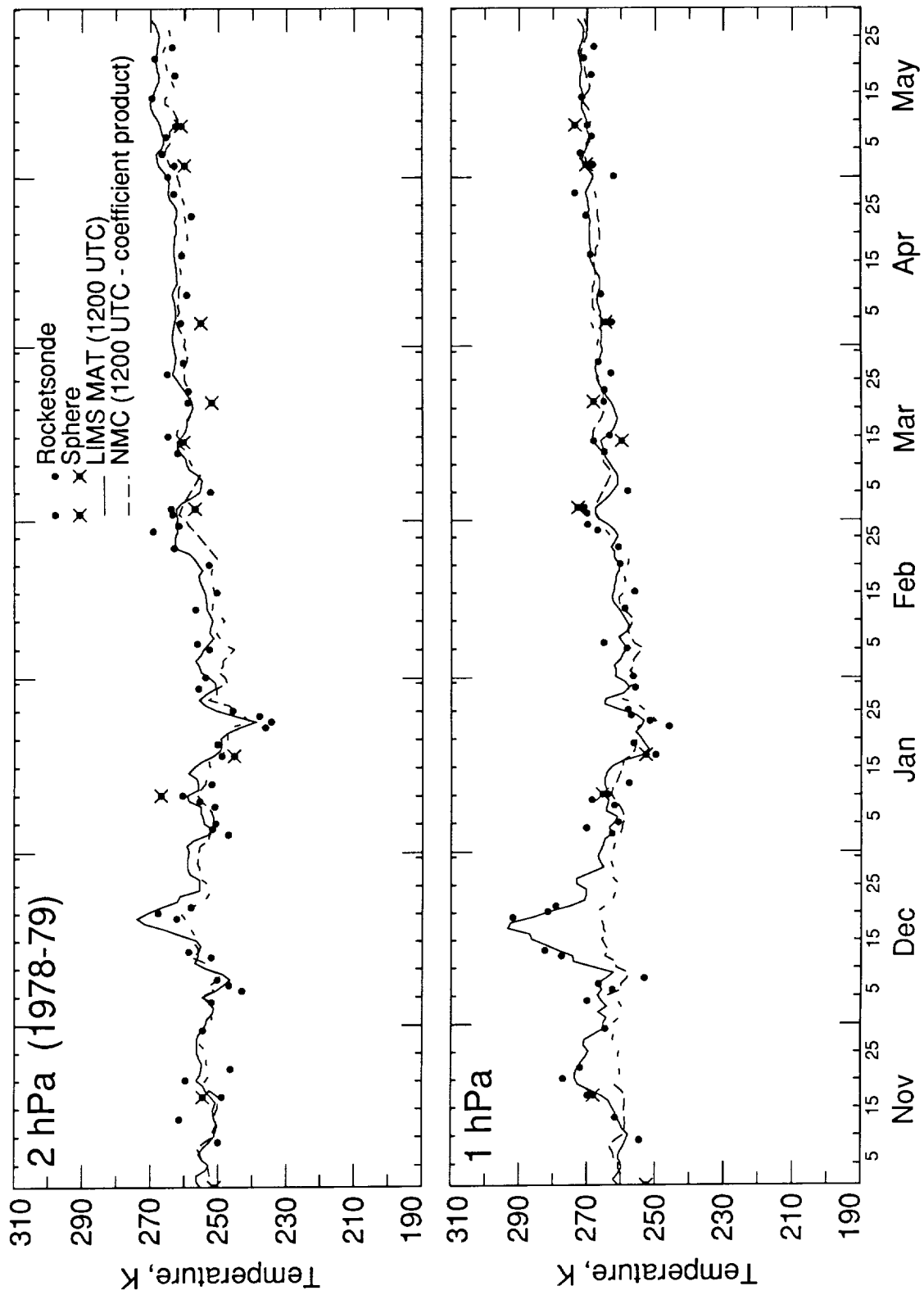
Figure A10. Continued.
