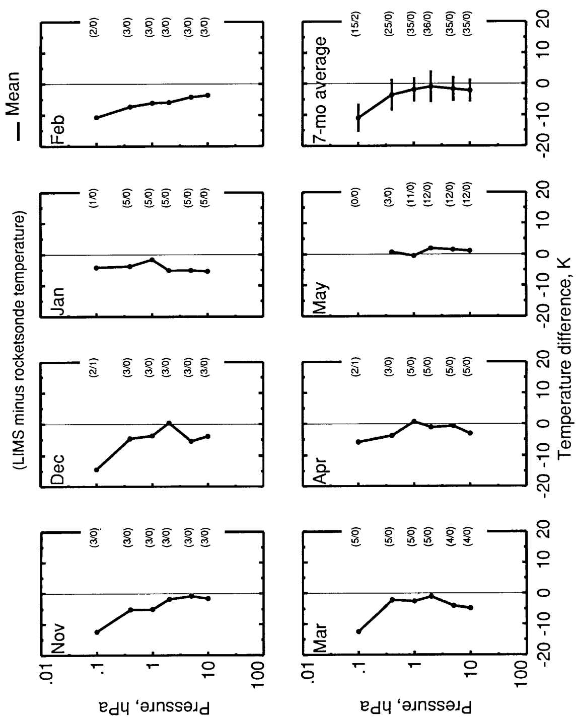
Figure A11. Concluded.
