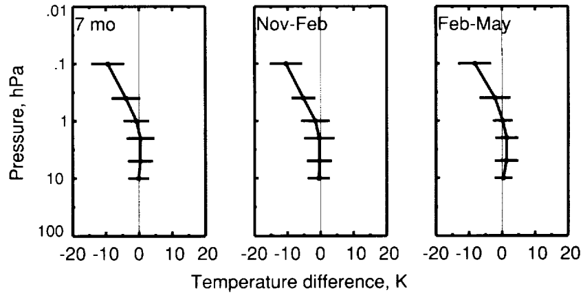
Figure 19. Seasonally averaged LIMS minus Datasonde (US) temperature differences for mid latitudes. Horizontal bars represent standard deviation about average difference.
