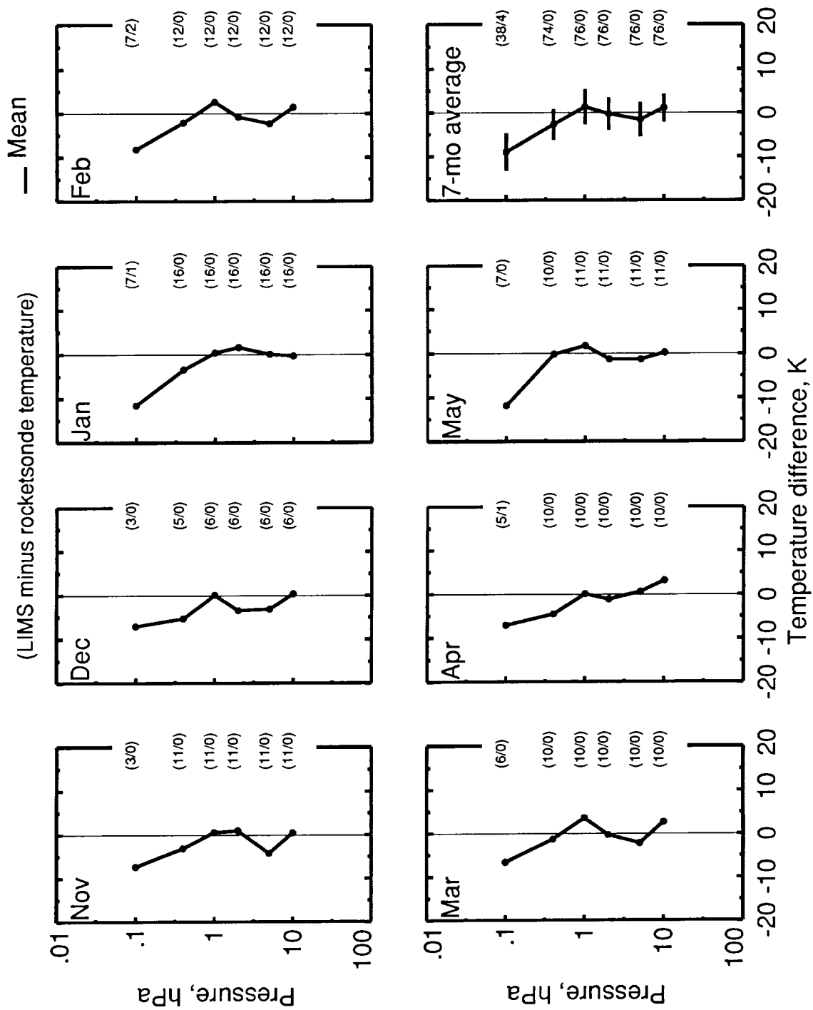
Figure A4. Concluded.
