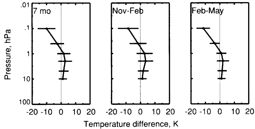
Figure 20. Seasonally averaged LIMS minus Datasonde (US) temperature differences for high latitudes. Horizontal bars represent standard deviation about average difference.
