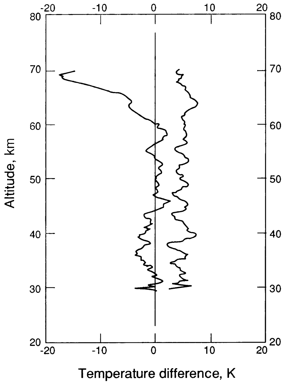
Figure 21. Sphere minus Datasonde differences from Schmidlin et al. (1991). Left curve is mean difference, right curve standard deviation of differences.
