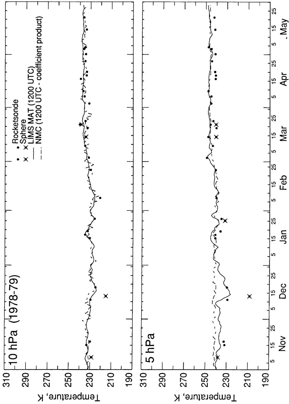
Figure A7. Barking Sands (22° N, 200° E).
