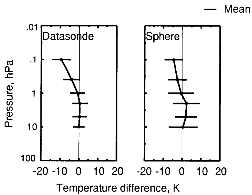
Figure 22. LIMS minus ROCOB temperature differences at mid latitudes.
