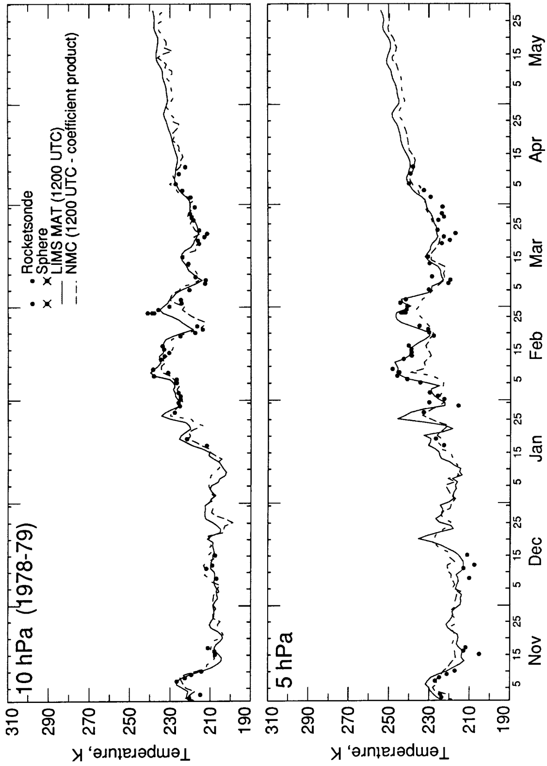
Figure A15. Fort Churchill (59° N, 266° E).
