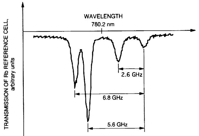
Fig. 9. The transmission spectrum of the absorption cell at a temperature of 300 K.
