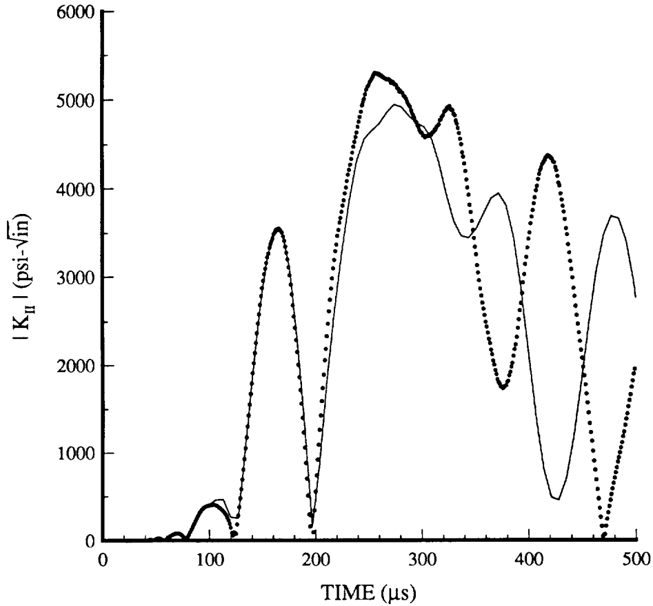
Figure 5: Comparison of K_{II} from spectral (—) and finite element ( \cdots ) methods for the plane strain problem.
