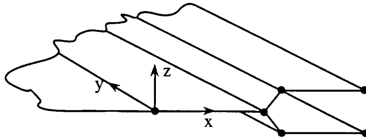
Figure 2: Spectral element discretization of an edge delamination crack.
