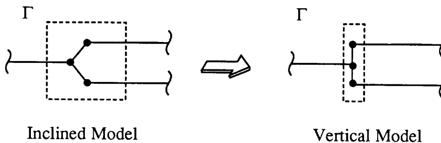
Figure 4: Zero volume J integral path showing the use of vertical spectral elements.
