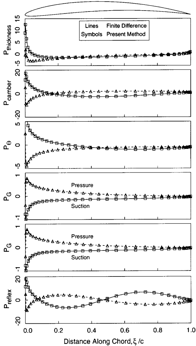
Figure 3: Sensitivity of steady surface pressure of cascade of NACA 5506 airfoils to perturbations in thickness, camber, stagger, gap, and reflex. M_{-\infty} = 0.5 , \beta_{-\infty} = 55^\circ , \Theta = 45^\circ .
