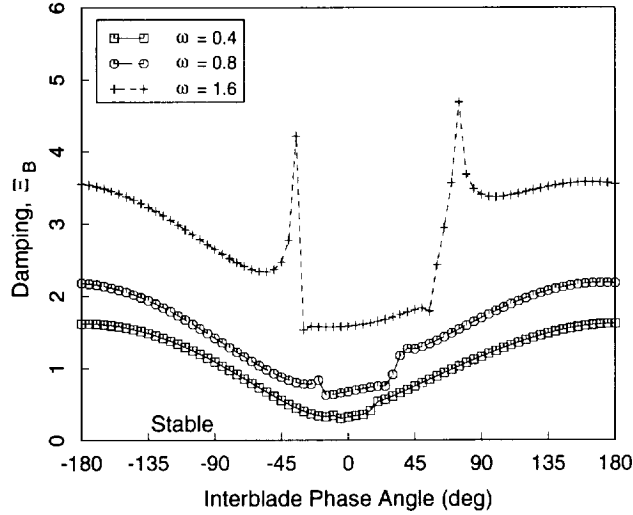
Figure 4: Aerodynamic damping of cascade of NACA 5506 airfoils vibrating in plunge at frequencies of 0.4, 0.8, and 1.6 for a range of interblade phase angles.
