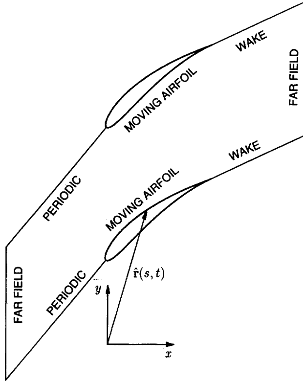
Figure 1: Typical solution domain used for calculation of flow through cascades. Five main boundary types are moving airfoil, upstream periodic, downstream wake, upstream far field, and downstream far field.
