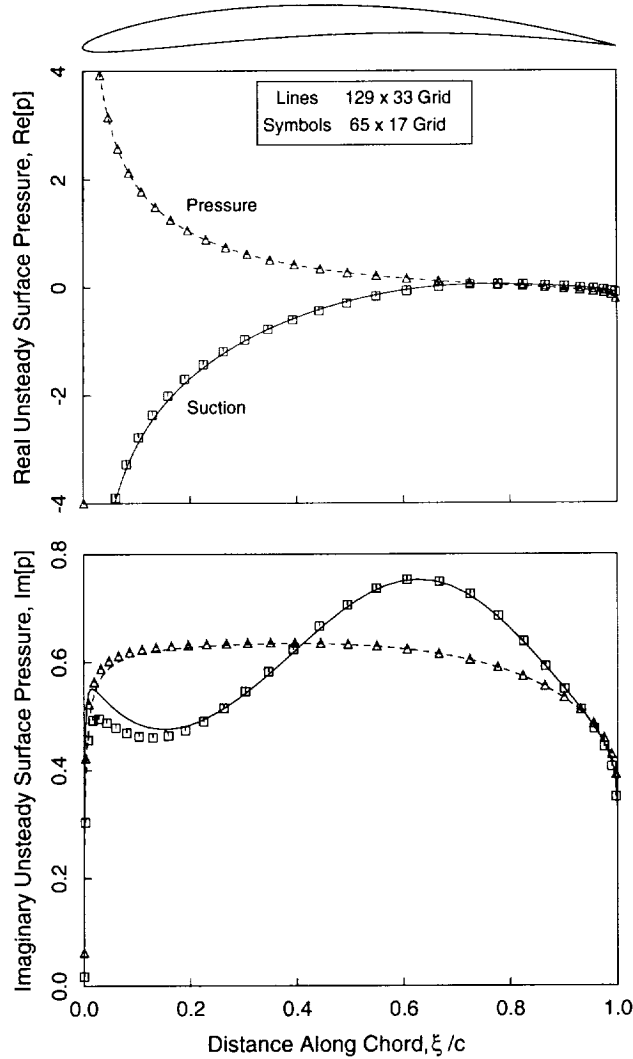
Figure 6: Real and imaginary parts of unsteady surface pressure of NACA 5506 airfoils pitching about their midchords. \omega = 0.4 , \sigma = 60^\circ .
