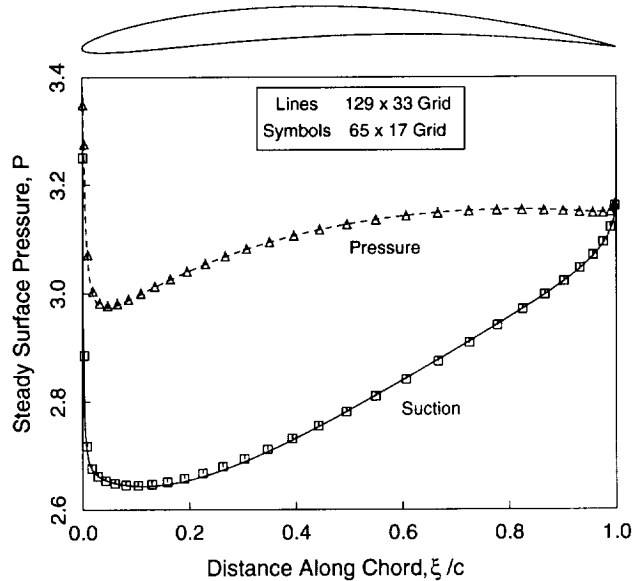
Figure 2: Steady surface pressure of cascade of NACA 5506 airfoils. M_{-\infty} = 0.5 , \beta_{-\infty} = 55^\circ , \Theta = 45^\circ .
