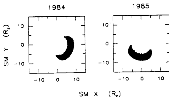
Fig. 3. Spatial extent of selected CCE data sets in Solar Magnetic (SM) coordinates. These extend in geomagnetic latitude from -16° to +12°. Equivalent regions are used for ISEE 1 data as well (see text).
