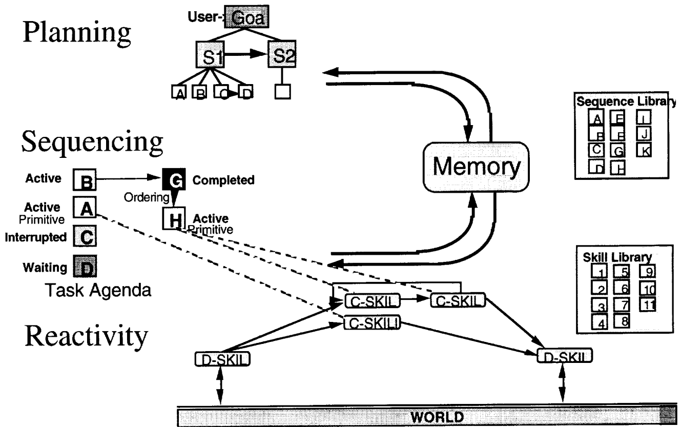
Figure 1: The flow of information through MIAA.
