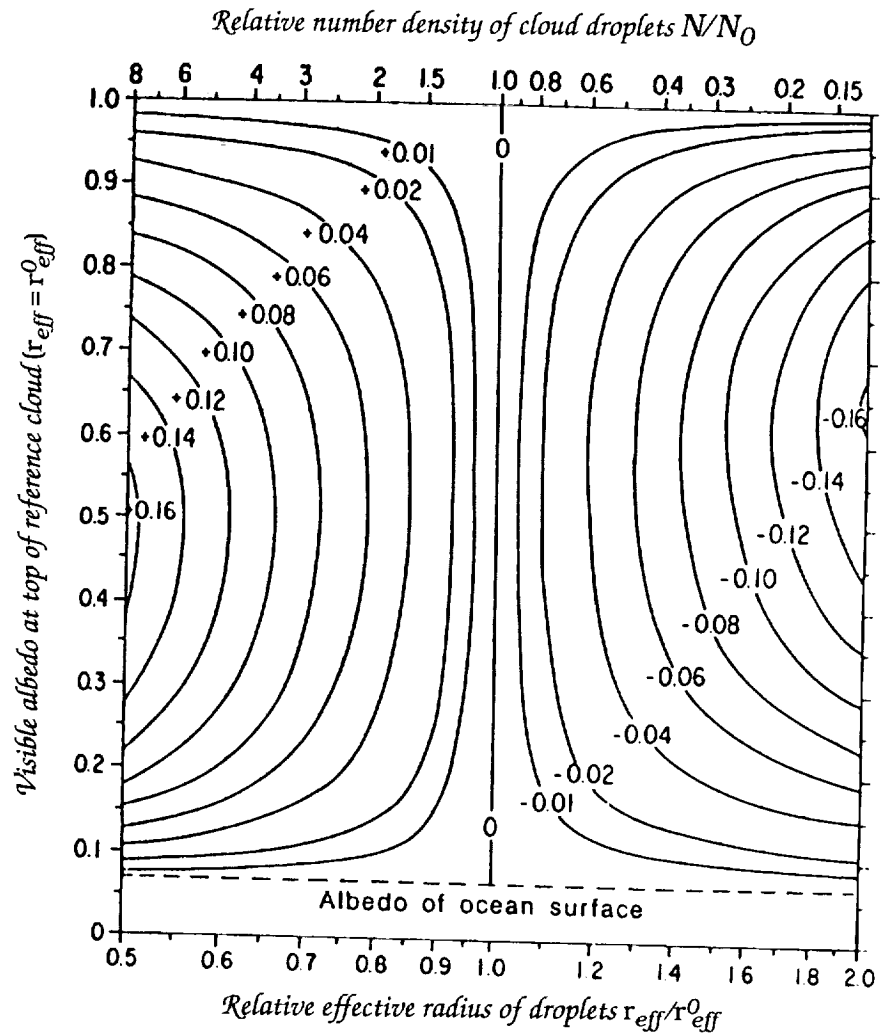
Figure 3. Contours showing change of visible albedo caused by changing droplet number density N or equivalently droplet effective radius r_{\text{eff}} relative to a reference cloud ( N_0, r_{\text{eff}}^0 ). Albedo at top of reference cloud given on left-hand vertical scale (adapted from Charlson et al., 1987; reprinted by permission from Nature, © 1987 Macmillan Magazines Ltd.).
