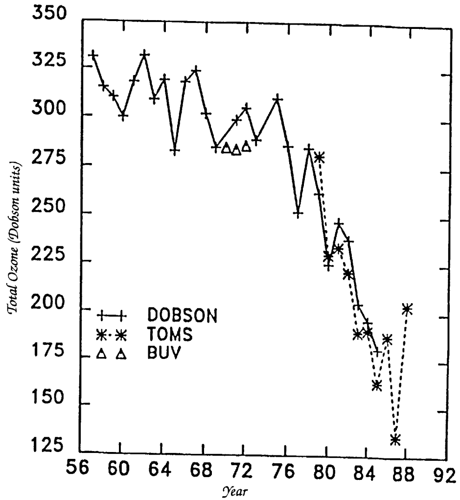
Figure 16. October monthly mean total ozone measurements over Halley Bay as measured by Halley Bay Dobson and Nimbus 4 BUV (backscatter ultraviolet) instruments. The polar minimum values for TOMS (total ozone mapping spectrometer) for October are also shown. Dobson unit is 2.7 \times 10^{16} ozone molecule per \text{cm}^2 (Schoeberl et al., 1989; Stolarski, 1988).
