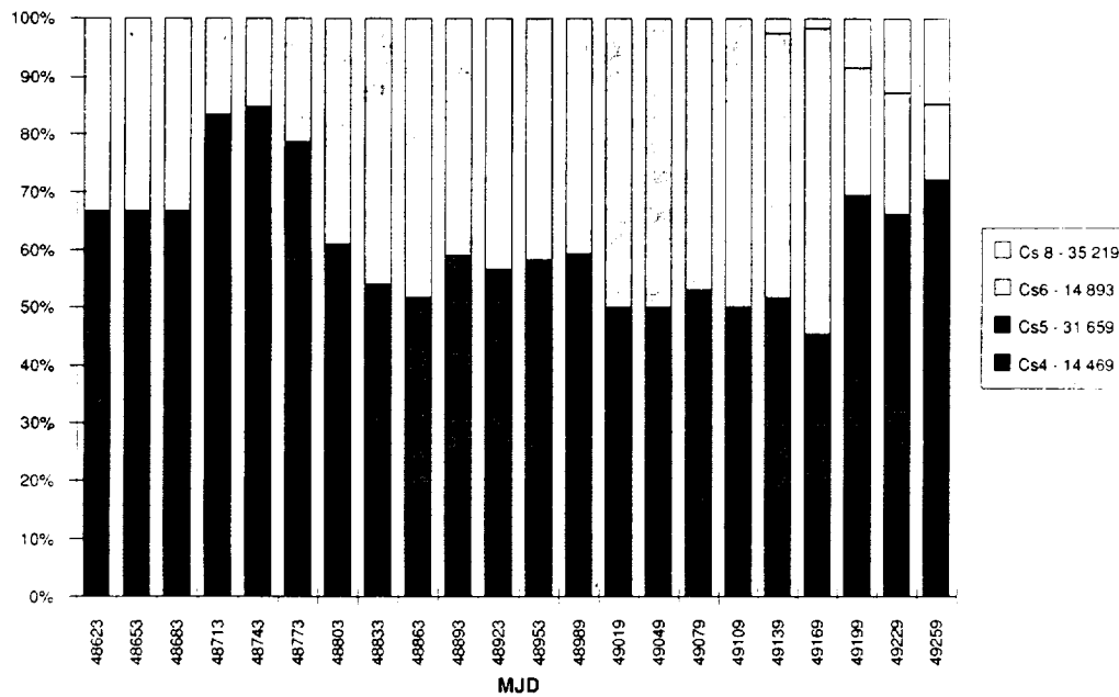
Fig. 8 - Relative weights of the clocks used in the TA(IEN) time scale.
