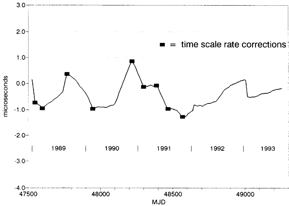
Fig. 2 - UTC(IEN) vs. UTC from January 1989 to September 1993.
