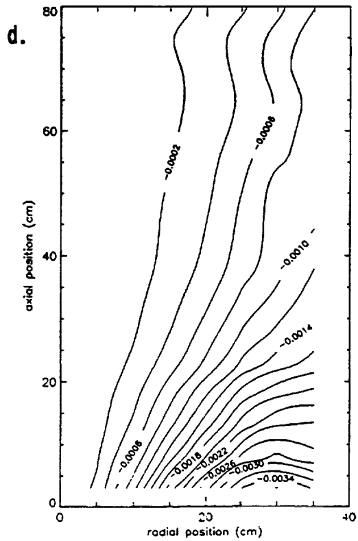
Figure 10. Contours of constant magnetic flux for a 6 MW helium discharge at (a) 0 ms, (b) 4 ms, (c) 10 ms, and (d) 14 ms.
