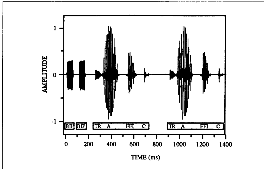
Figure 4. Arrangement of the pre-alert and traffic enunciation used for TCAS advisories in the experiment.
