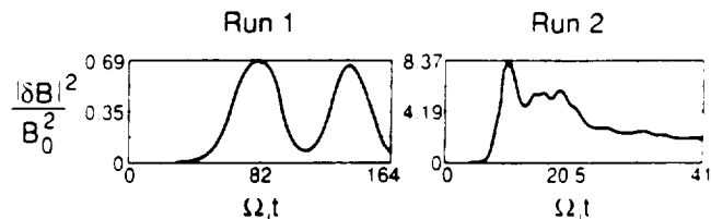
Fig. 4. The temporal evolution of the fluctuating magnetic energy of the system normalized to the initial magnetic energy |\delta B|^2/B_0^2 . Here, as in Figs. 5 through 7, the left panels depict results from the computer simulation labeled Run 1, whereas the right panels show results from Run 2.
