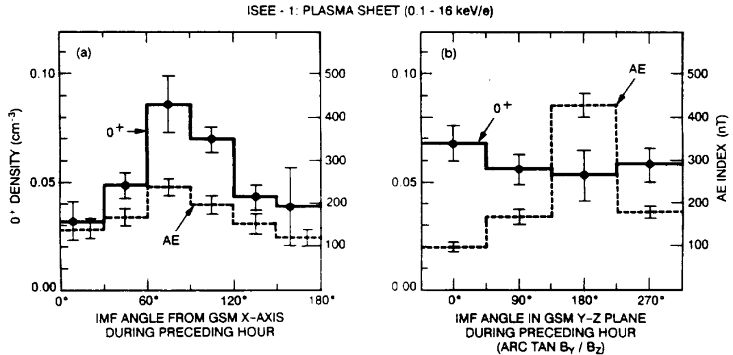
Fig. 5. (a) Average O + density (solid line) ordered by the angle between the Earth-Sun line ( X -axis) and the IMF direction. (b) Same density ordered by the rotation angle of the IMF around the Sun-Earth line. The concurrent average AE index is also indicated (dashed lines, scale on the right).
