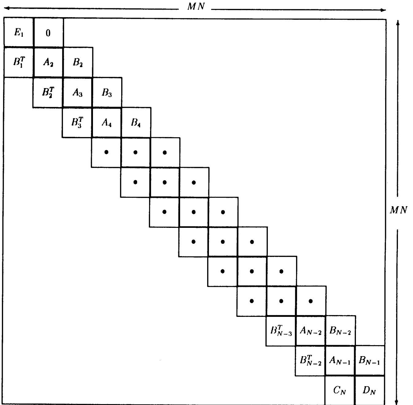
Figure 2: Structure of the global stiffness matrix, [A] , with minor blocks.
