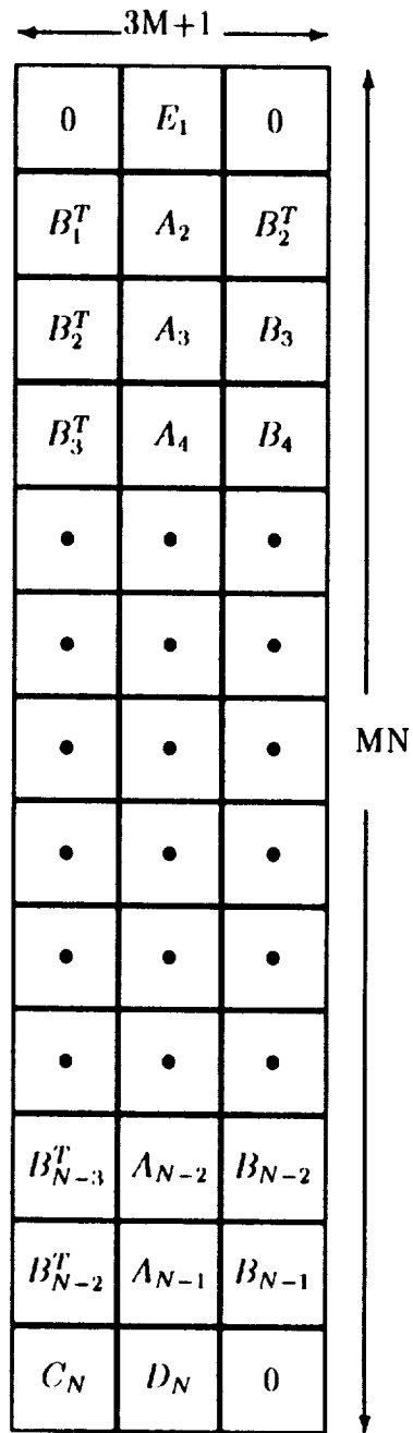
Figure 3: The stored MN \times (3M+1) rectangular coefficient matrix with nonzero coefficients.
