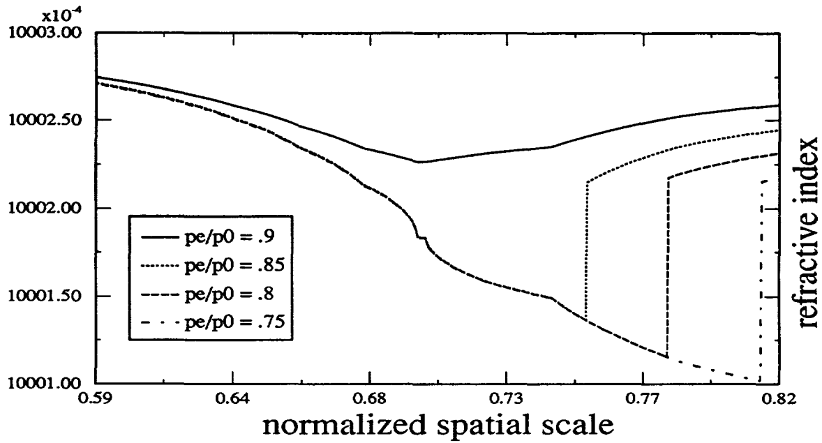
Figure 5: Theoretical refractive index in minimum throat region.
