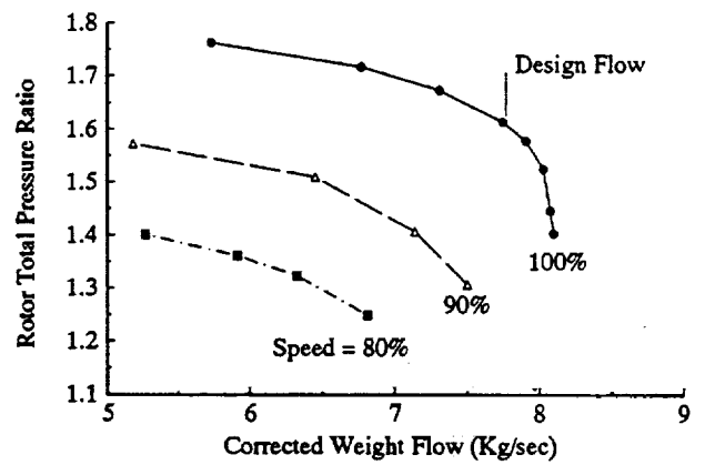
(b) Rotor Total Pressure Ratio
