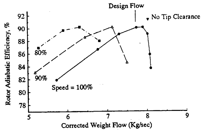
(a) Rotor Adiabatic Efficiency
