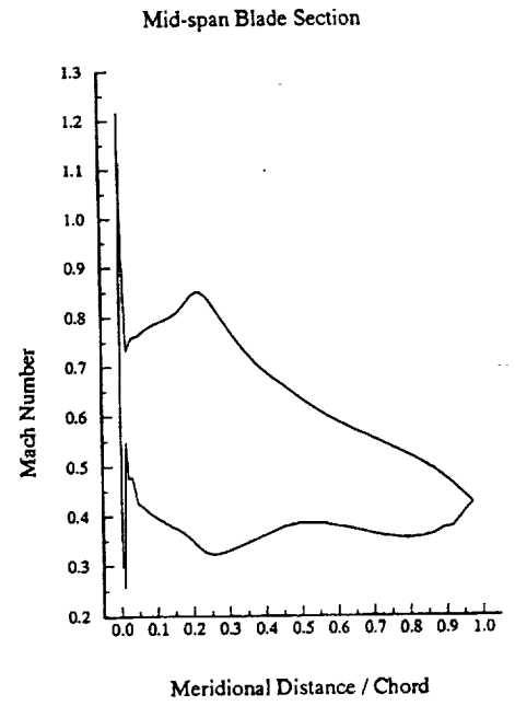
Fig. 20 Typical stator surface Mach number distribution
