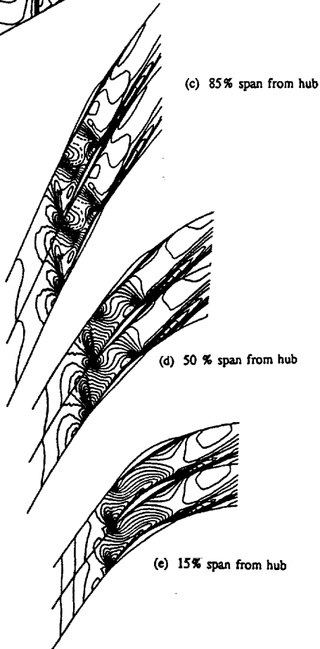
Fig. 9 Rotor relative Mach number at design flow
