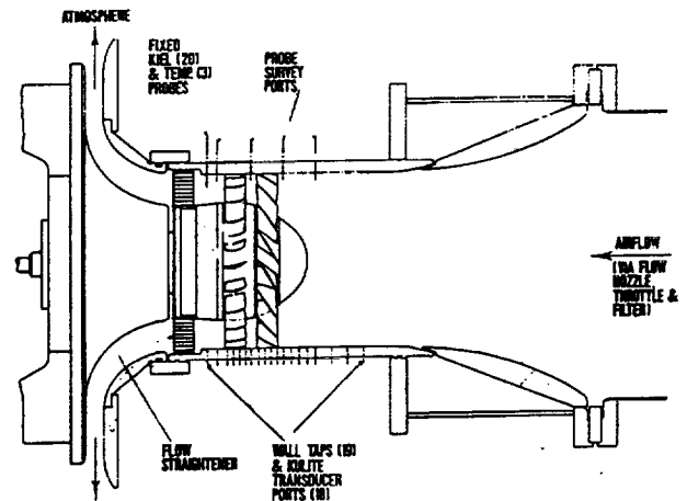
(b) Existing transonic stage (Vavra design)
