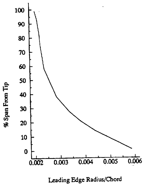
Fig. 5 Rotor Leading Edge Radius/Chord
