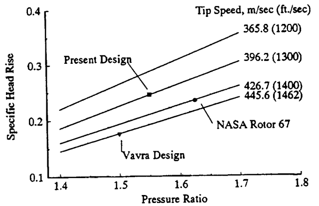
Fig. 2 Specific Head Rise
