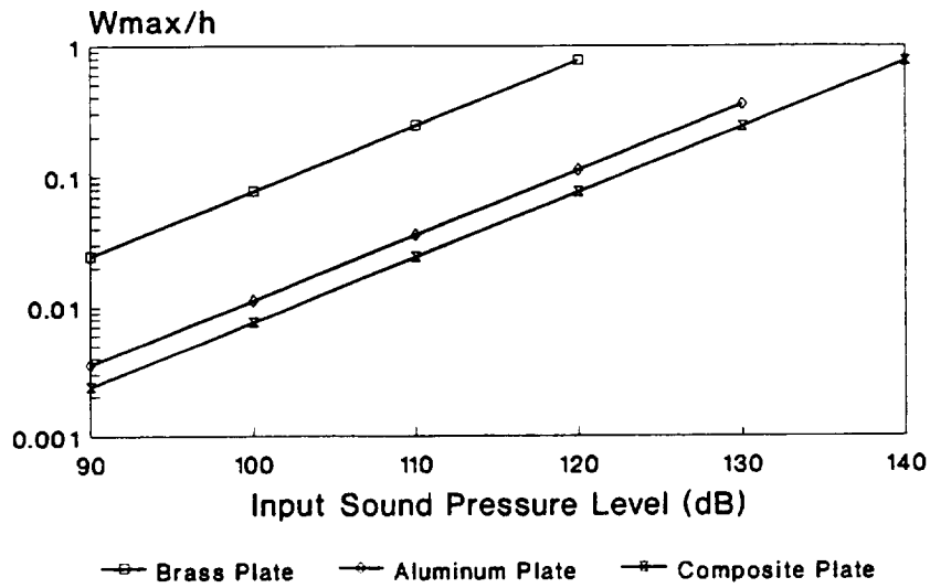
Figure 4.33 Harmonic Response of Simply Supported Panels.
