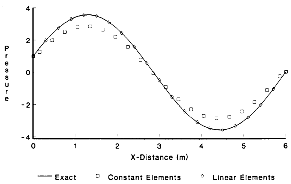
Figure 4.2 Open Outlet Rectangular Duct Results.
