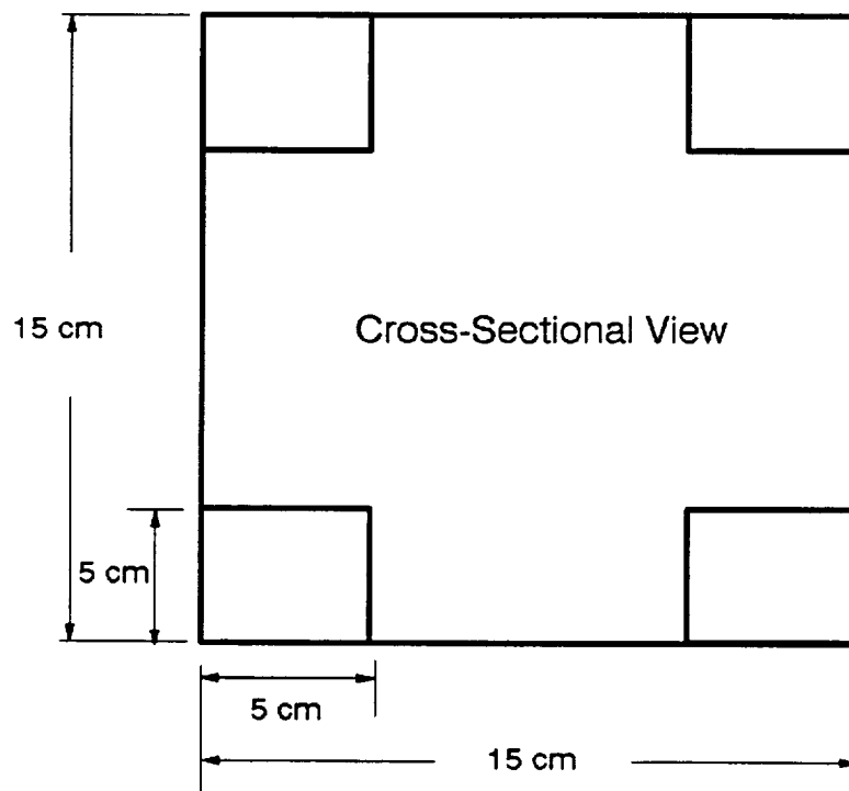
Figure 4.17 Four-Inlet and Outlet Irregular Duct System.
