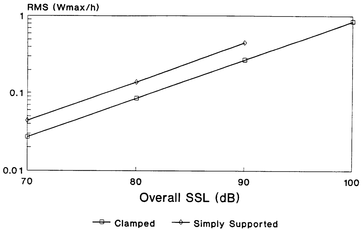
Figure 4.39 Random Response of Clamped and Simply Supported Panels in the TAFE Facility.
