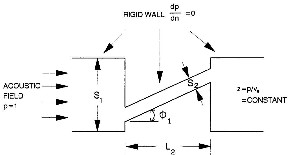
Figure 4.9 Three-Section Rectangular Duct.
