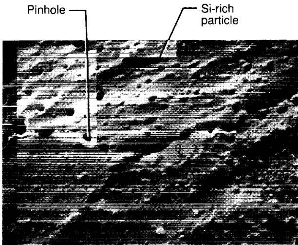
(b) After dynamic oxidation for 12.5 hr.
