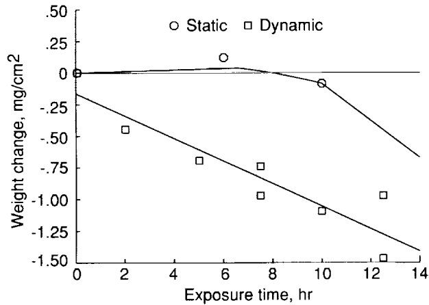
(a) Short-time oxidation data.
