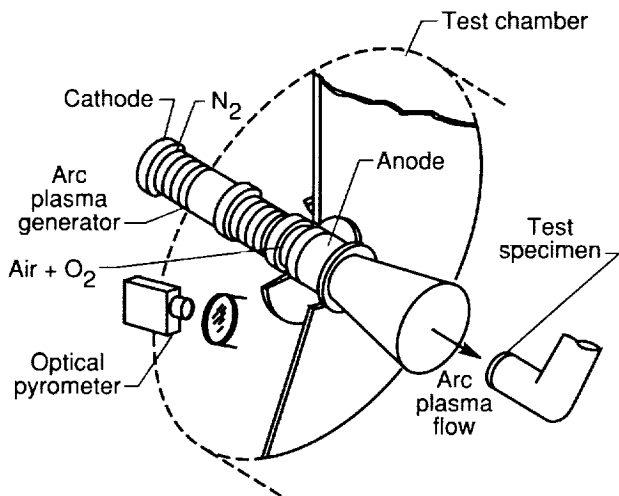
Figure 1. Schematic diagram of HYMETS facility.
