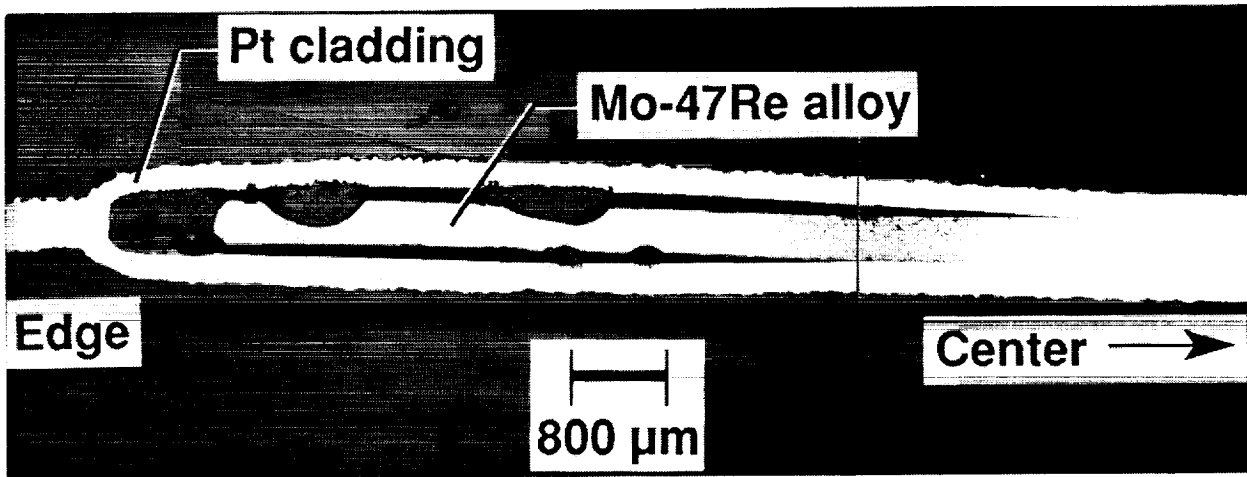
(b) After static oxidation for 140 hr.
