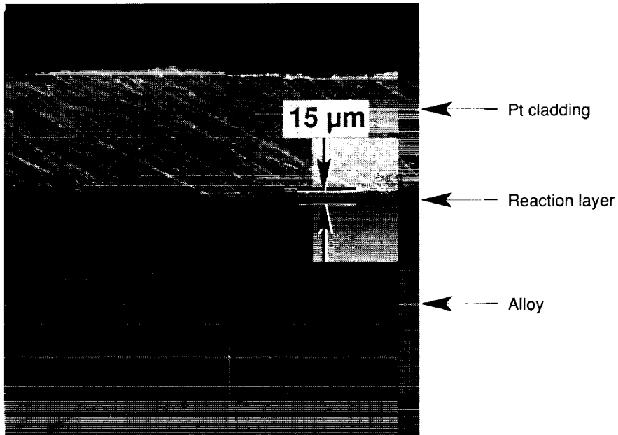
(a) With no oxidation.
