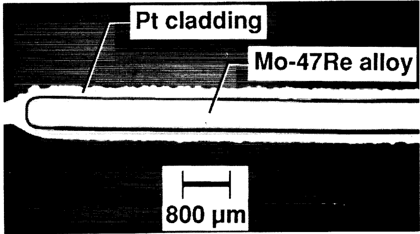
(a) With no oxidation.
