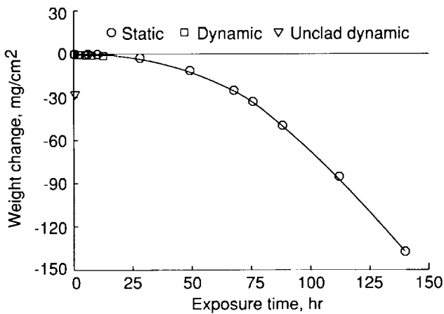
(b) Long-time oxidation data.
