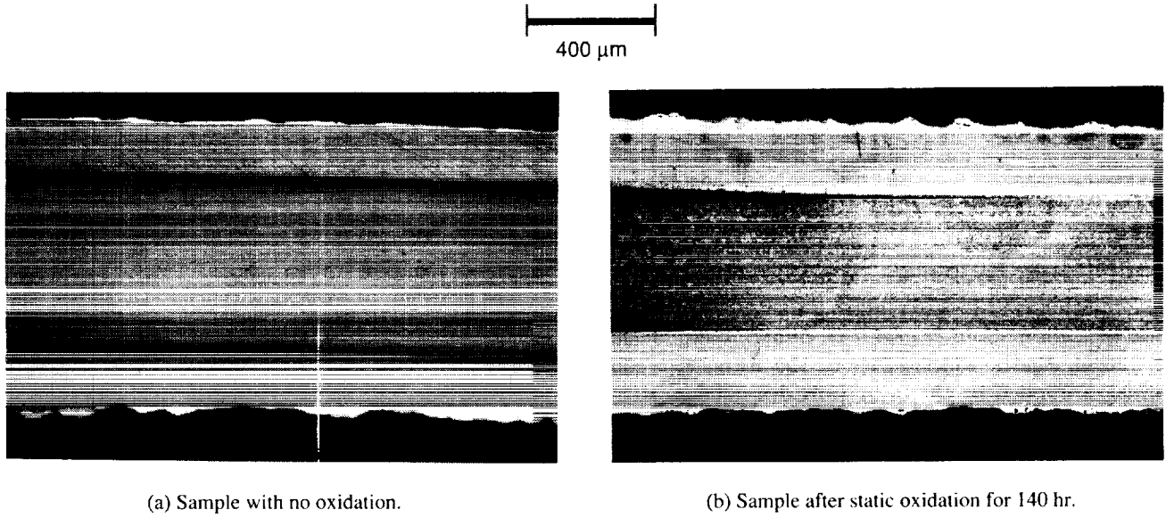
Figure 7. Separation of cladding from alloy of Pt-clad Mo-47Re sample after static oxidation exposure for 140 hr.
