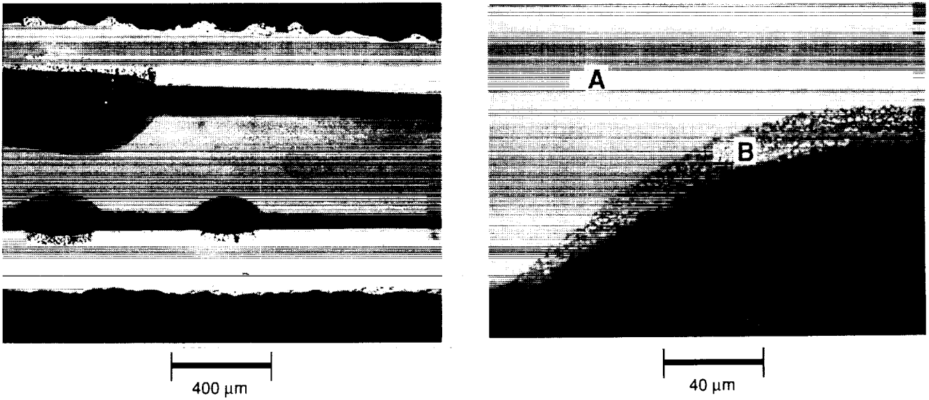
Figure 8. Details of intense oxidation attack of Pt-clad Mo-47Re sample after static oxidation exposure for 140 hr.
