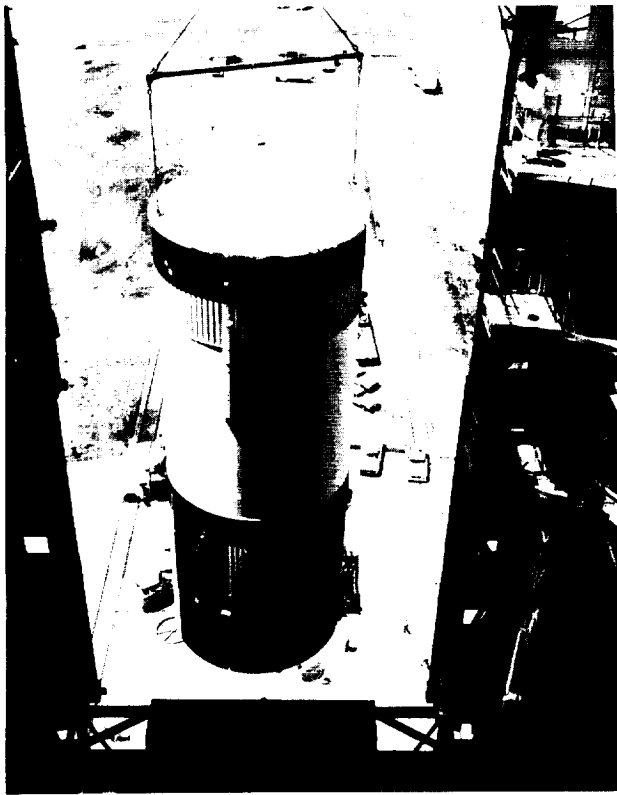
The Saturn S-IVB second stage is hoisted aloft for mating to the remainder of the launch vehicle at the Kennedy Space Center in 1968. NASA Photo #68-H-386.
