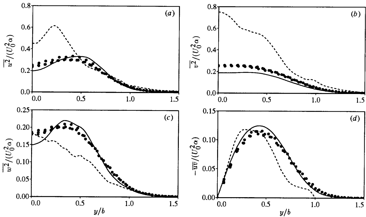
Figure 6. Comparison of the time-averaged (in scaled coordinates) profiles of \overline{u^2} , \overline{v^2} , \overline{w^2} , and \overline{uv} normalized by U_0^2 \alpha from —, the unforced wake simulation, ---- the forced wake simulation, and • the experiments of Ref. 9.
