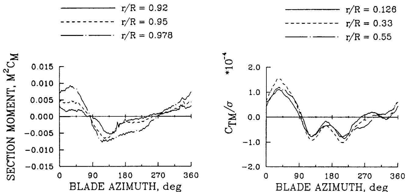
(a) Oscillatory aerodynamic section moment near the blade tip
