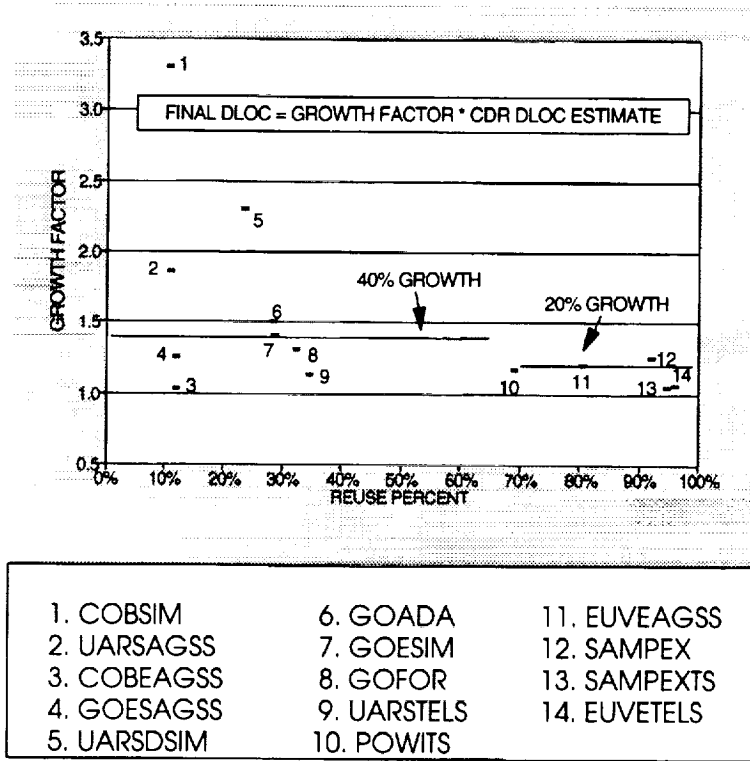
Figure 3-4. DLOC Growth Factors: Actual DLOC Divided by CDR Estimate
