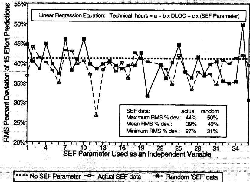
Figure 4-6. Accuracy of Effort Prediction (Measured by RMS Percent Deviation) for 15 Recent FORTRAN Projects
