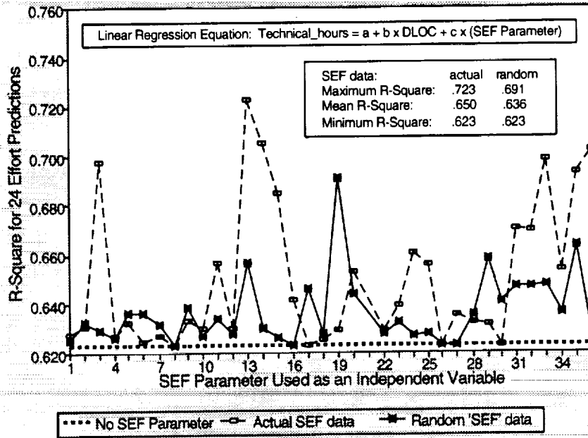
Figure 4-3. Accuracy of Effort Prediction (Measured by R-Squared) for 24 Older FORTRAN Projects
