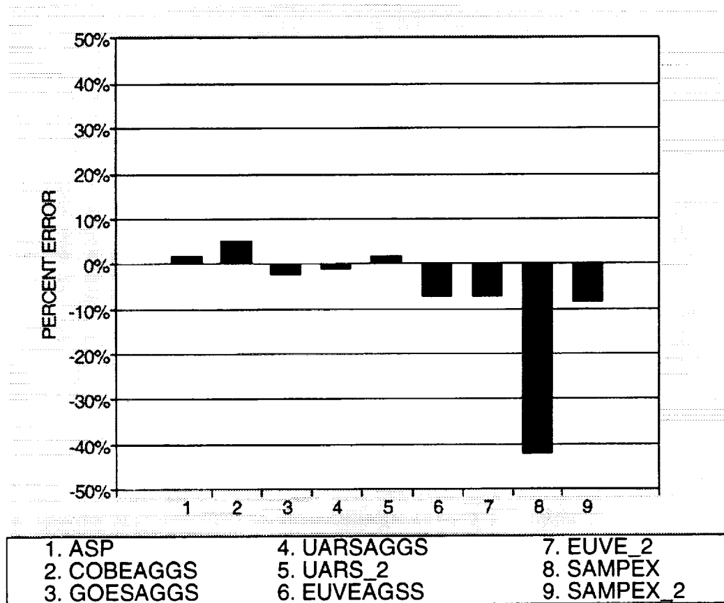
Figure 5-3. Accuracy of Schedule Duration Model for AGSSs (Based on Actual Technical and Management Effort)
