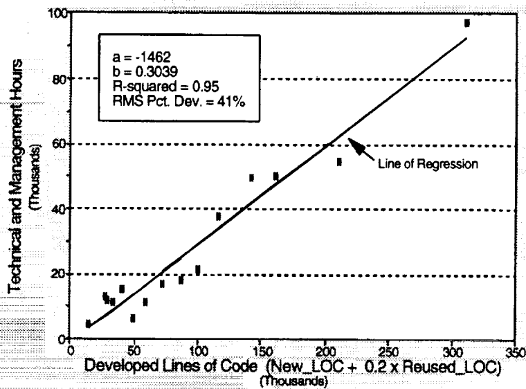
Figure 4-2. Effort as a Function of DLOC for 15 Recent FORTRAN Projects
