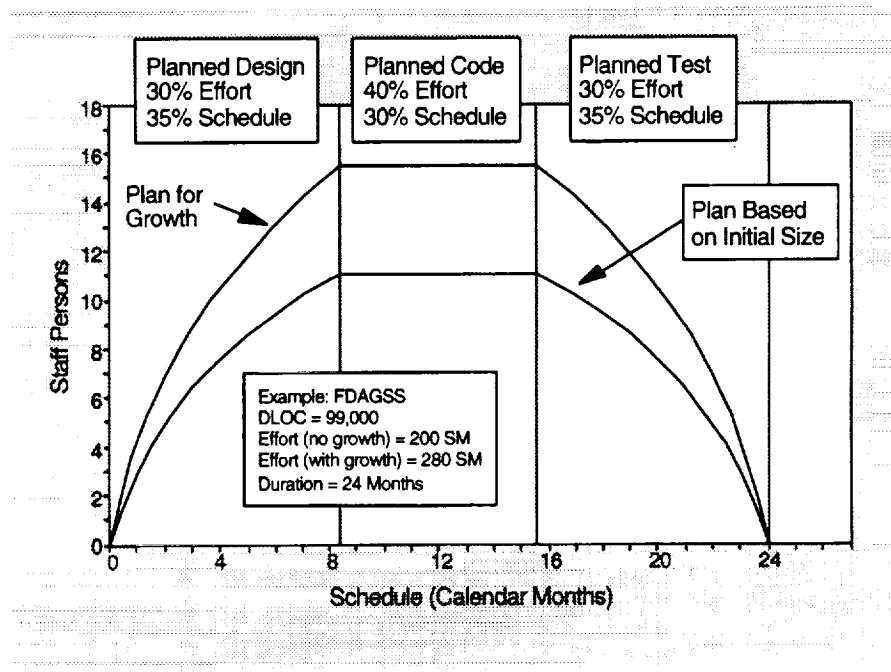
Figure 7-2. Staffing Plan That Anticipates Growth
