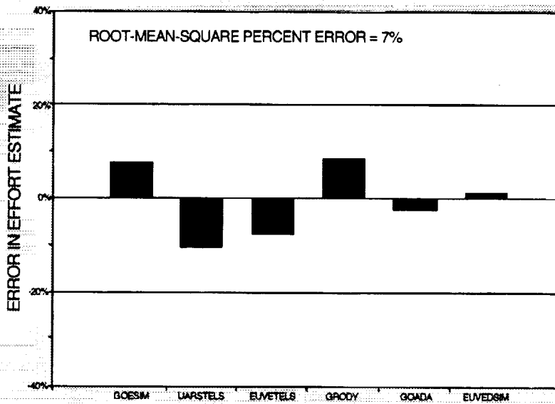
Figure 3-3. Accuracy of Ada Effort Estimation Model
