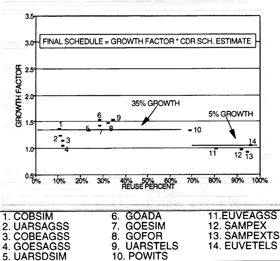
Figure 5-5. Schedule Growth Factors (Actual Duration Divided by CDR Estimate)
