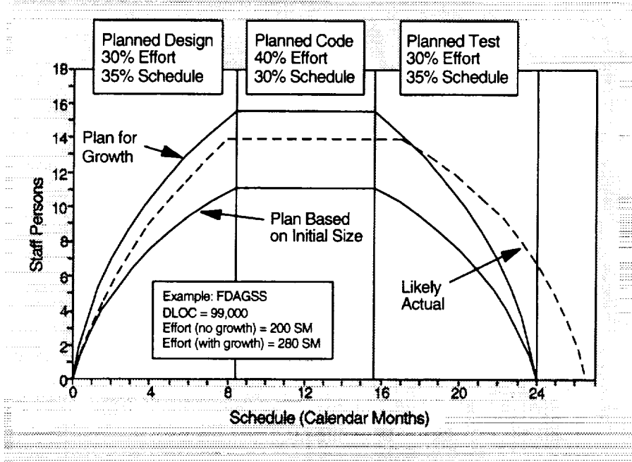
Figure 7-3. Plan Versus Actuals
