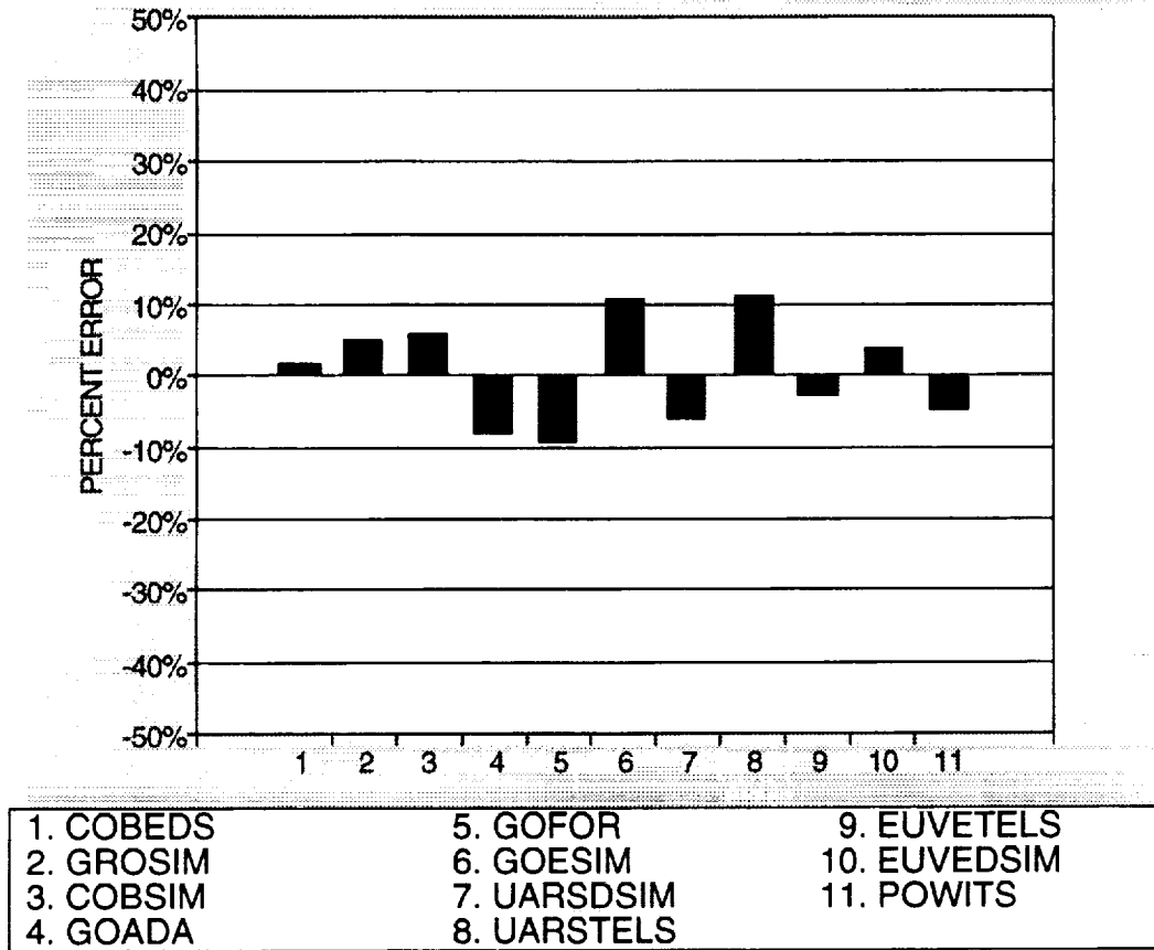
Figure 5-4. Accuracy of Schedule Duration Model for Simulators (Based on Actual Technical and Management Effort)
