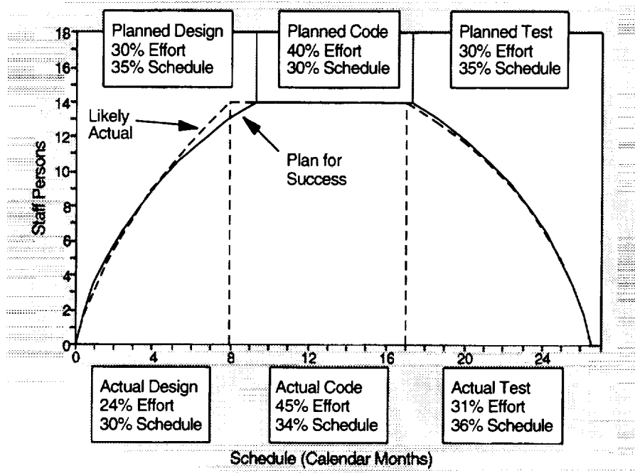
Figure 7-5. Planning Model Versus Baseline Model (Expected Actuals)
