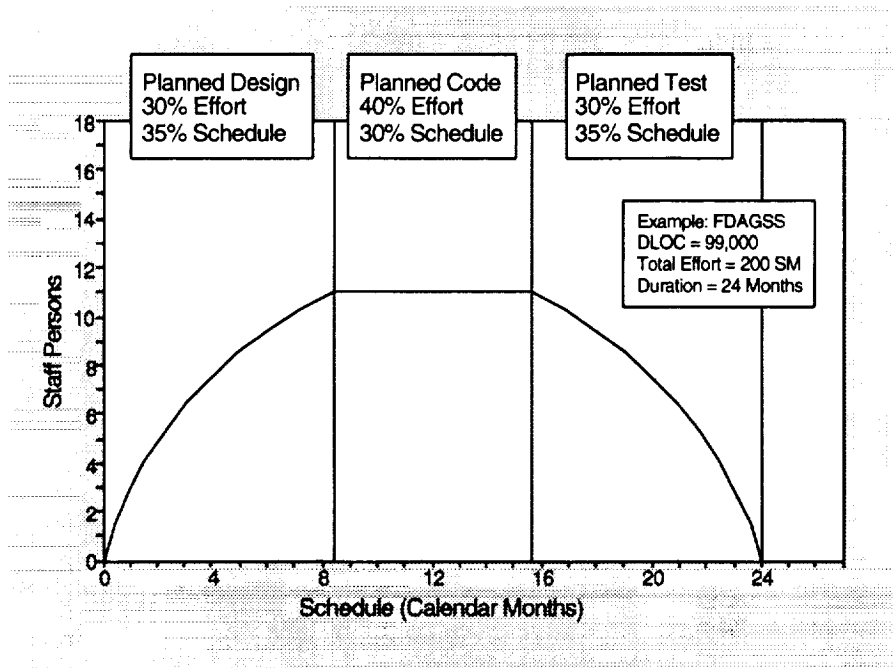
Figure 7-1. Staffing Plan Based on Initial Size
