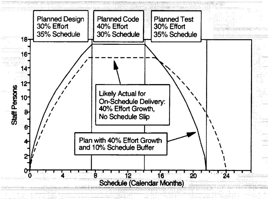
Figure 7-4. Plan for Success
