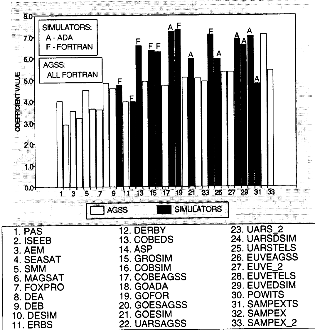
Figure 5-1. Coefficients of Schedule Duration Formula
