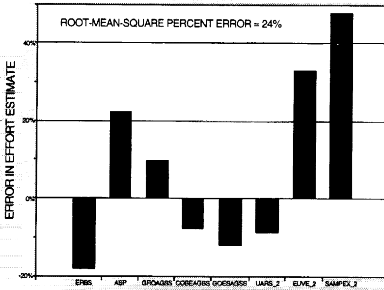
Figure 3-2. Accuracy of FORTRAN Effort Estimation Model
