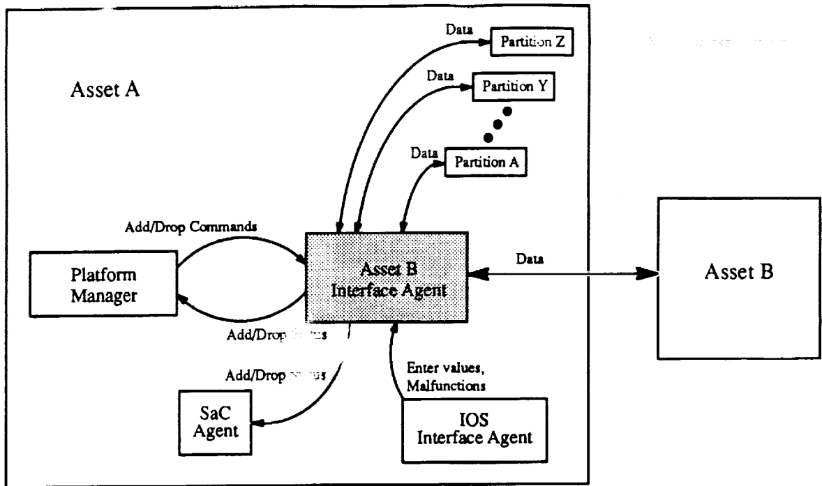
Figure 4.8-2 General Interface Agent Association Diagram
