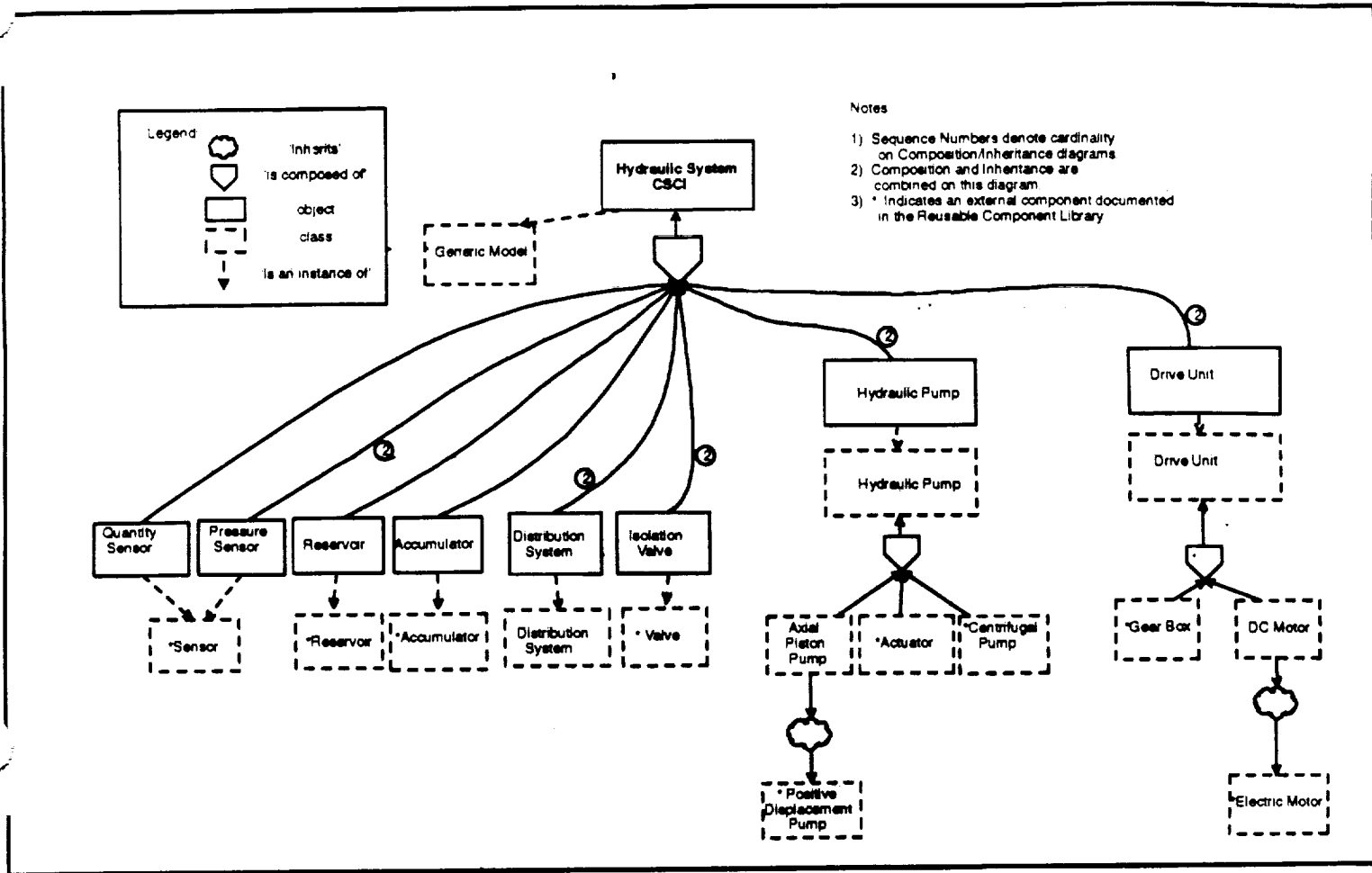
Figure 6 Hydraulic System Composition Diagram
