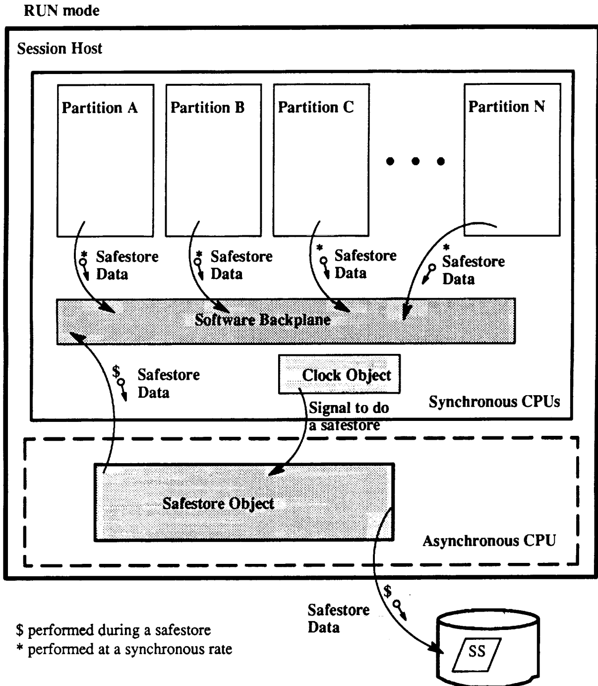
Figure 4.7-1. Taking a Safestore
