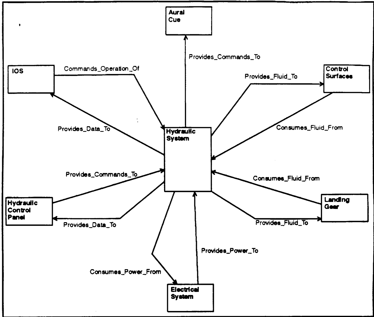
Figure 3 Hydraulic System External Association Diagram
