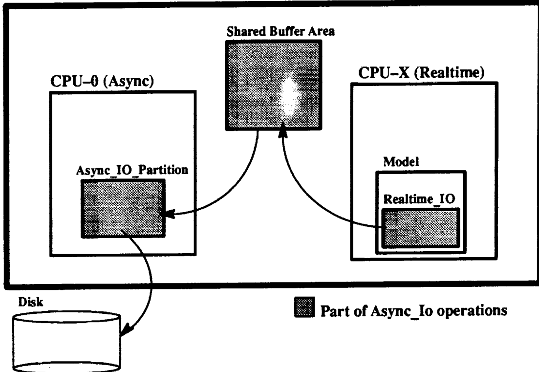
■ Figure 4.9-1 Asynchronous I/O Overview
