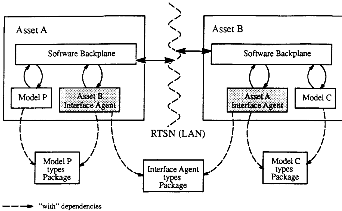
Figure 4.8-7 General Interface Agents within Two Assets with SVM
