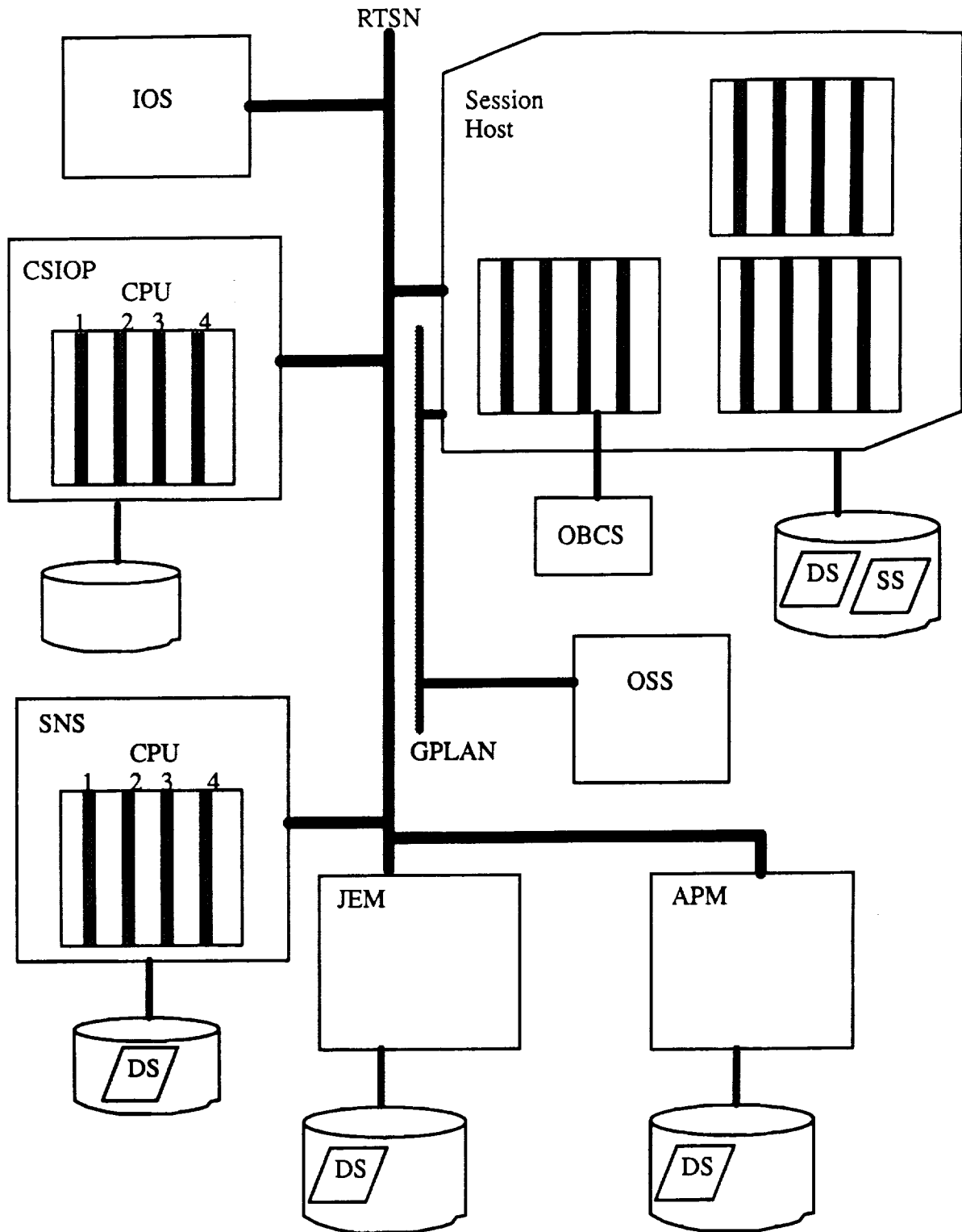
Figure 4.6-2. Physical Layout of Training Session
