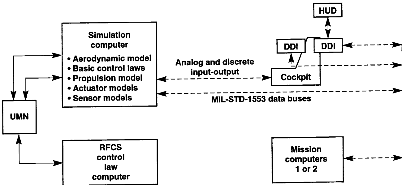
Fig. 6 The High Alpha Research Vehicle all-software simulation.
