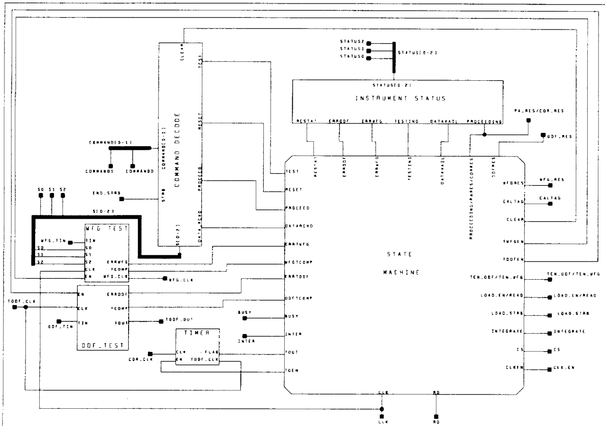
Figure 6: DDS Controller Prototype Schematic Diagram
