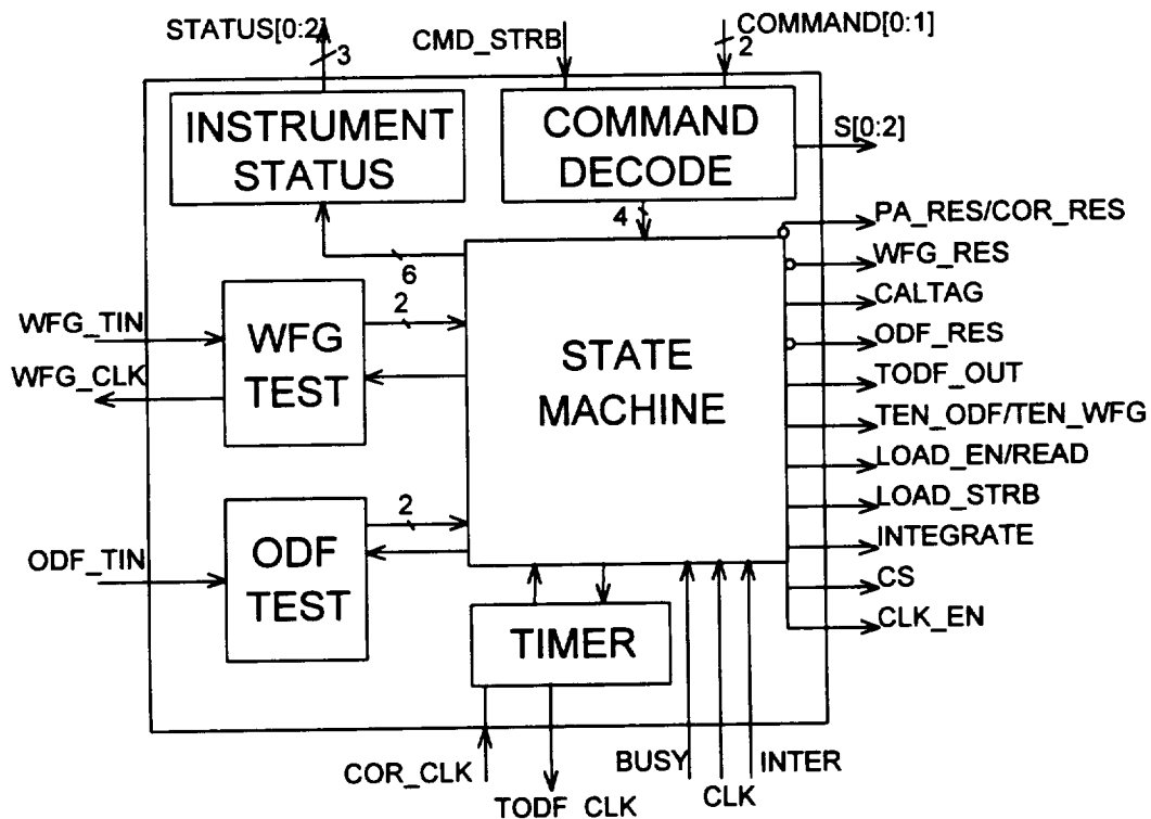
Figure 4: DDS Controller Functional Block Diagram
