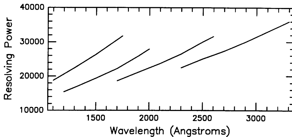
Figure 8-2. Spectrum resolving power as a function of wavelength for the GHR medium-resolution (holographic) gratings. From left to right the curves are for G140M, G160M, G200M, and G270M, respectively.
