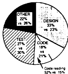
IMPACT ON EFFORT DISTRIBUTION Cleanroom vs. baseline
