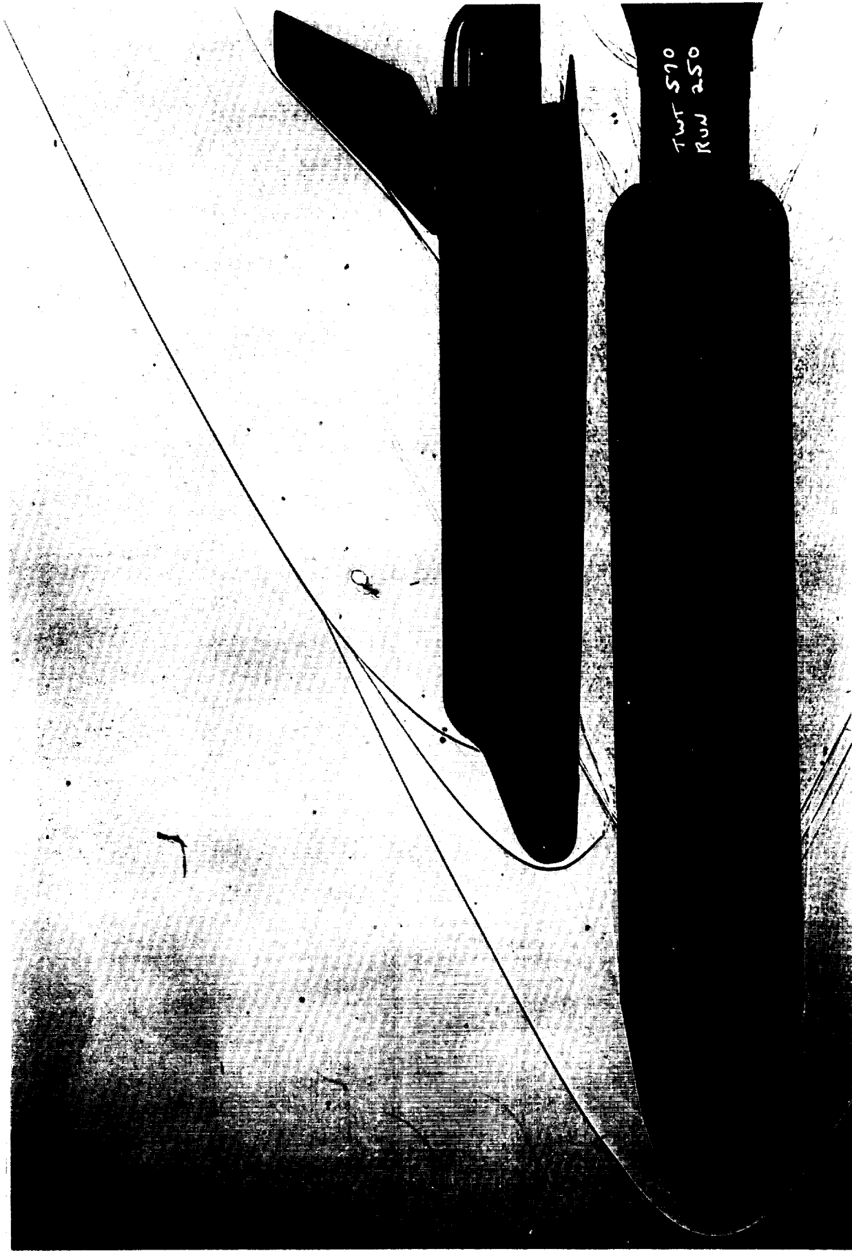
Figure C-9. SSLV with nose T12, Mach 3.48, \alpha = 0 , \beta = 0 , roll = 0.
