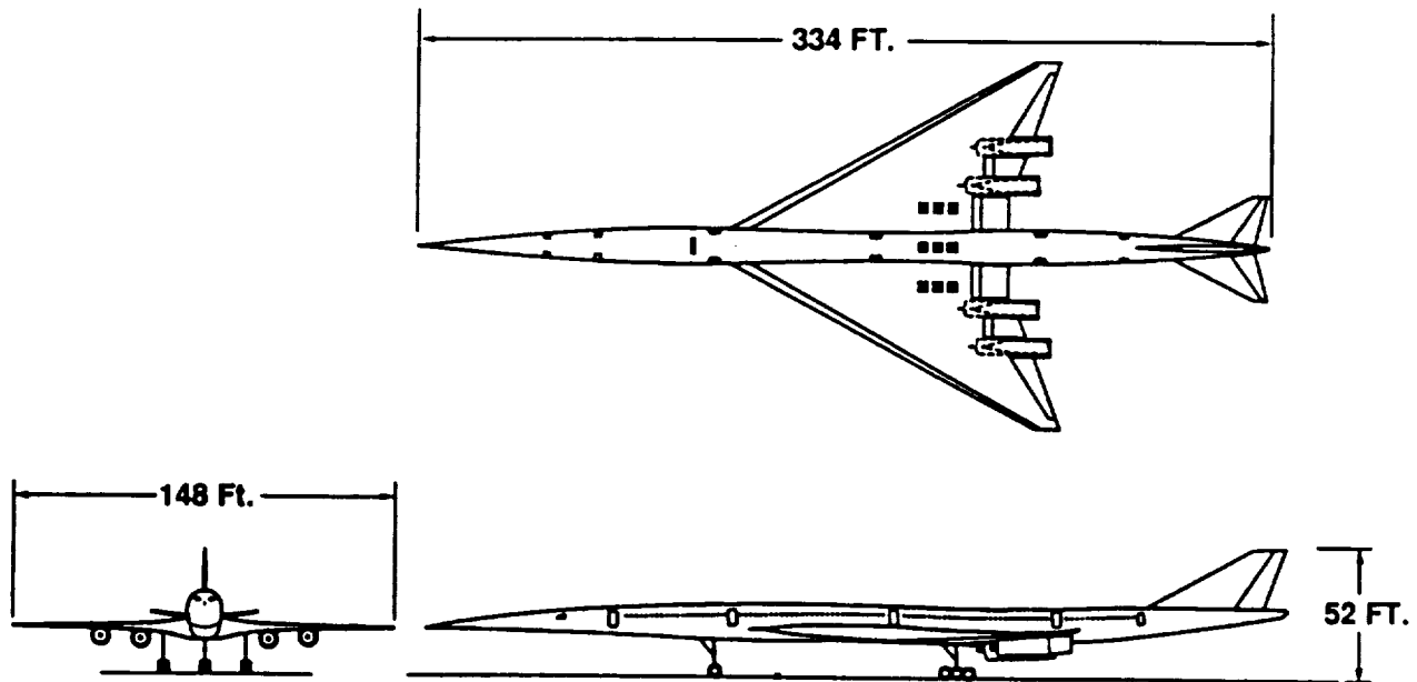
Figure 12. Configuration for a Mach 1.6 HSCT from design optimization studies at McDonnell Douglas.
