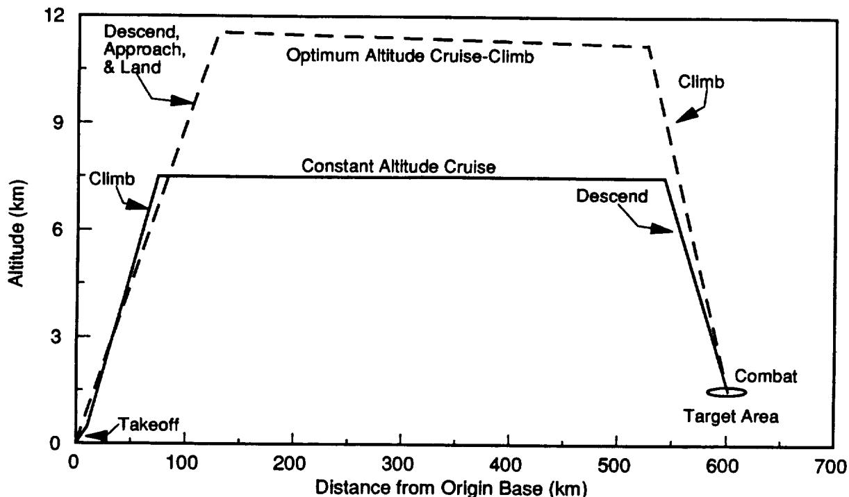
Figure 7. Example mission profile for a fighter/attack generic aircraft. All military air traffic component missions begin and end at the same location.
