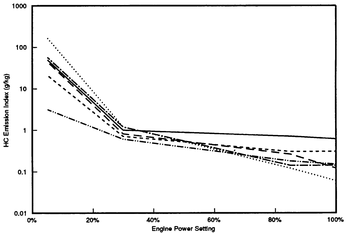
Figure 2. CO (upper panel) and HC (lower panel) emission indices decrease as engine power setting (percent of takeoff rated thrust) increases. Engine rated thrust is expressed in kilonewtons.
