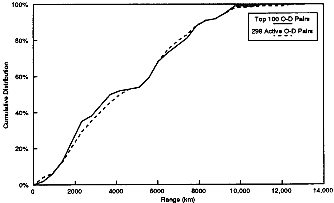
Figure 9. Cumulative distribution of ranges between selected origin-destination city pairs that have a positive 1990 charter air traffic level. Top 100 city pairs formed the basis for the charter network.
