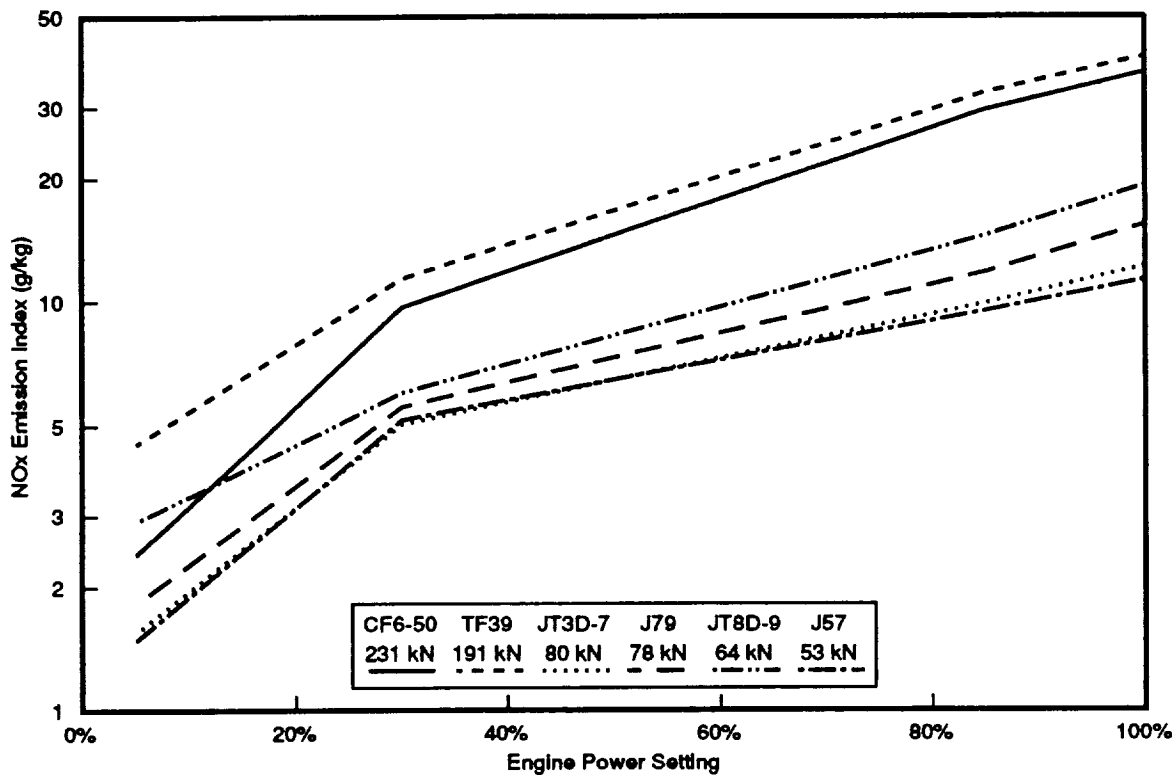
Figure 3. NO x emission indices increase as engine power setting (percent of rated thrust) increases. Engine rated thrust is expressed in kilonewtons.
